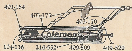
Camp Stove Nos. 2C and 9C
