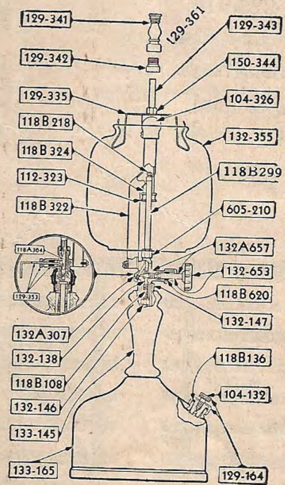
Instant Lighting Lamp No. 133
