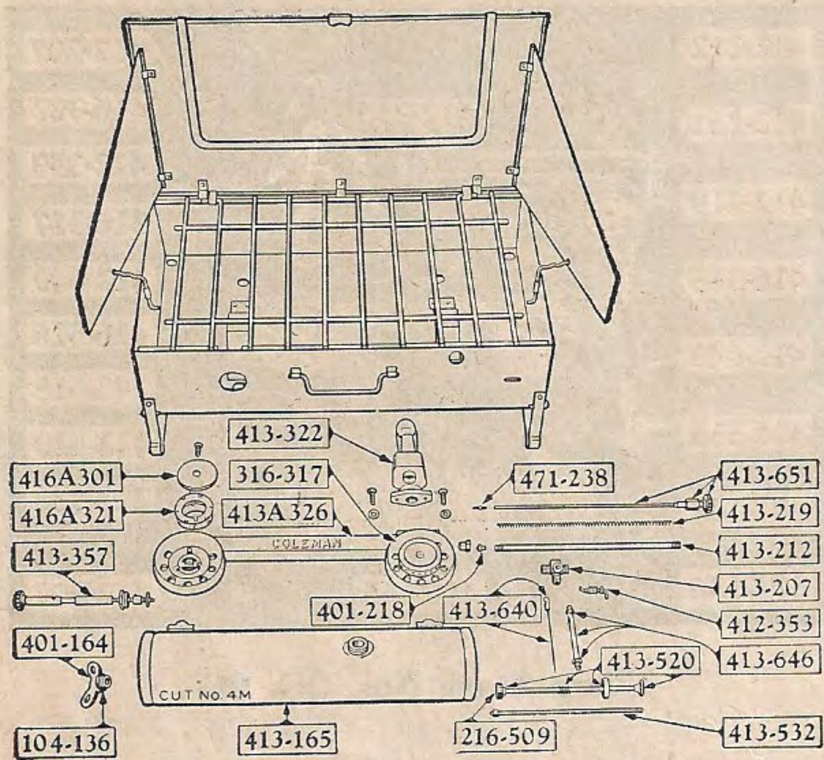
Camp Stove No. 3H
