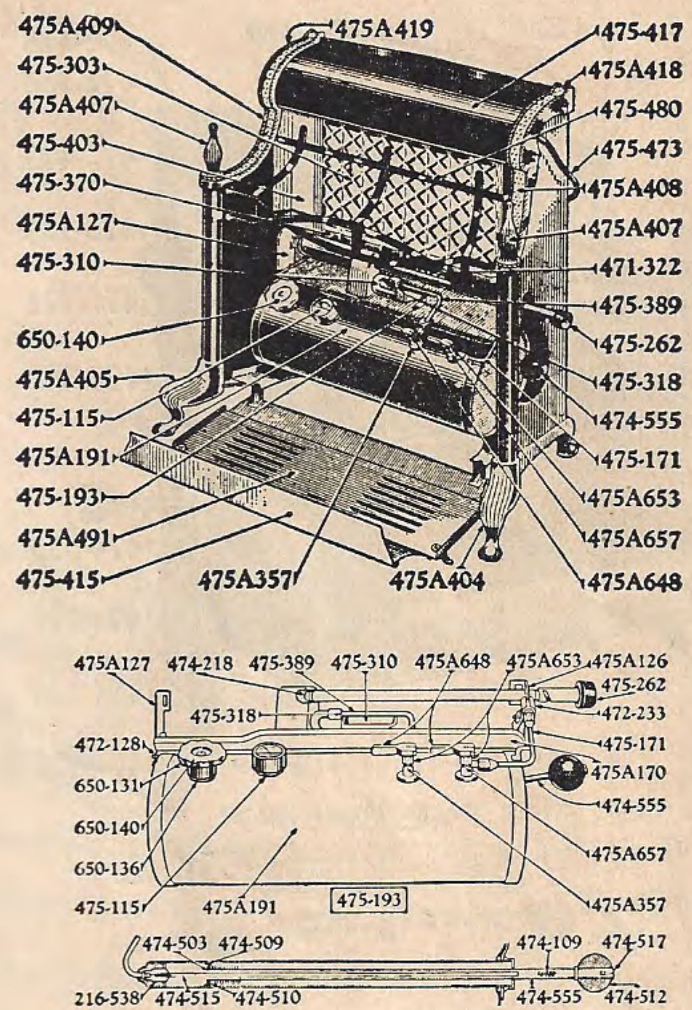
Radiant Heater No. 5A
