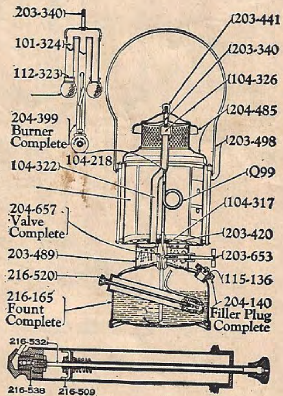
Match-Generating Quick-Lite Lantern Nos. L427, L227 (old style)
