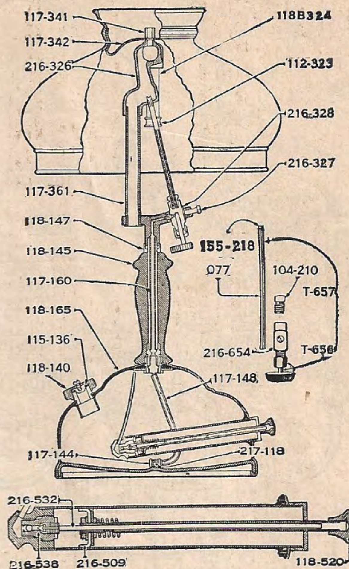
Instant-Lite Lamp Nos. 118 and 119
