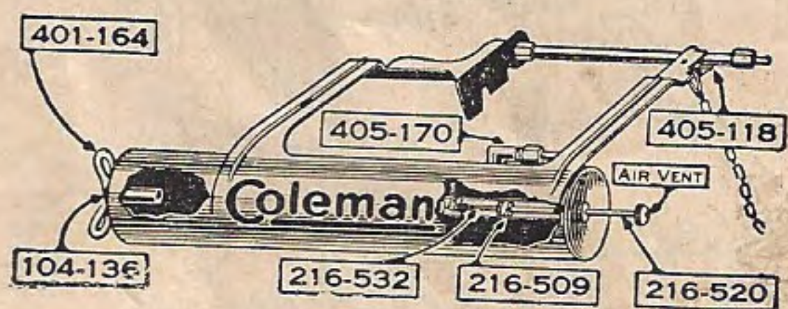
Camp Stove Nos. 2D and 9D
