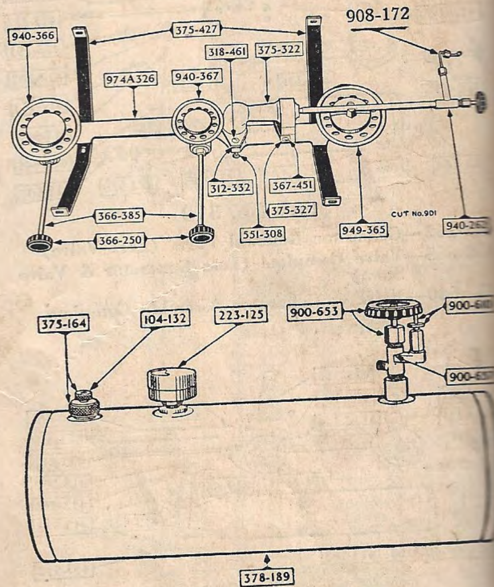
Cabin Stove No. 378, 379
