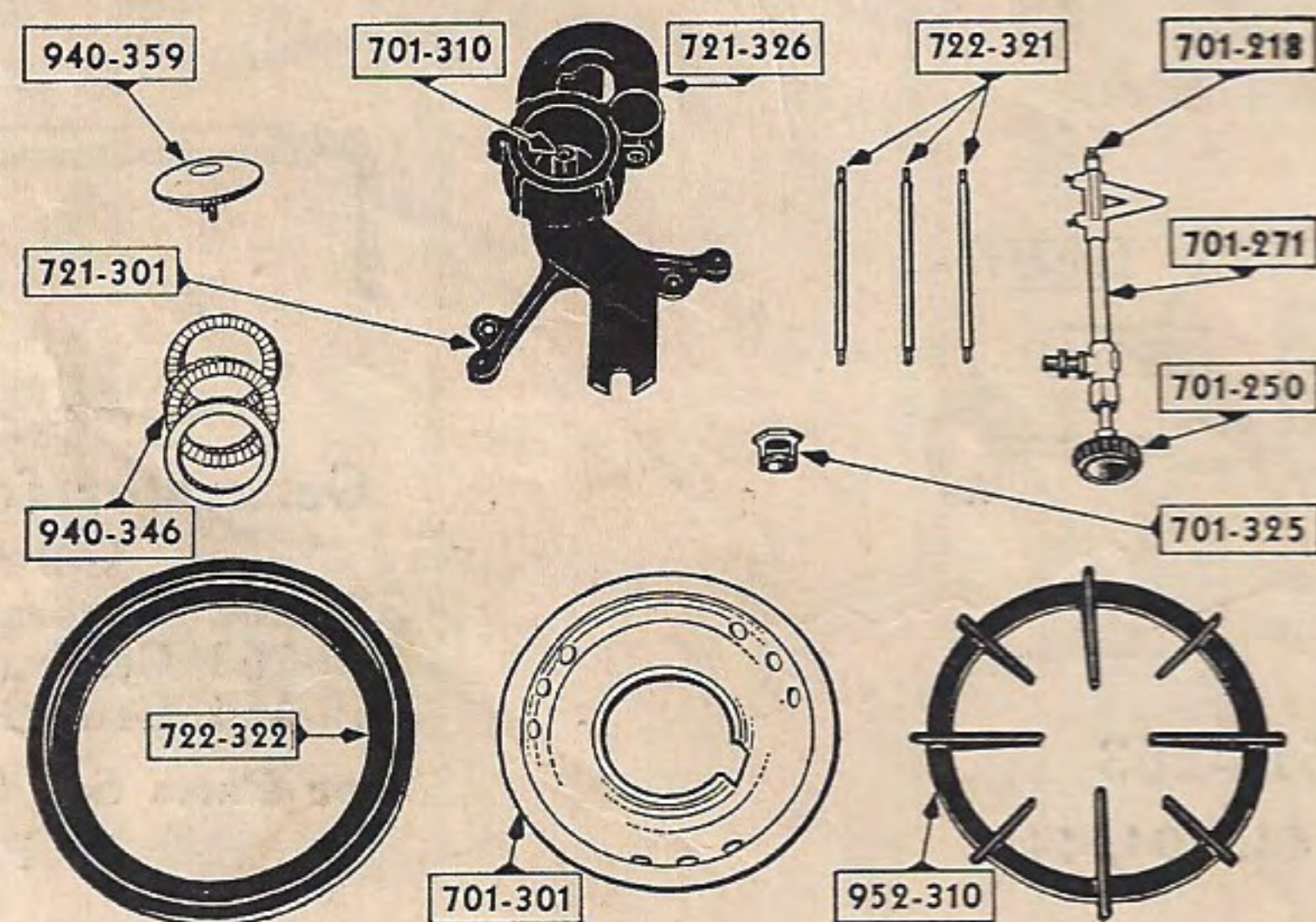
Bottle Gas Burner Nos. 721 and 722
