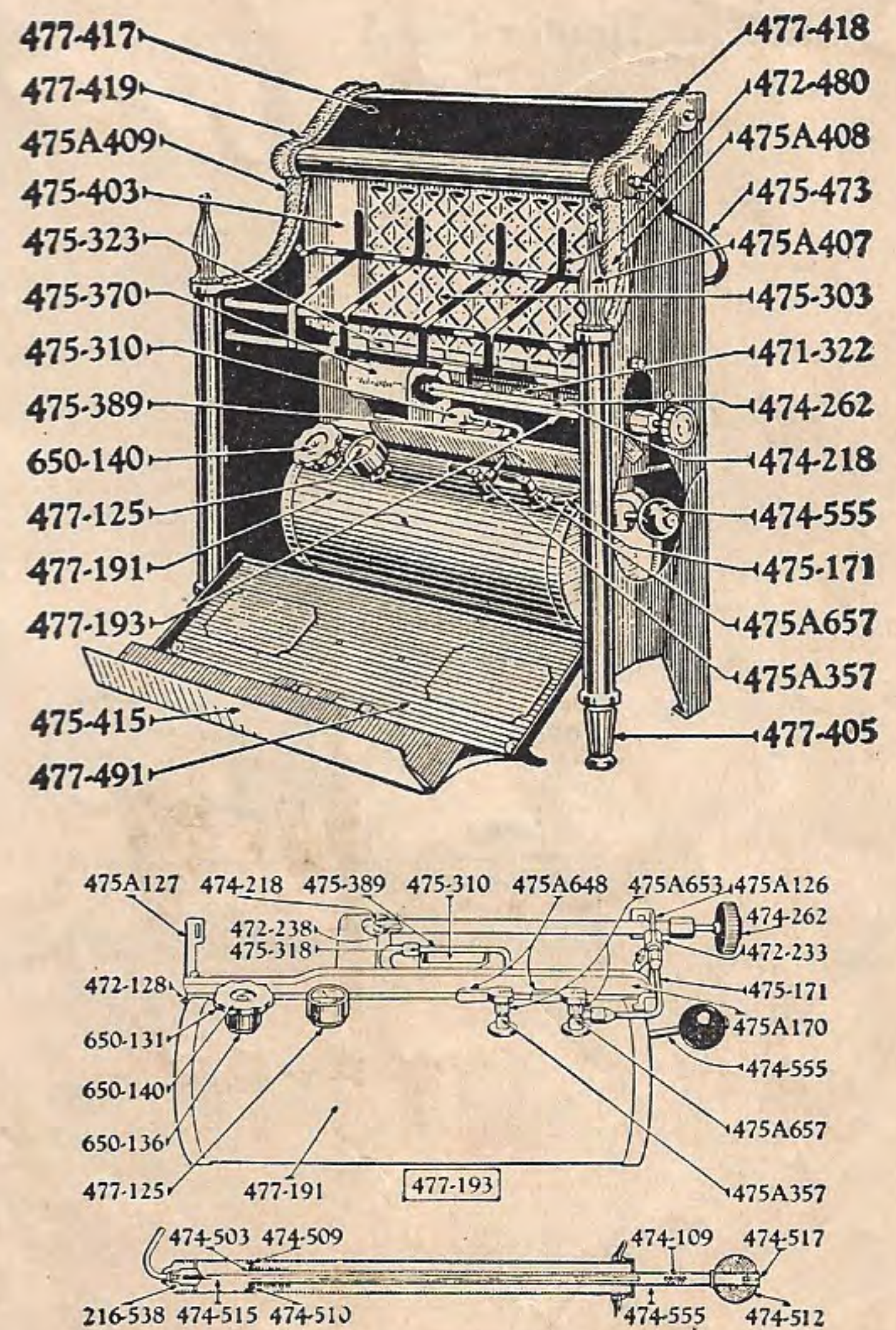
Radiant Heater No. 7
