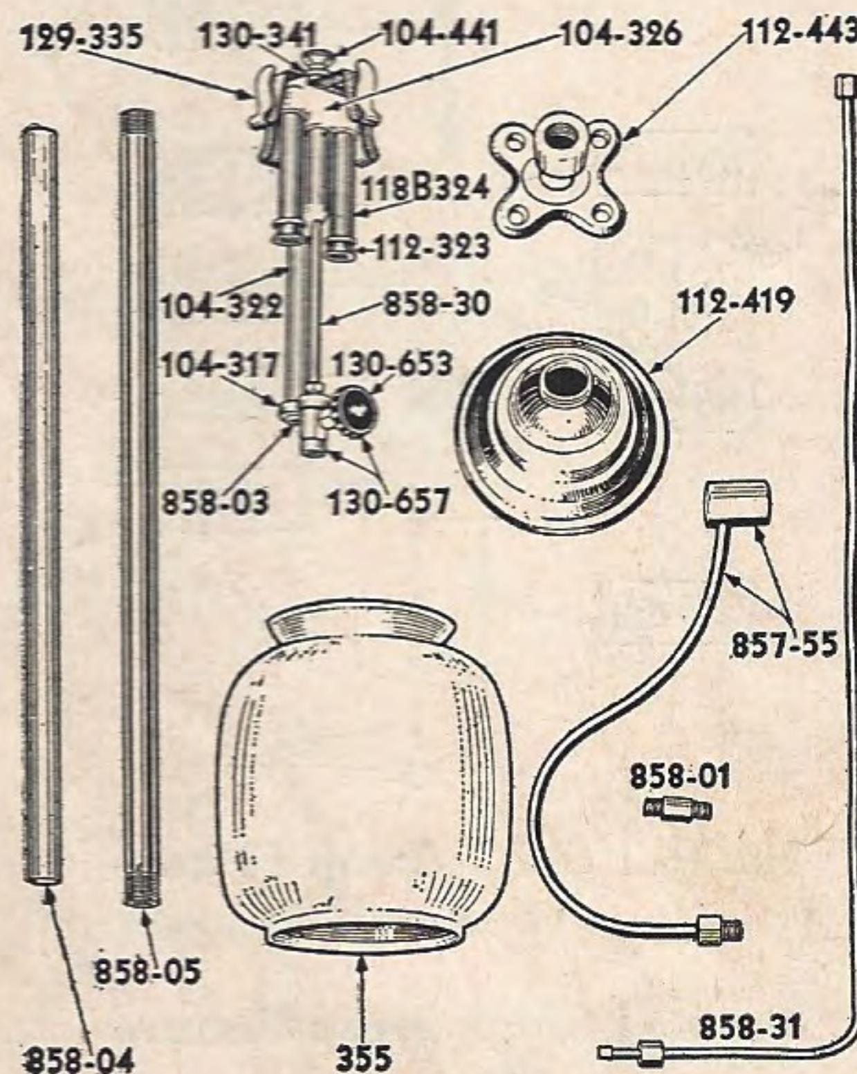
No. 857 Single-Drop Fixture
