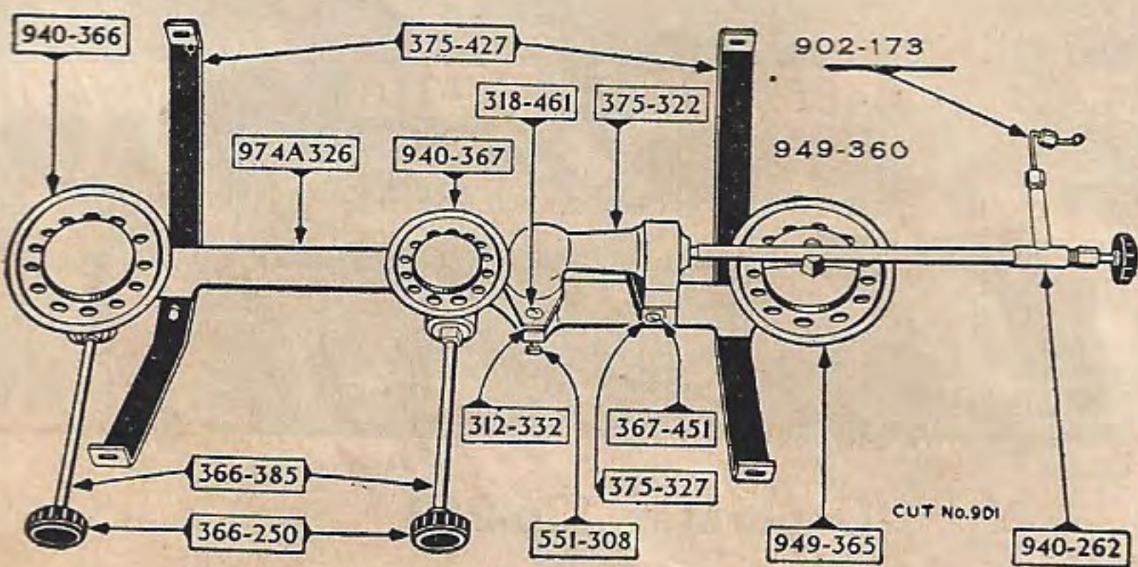
Cabin Stove Nos. 378A and 379A
