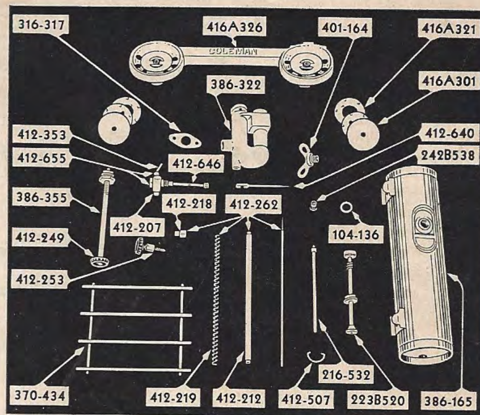
Stove No. 386
