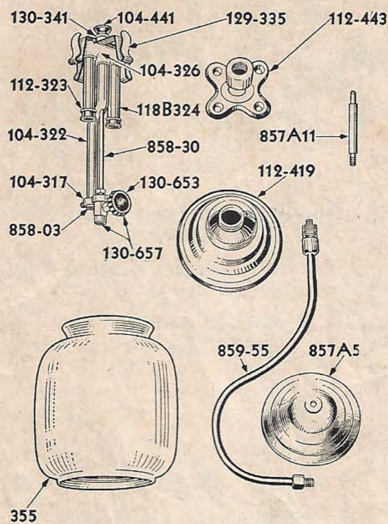
No. 859 Bracket Fixture
