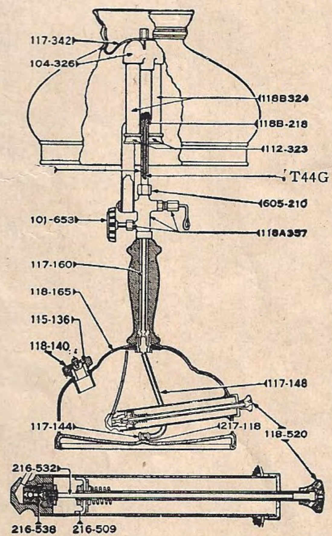
Instant-Lite Lamp Nos. 118A, 119A
