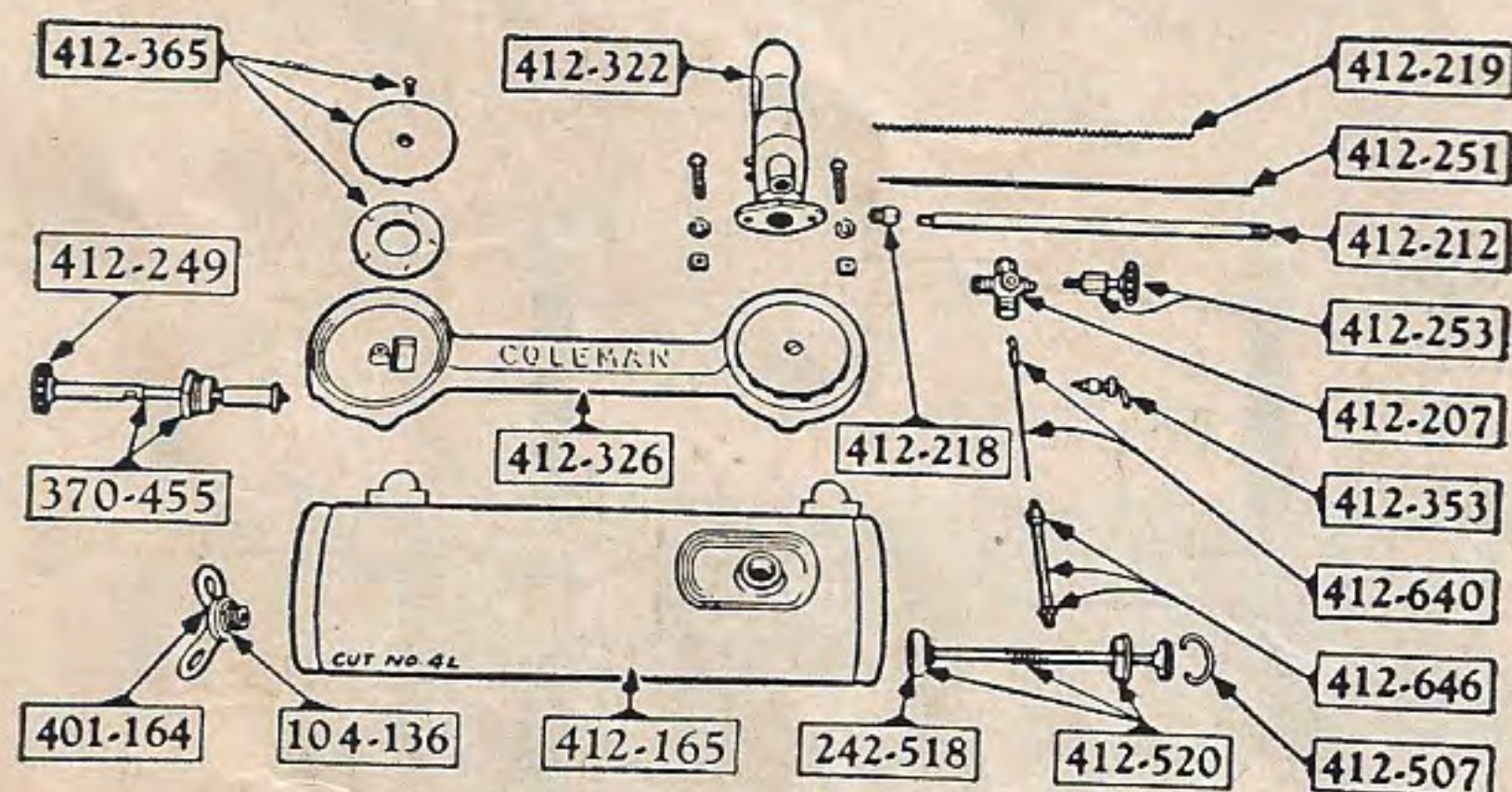
Stove No. 370
