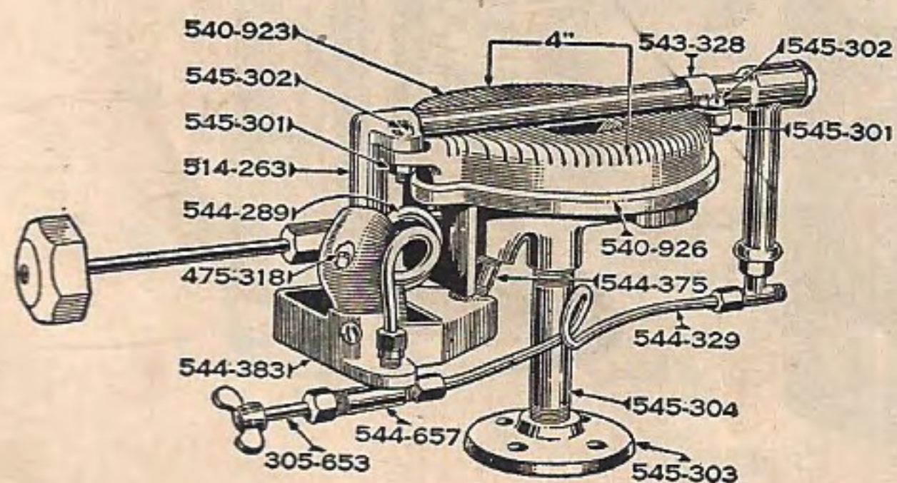
Burner No. 404 (Uses 4-inch Burner Cap)
