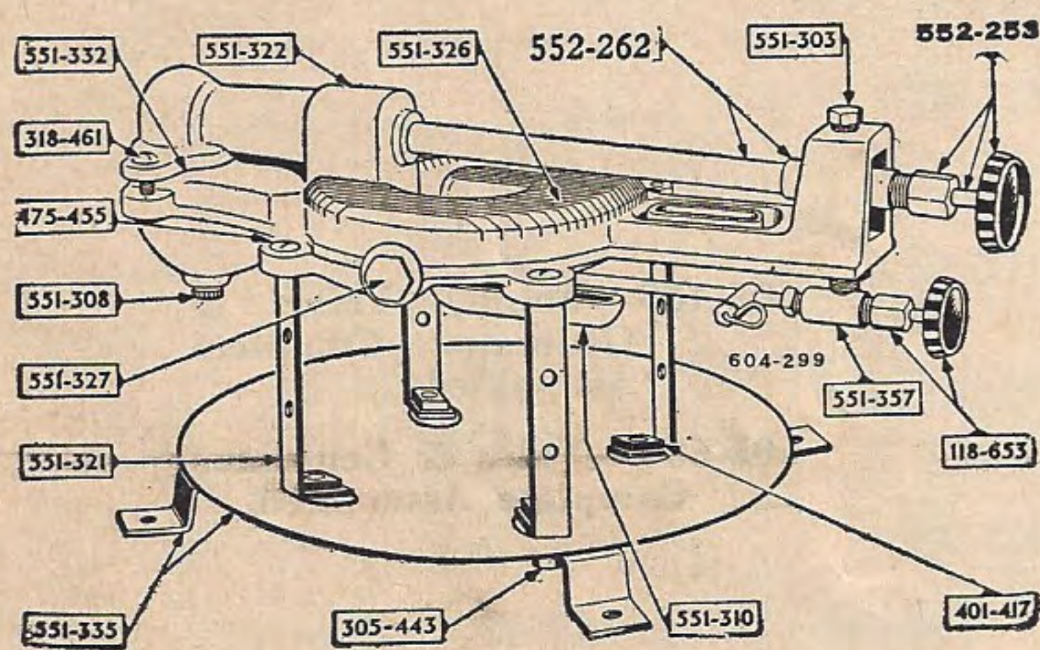
Burner No. 501
