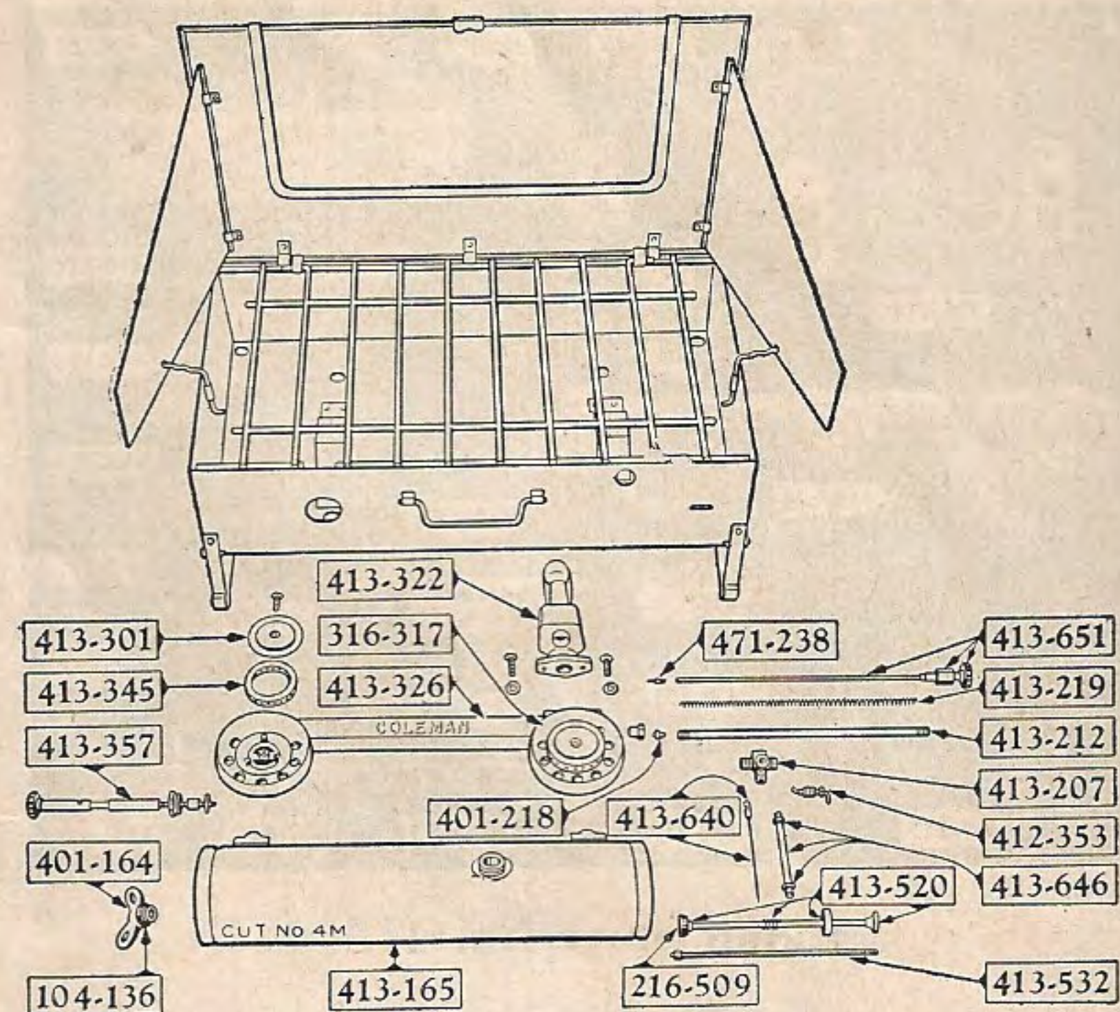
Camp Stove No. 3F
