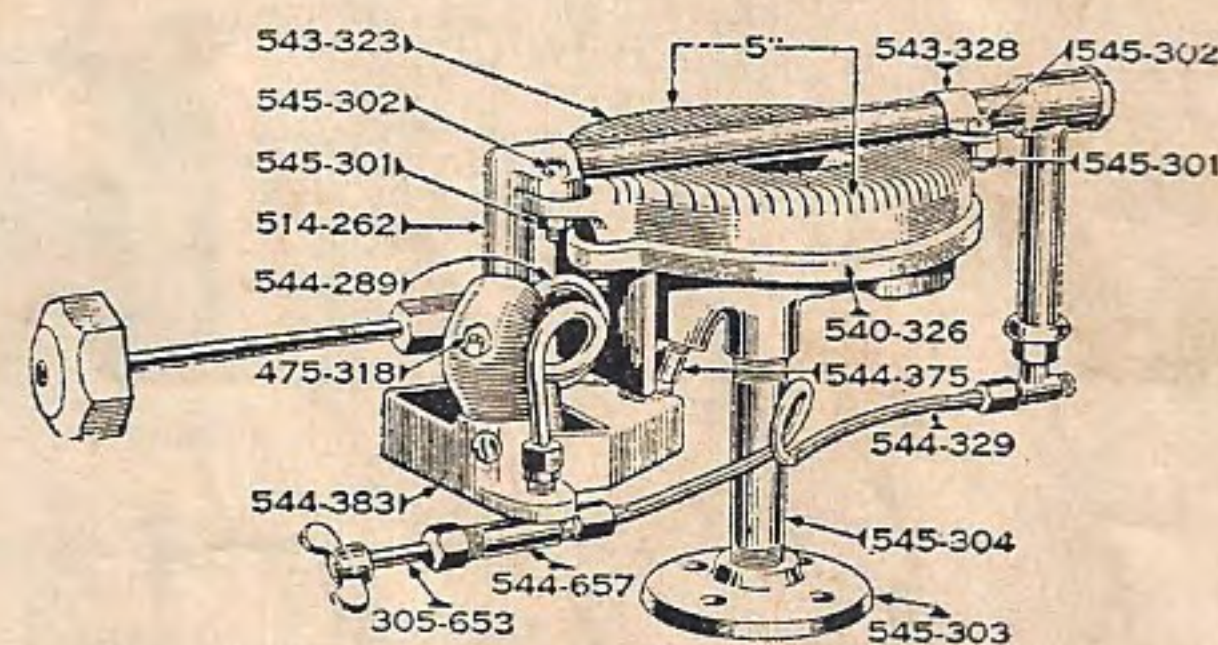
Burner No. 505 (Uses 5-inch Burner Cap)
