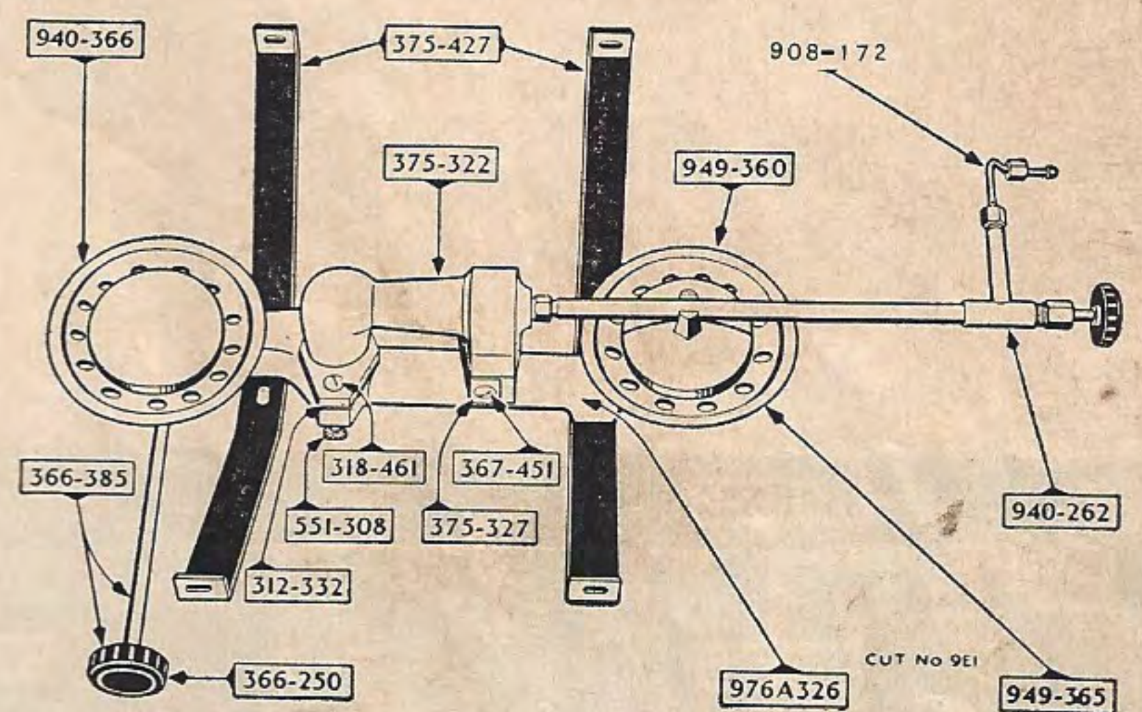
Cabin Stove No. 377
