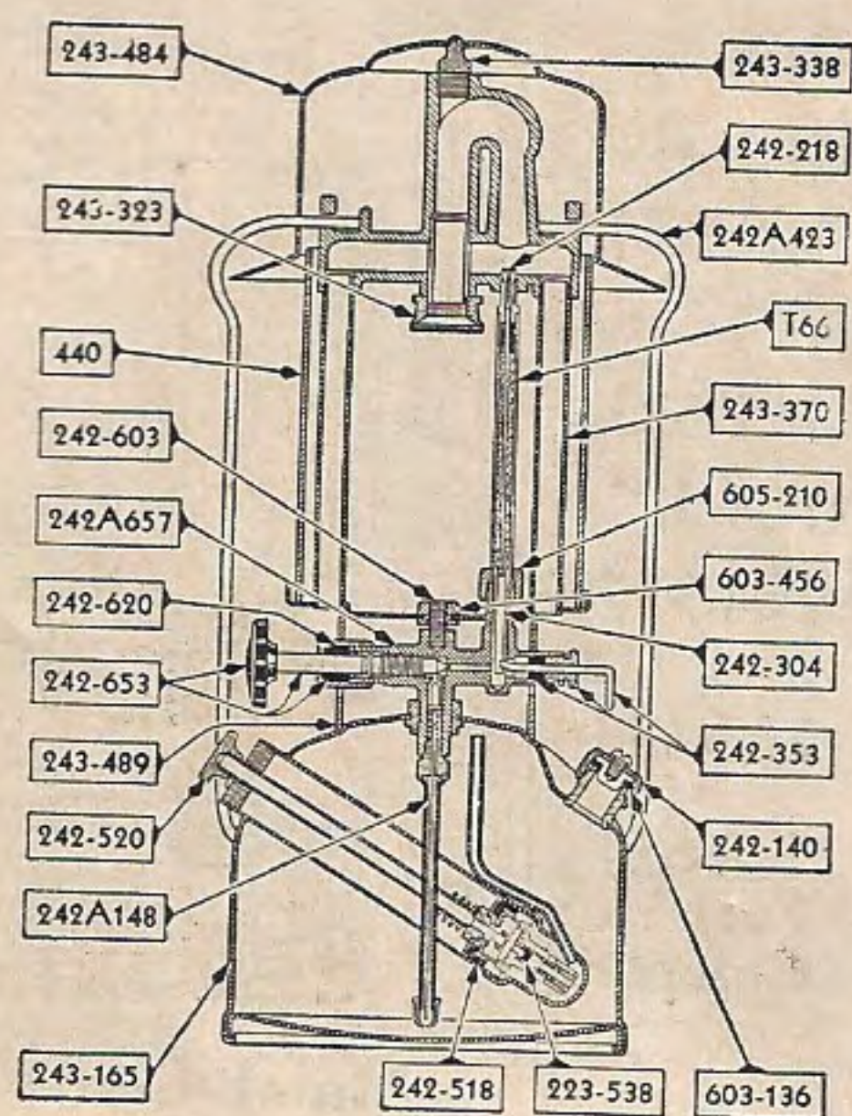
Instant-Lite Lantern No. 243
