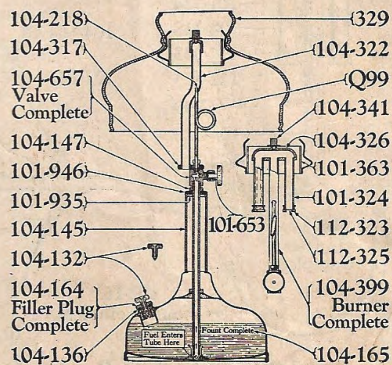
"C" Model Quick-Lite Lamp
