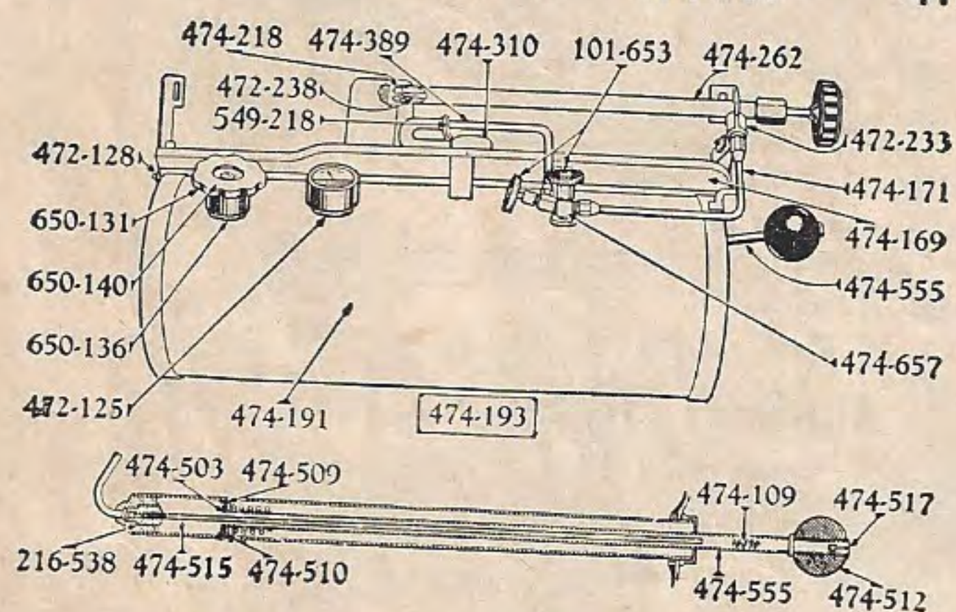
Radiant Heater No. 4
