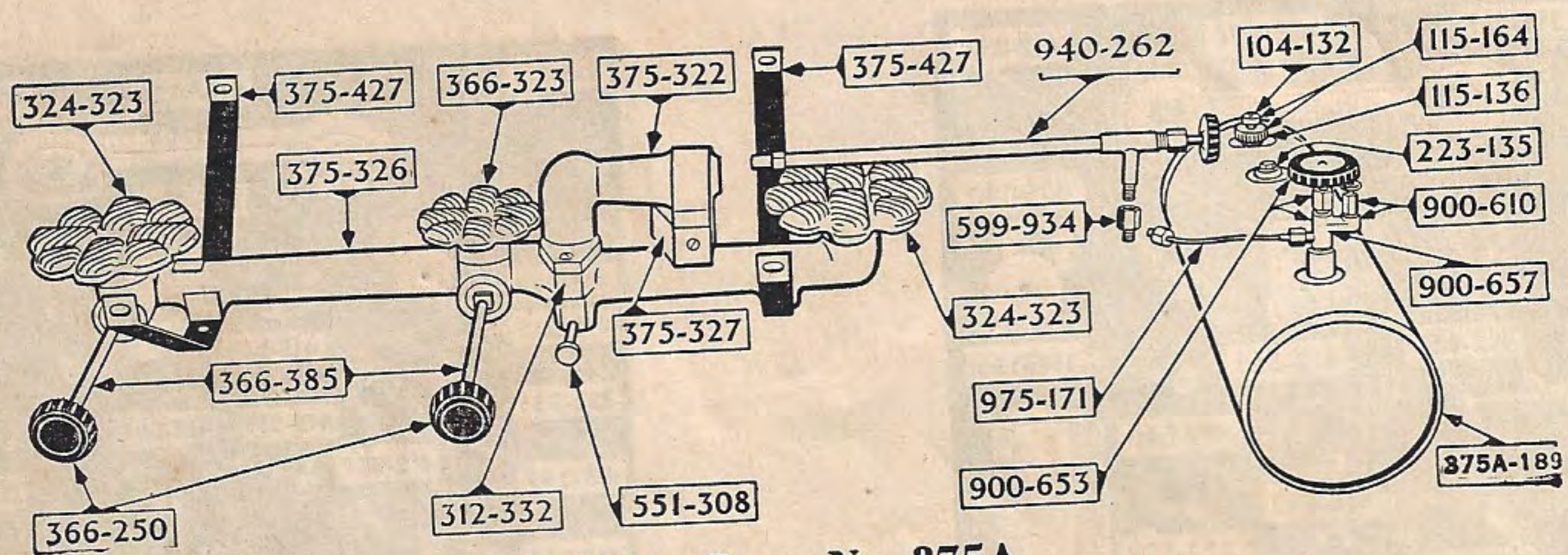
Cabin Stove No. 375A
