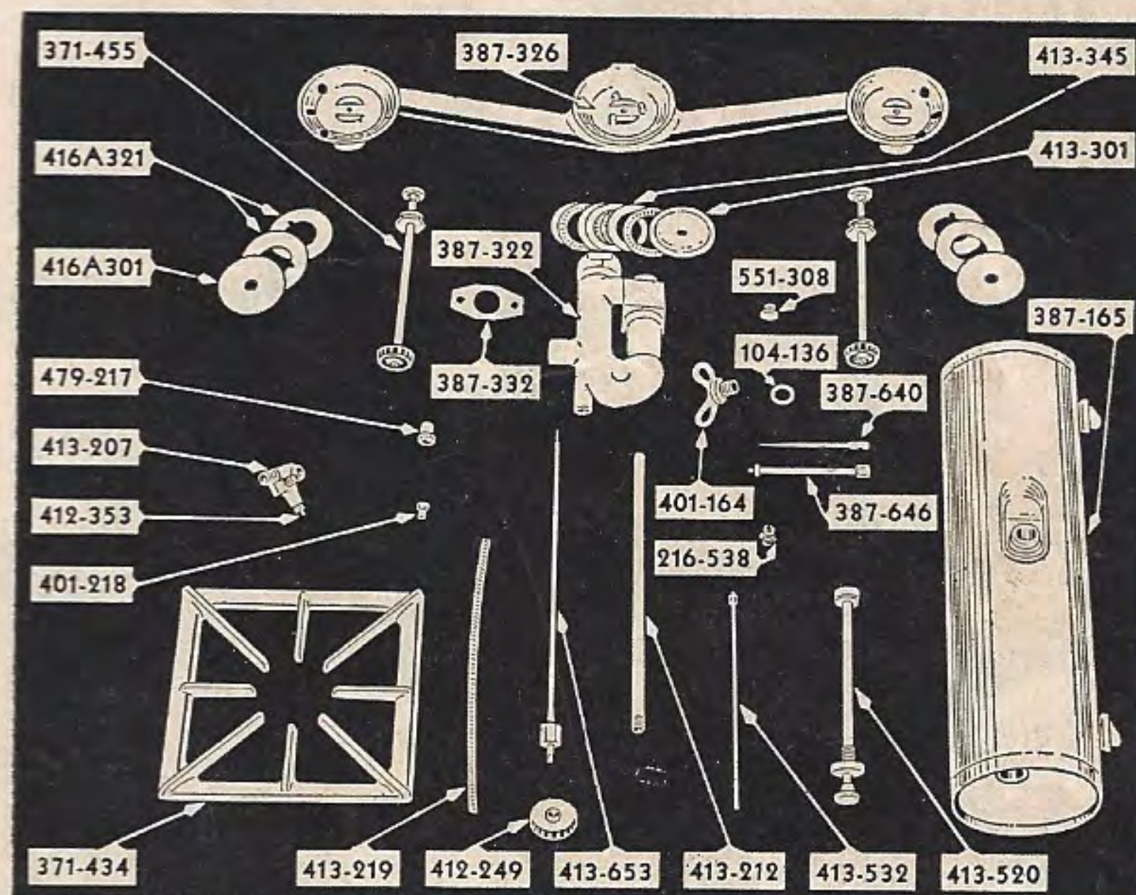
Stove No. 387
