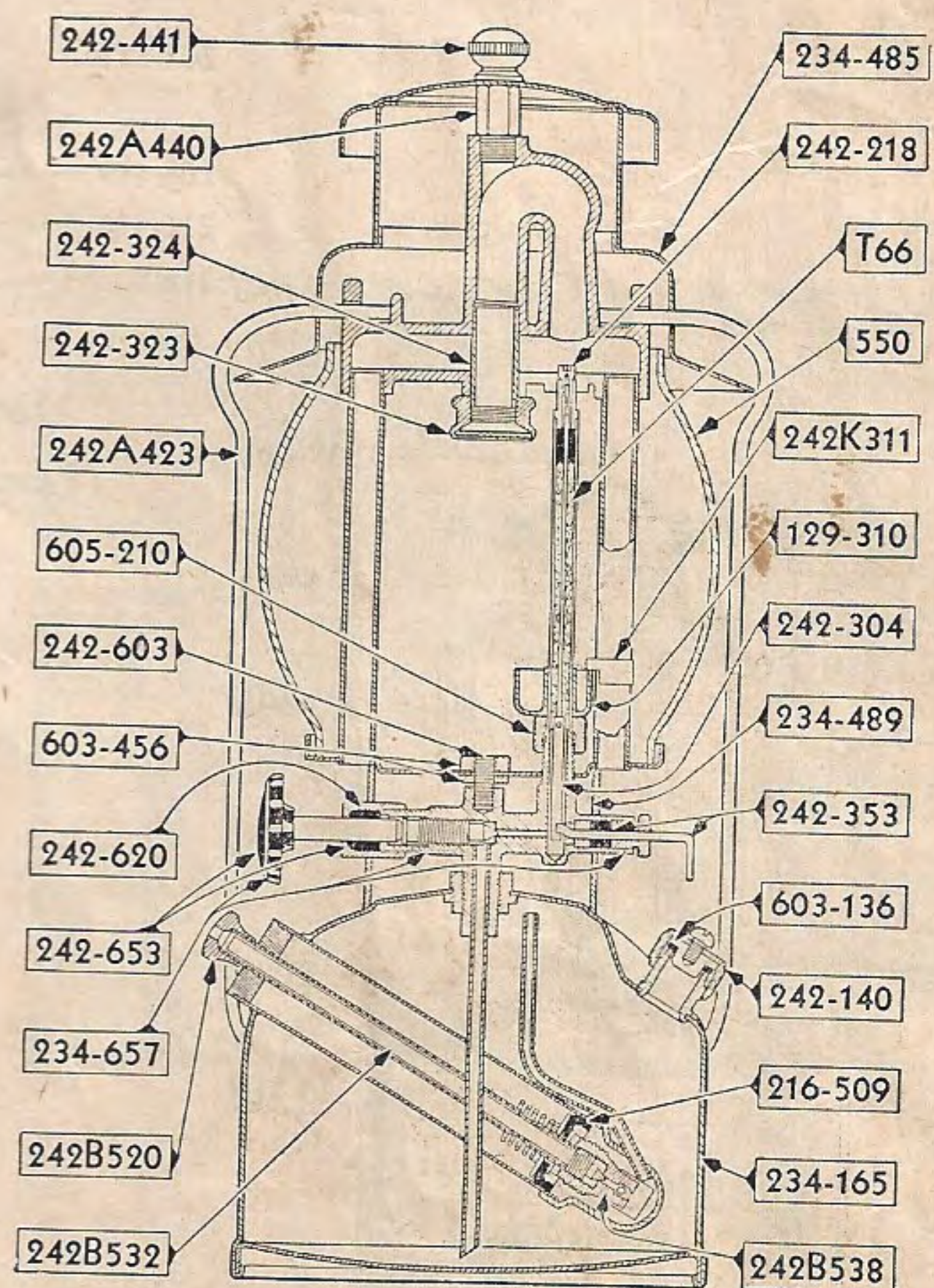
Kerosene Single Mantle Lantern No. 234 Alcohol Generating
