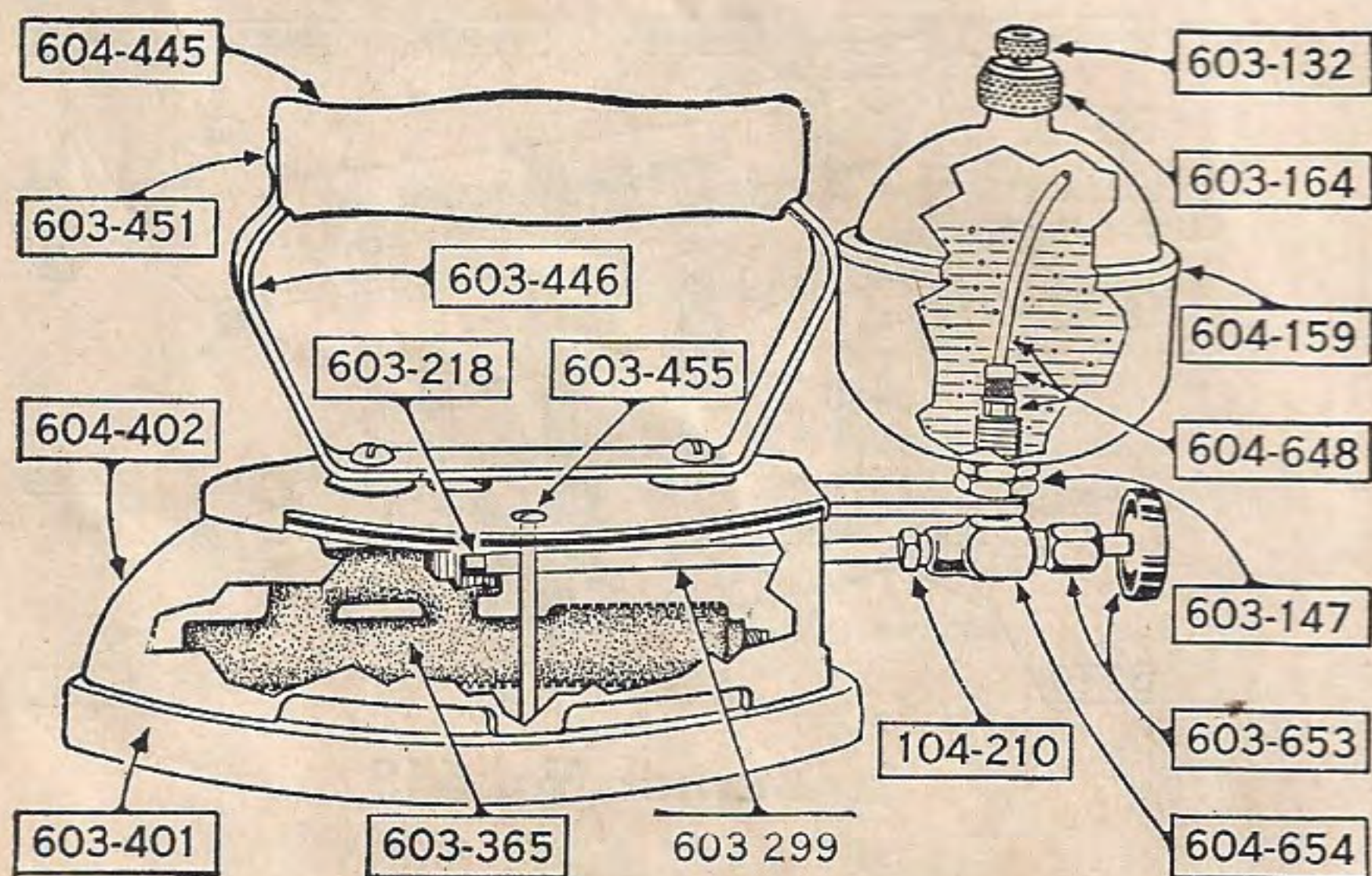
Iron No. 4 (Instant-Lighting)
