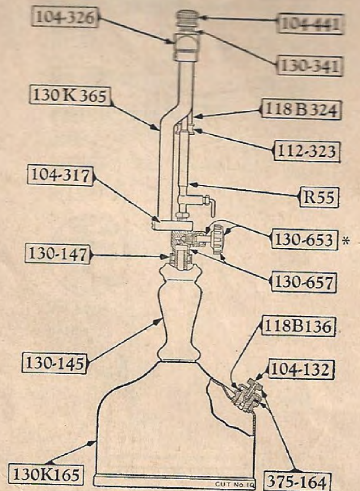
Kerosene Mantle Lamp Torch-Generating Lamp No. 130K
