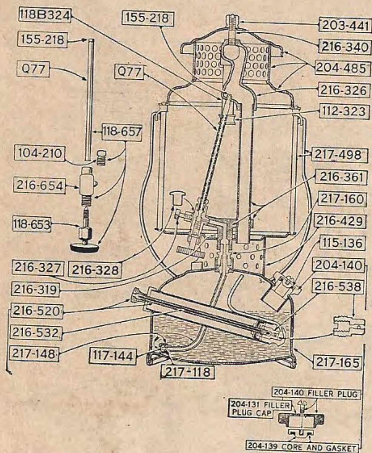
Instant-Lite Lantern Nos. 220, 228
