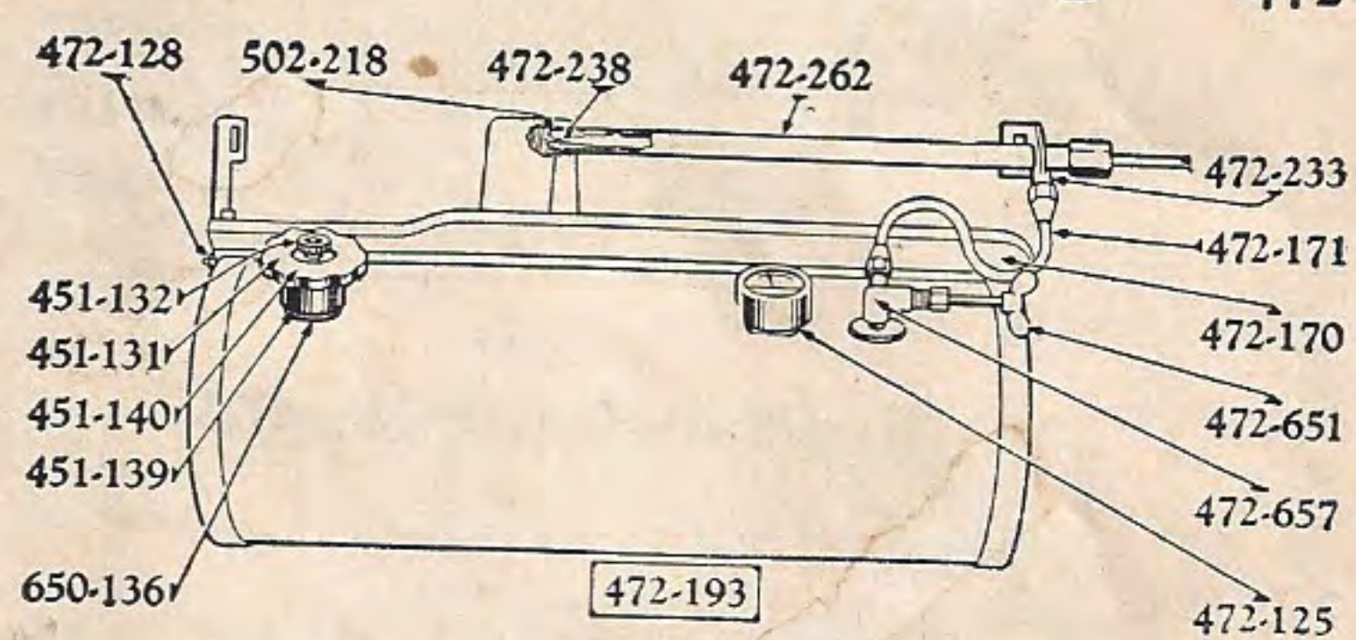
Radiant Heater No. 2
