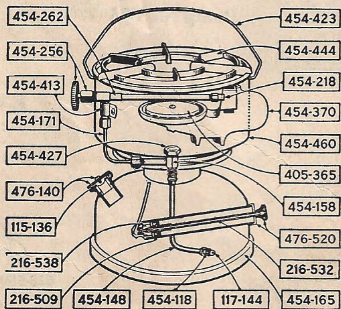
Utility Burner No. 454
