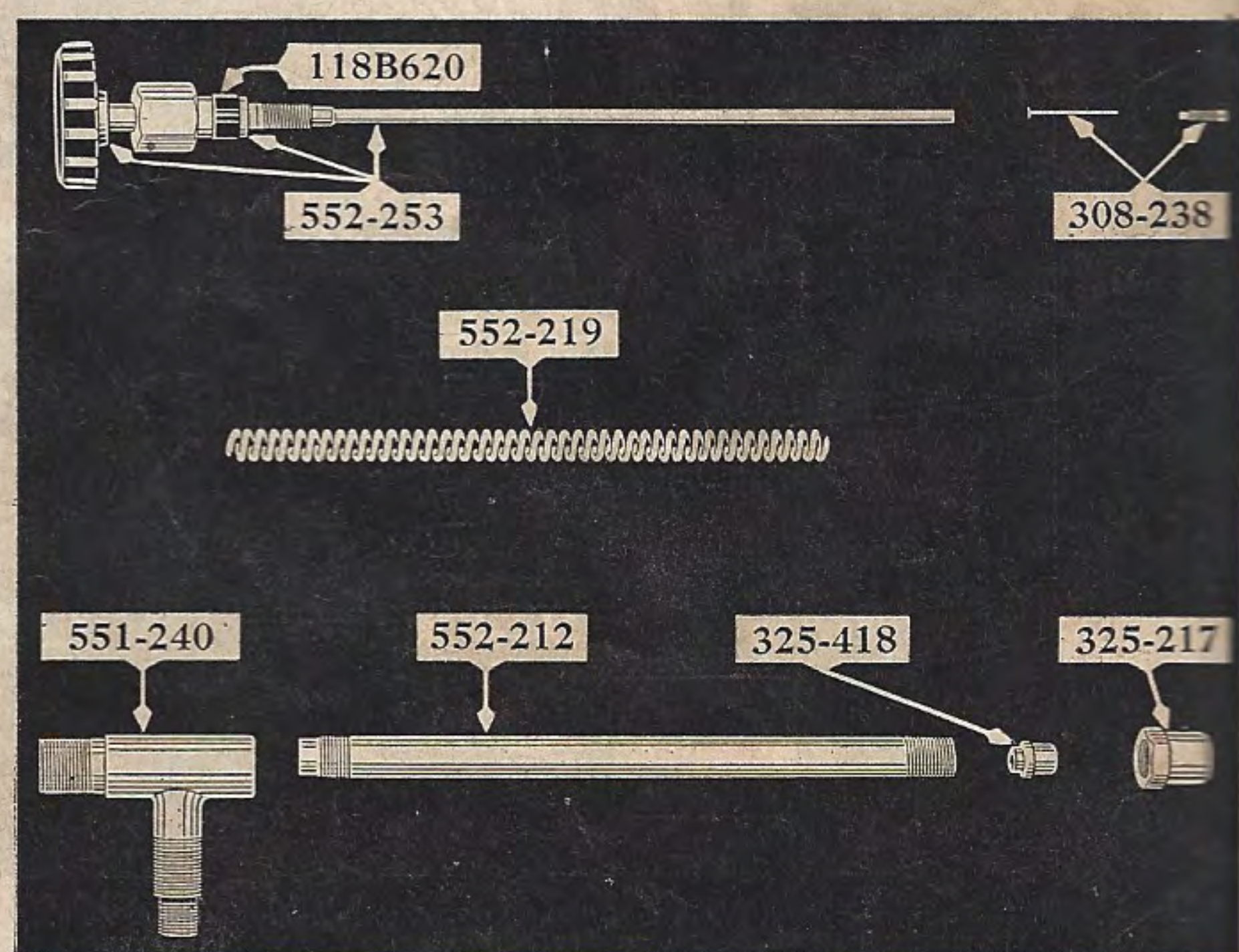
Generator No. 552-262
