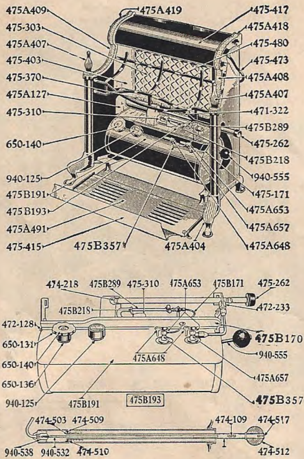
Radiant Heater No. 5B
