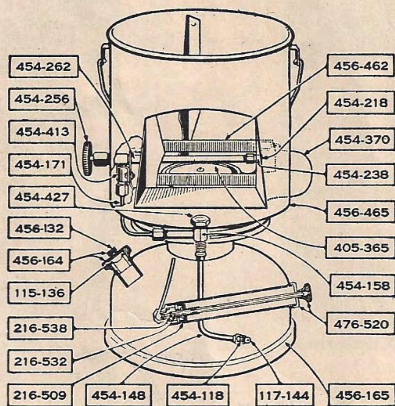
Soldering Furnace No. 456
