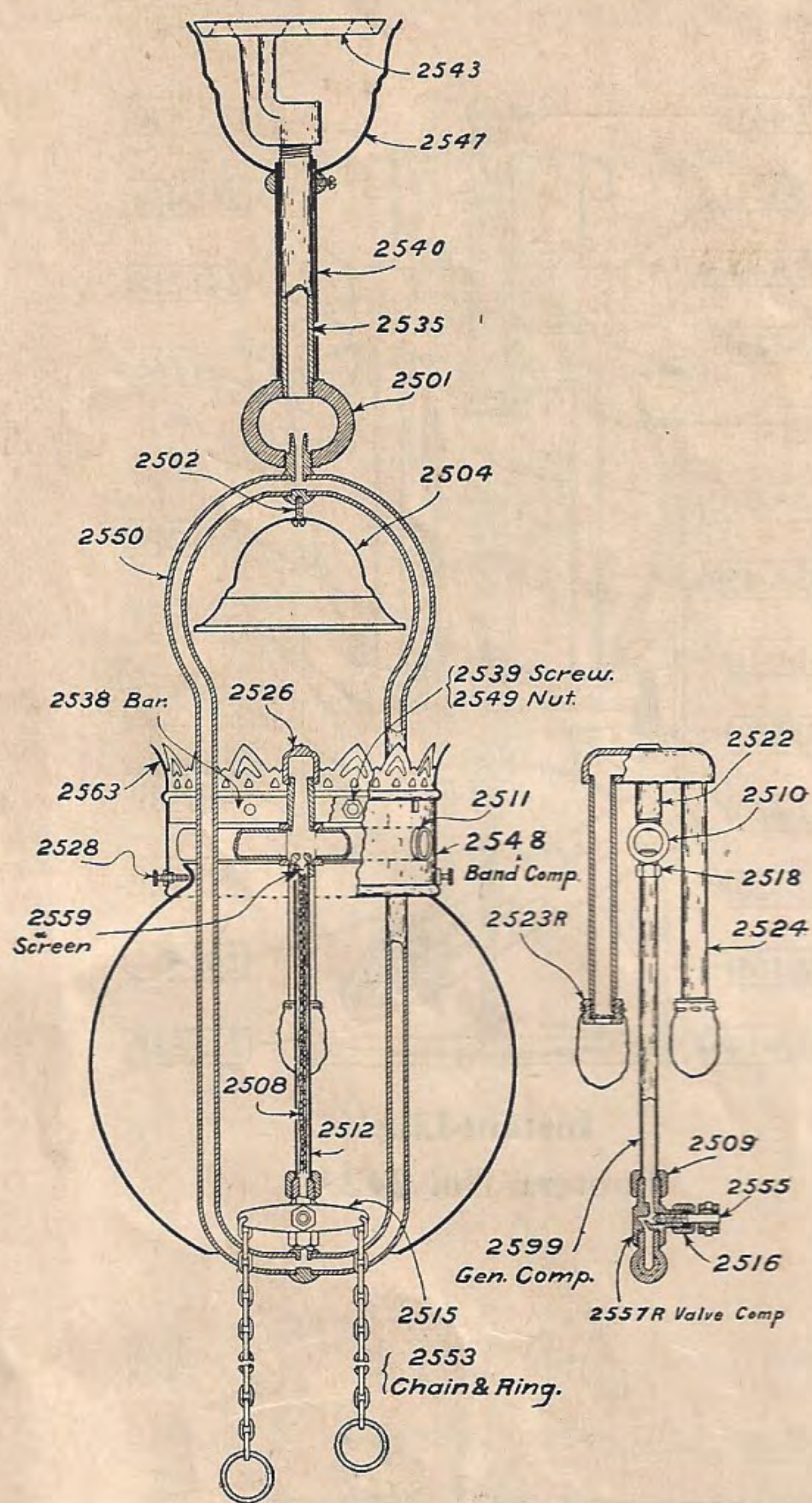
Ceiling Fixture System Lamp No. 25
