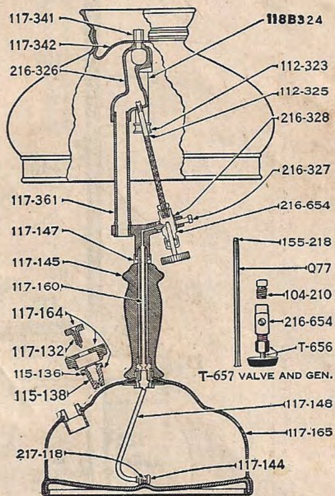
Instant-Lite Lamp No. 117
