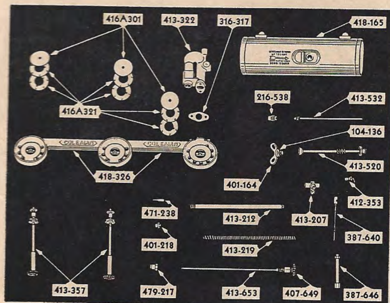
Camp Stove No. 418
