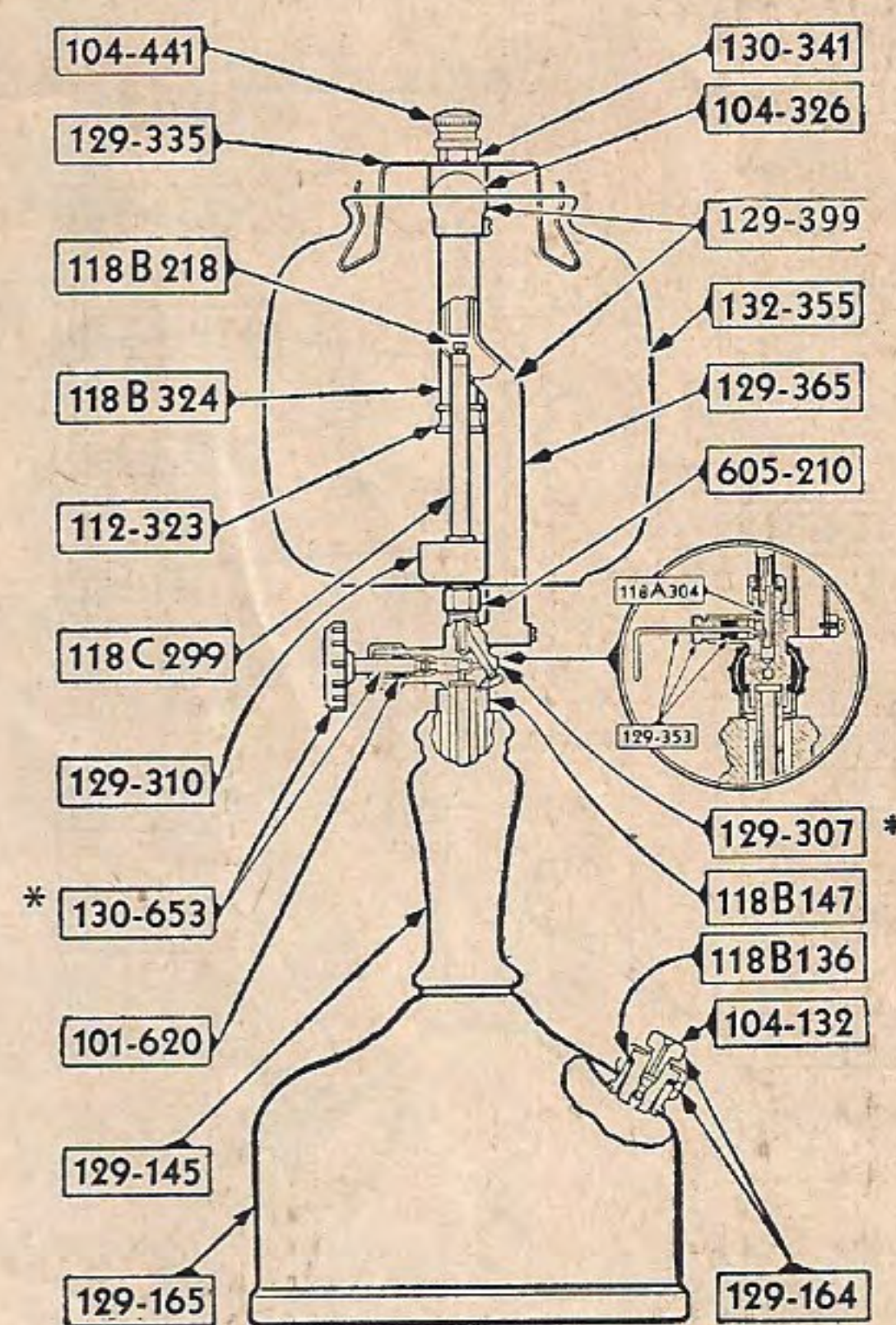
Kerosene Mantle Lamp Alcohol Generating Lamp No. 129G
