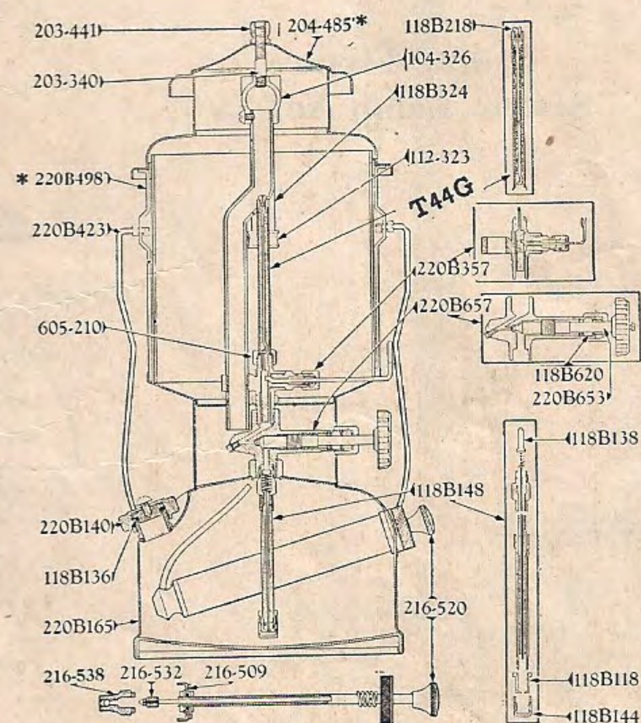
Instant-Lite Lantern Nos. 220B, 228B
