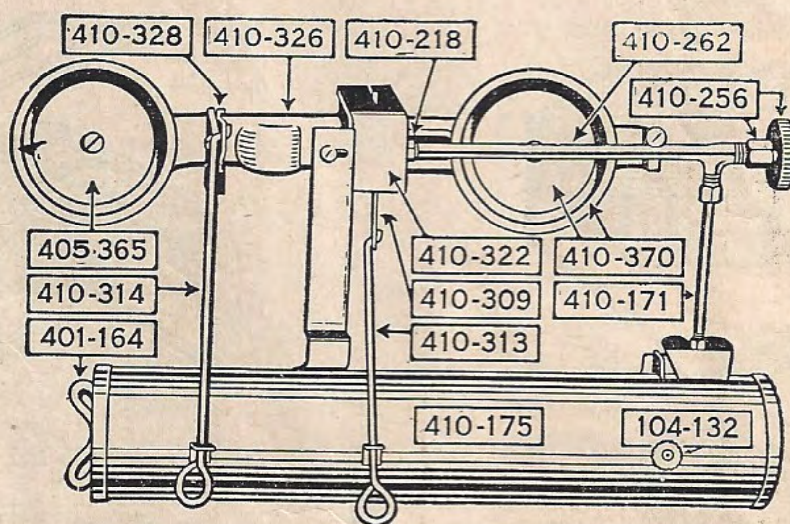
Gypsy Camp Stove No. 10
