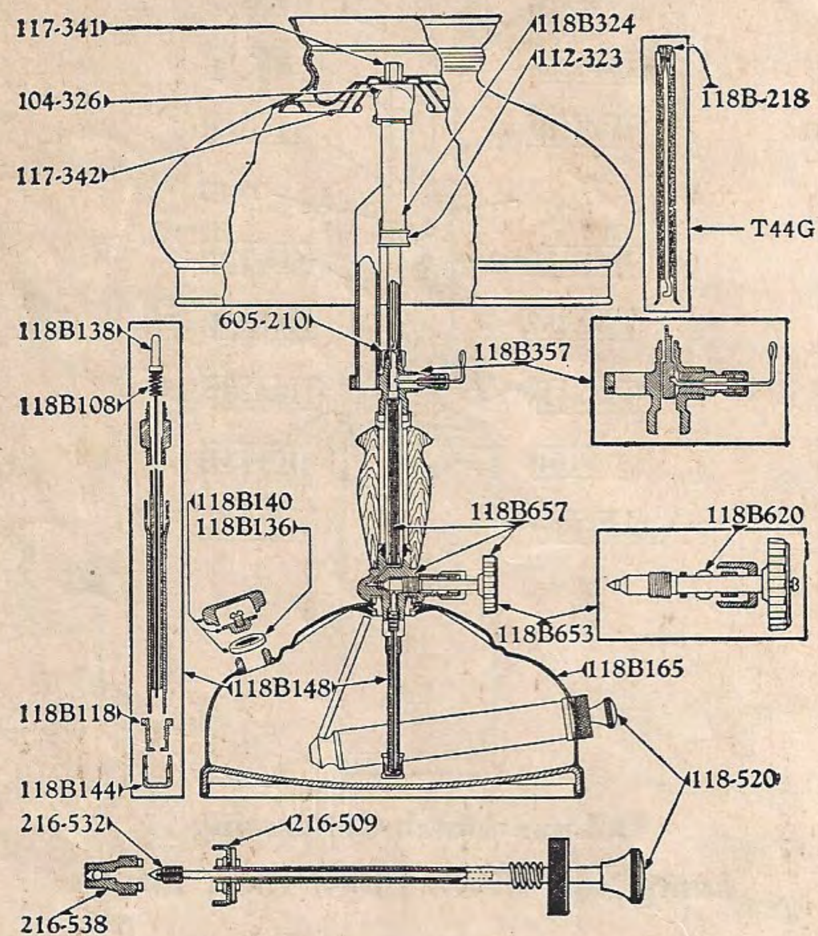
Instant-Lite Lamp No. 118B
