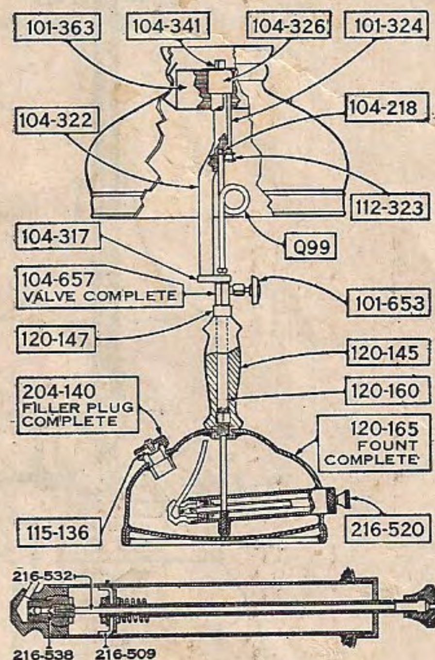
Quick-Lite Lamp No. C331
