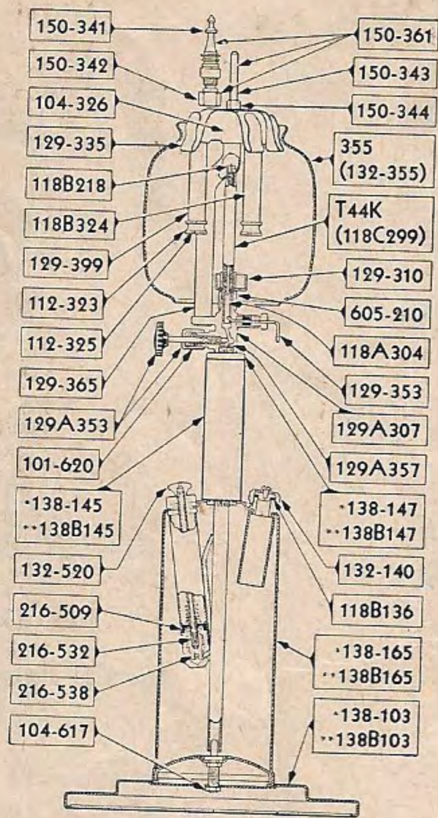
Kerosene Lamps Nos. 138A and 138B
