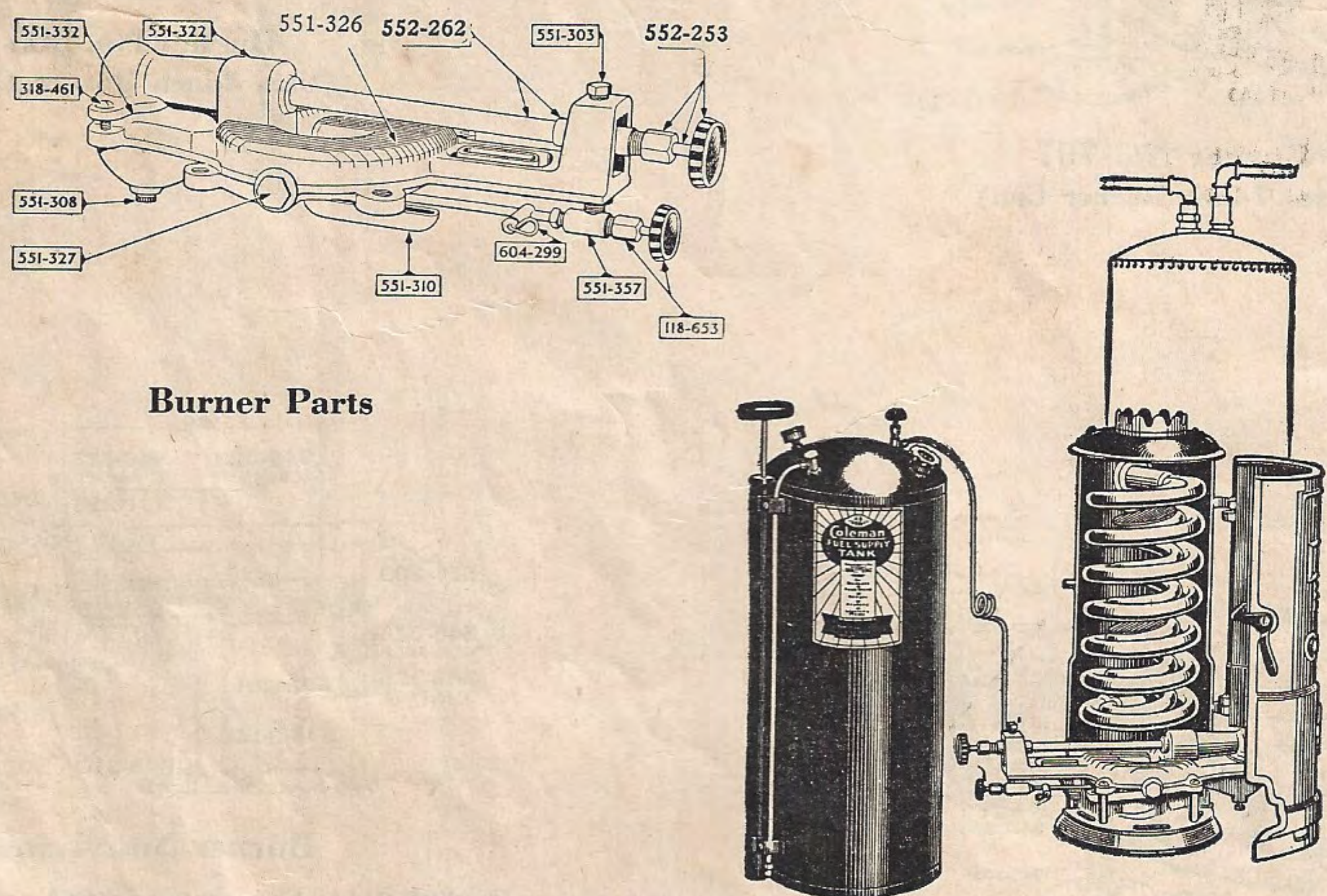
Water Heater No. 463T (Match-Generating)
