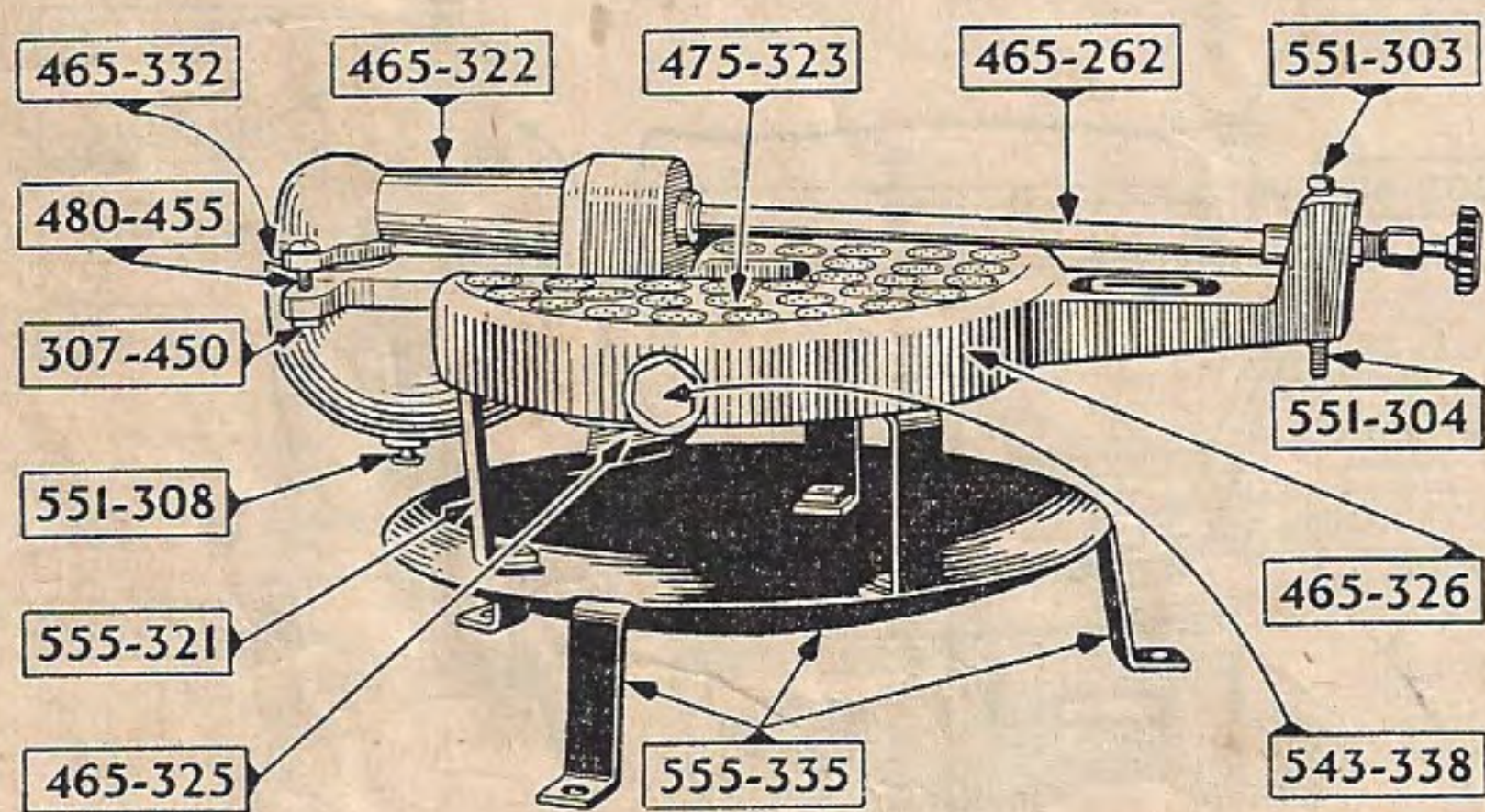
Burner No. 555
