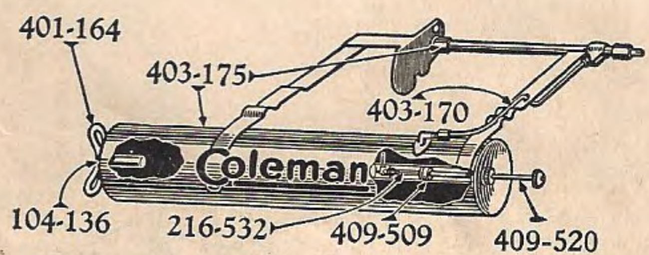
Camp Stove Nos. 2C and 9C
