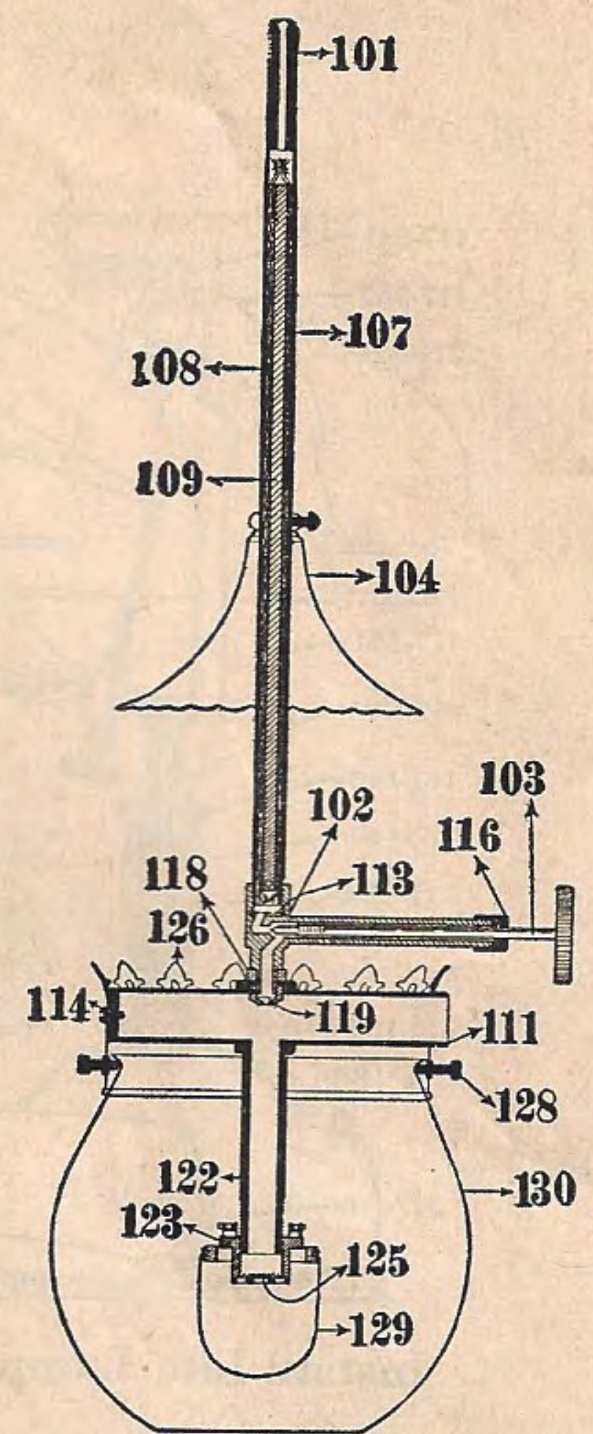
Ceiling Fixture System Lamp No. 1
