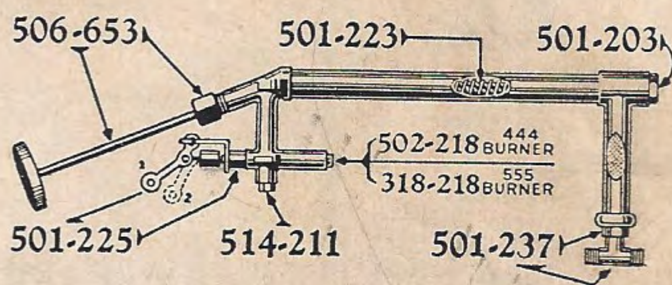
Generator No. 501-262
