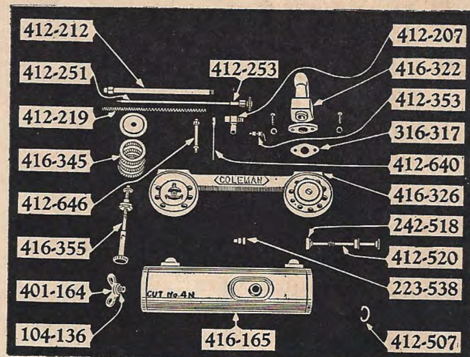
Camp Stove Nos. 2G, 9G
