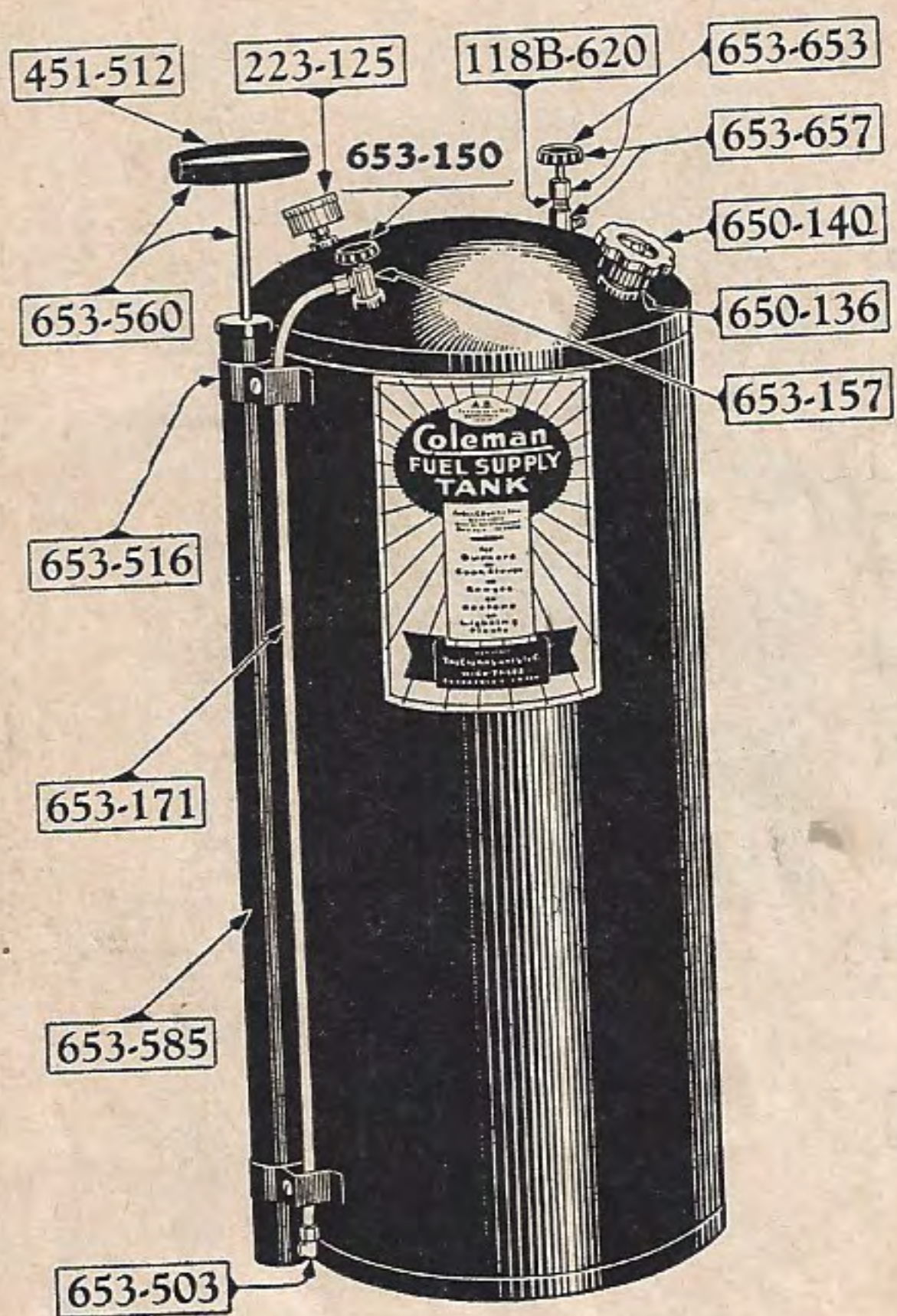
Tank No. 653B
