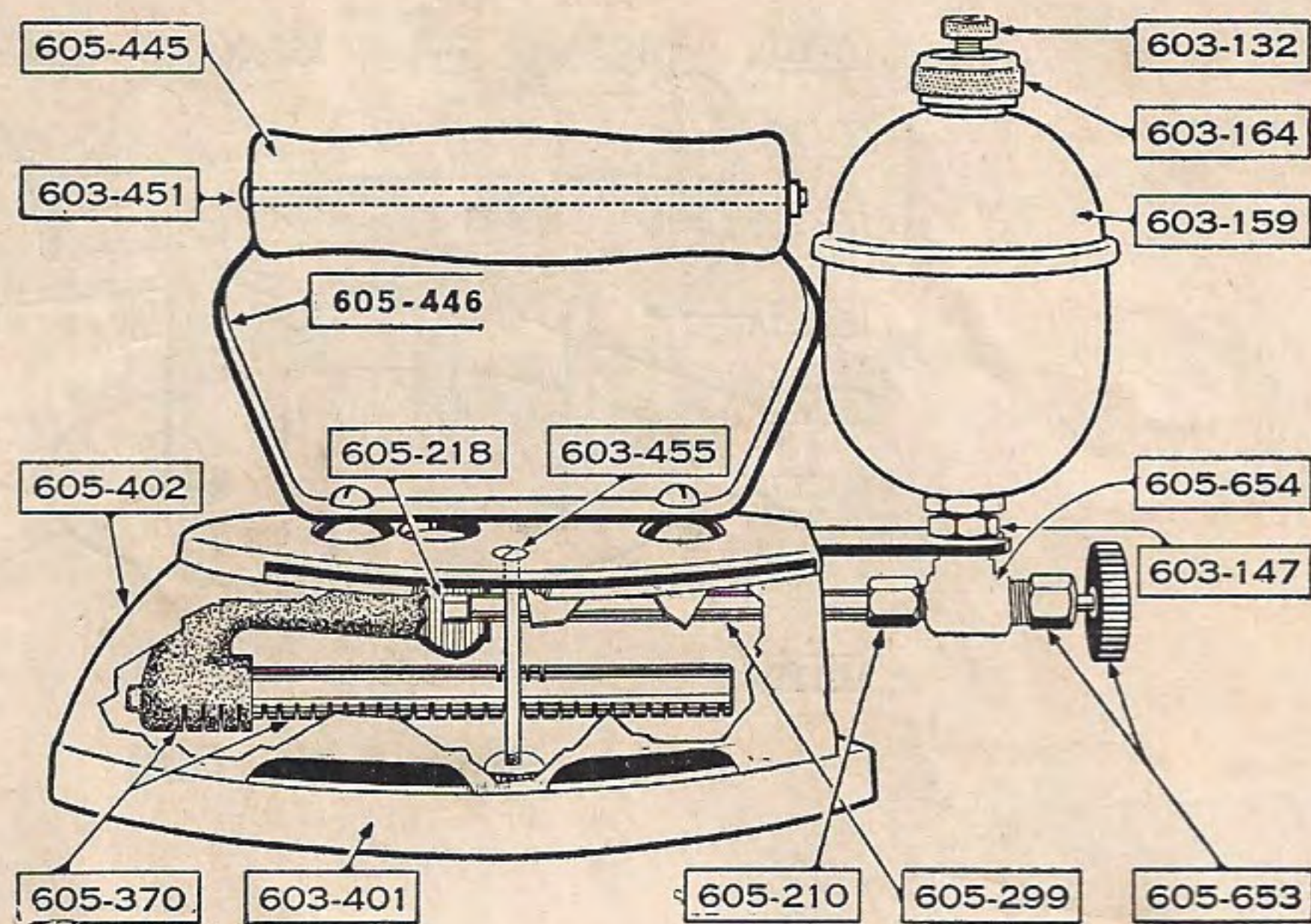
Iron No. 5 (Torch-Generating)
