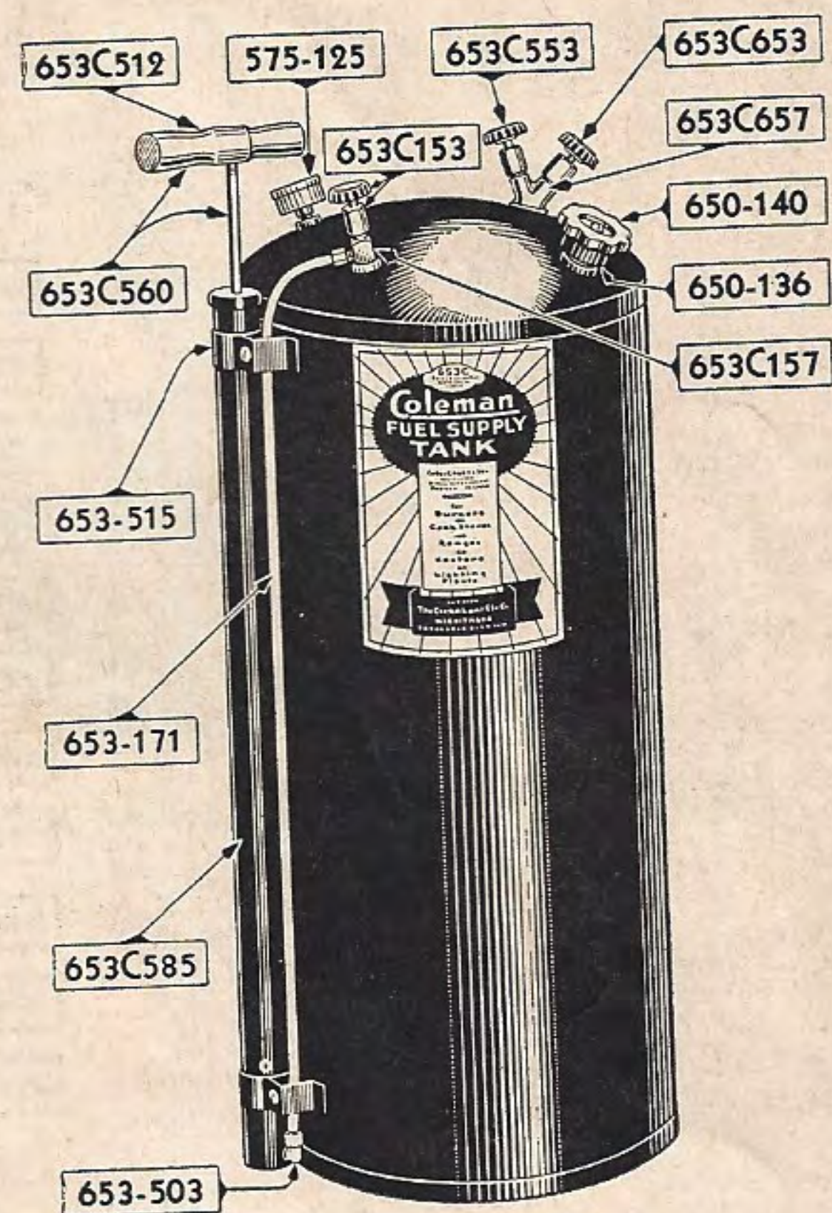
Tank No. 653C
