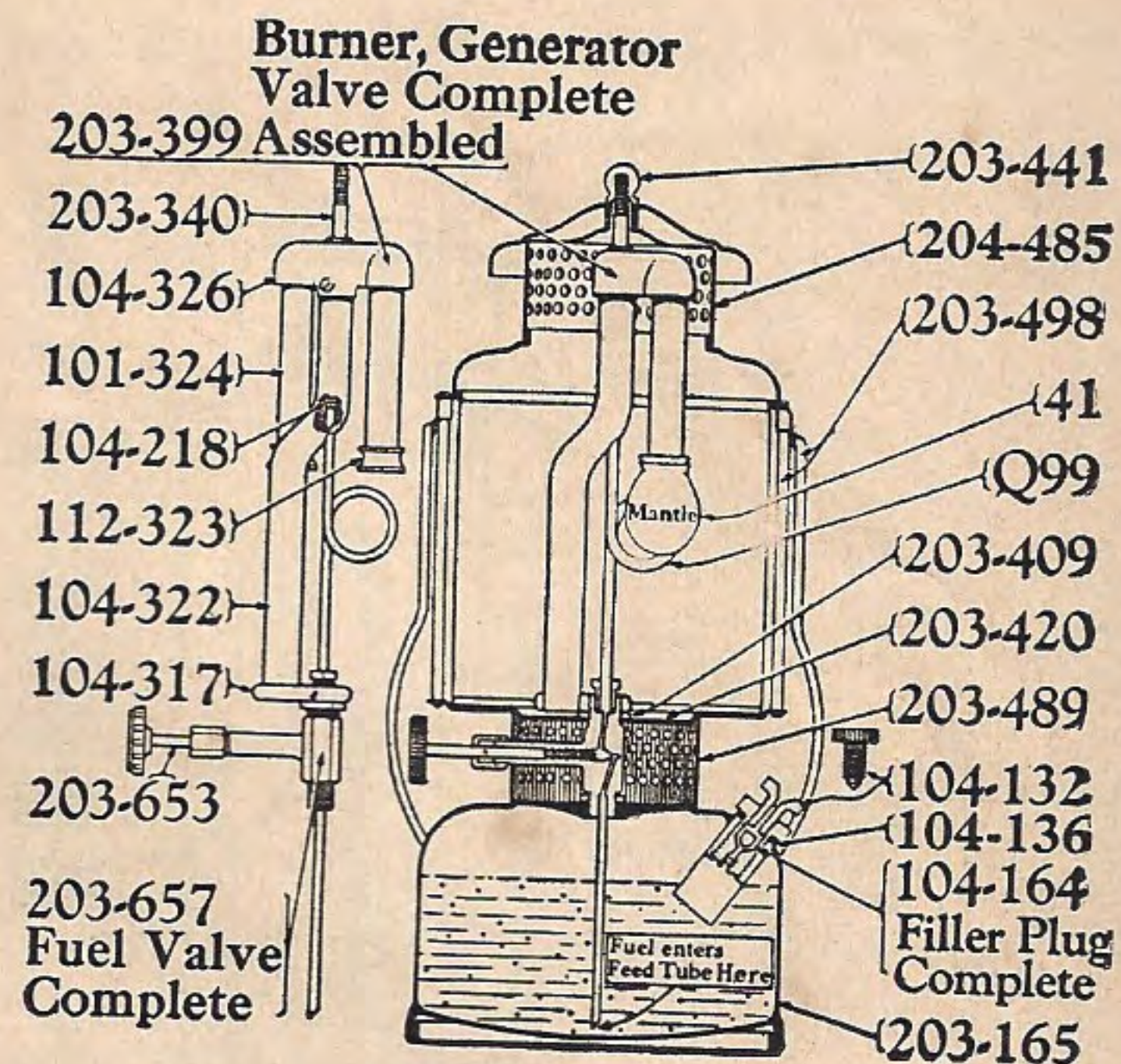
Match-Generating Quick-Lite Lantern No. L327 (with separate pump)
