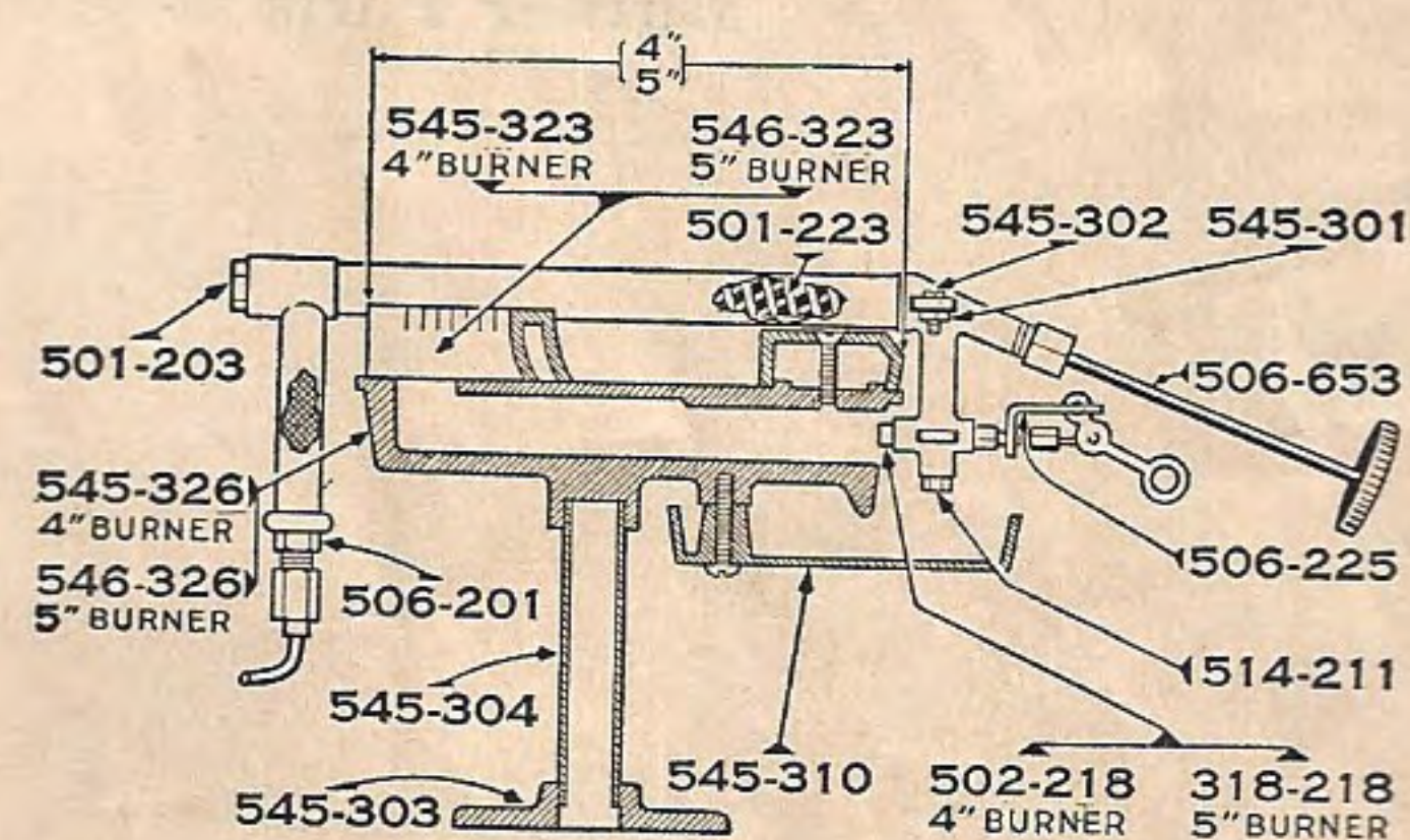
Burner Nos. 4 and 5
