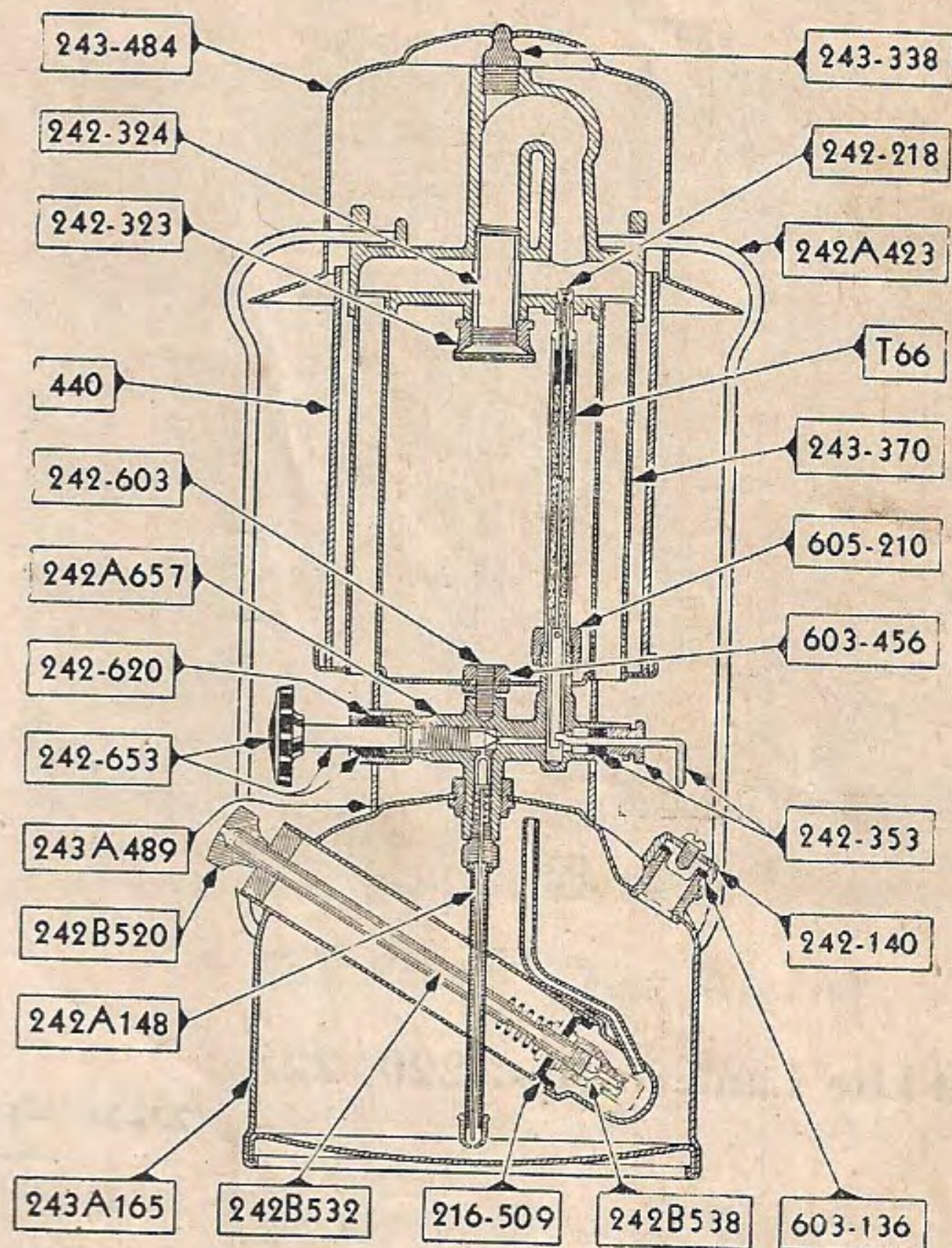
Instant-Lite Lantern No. 243A
