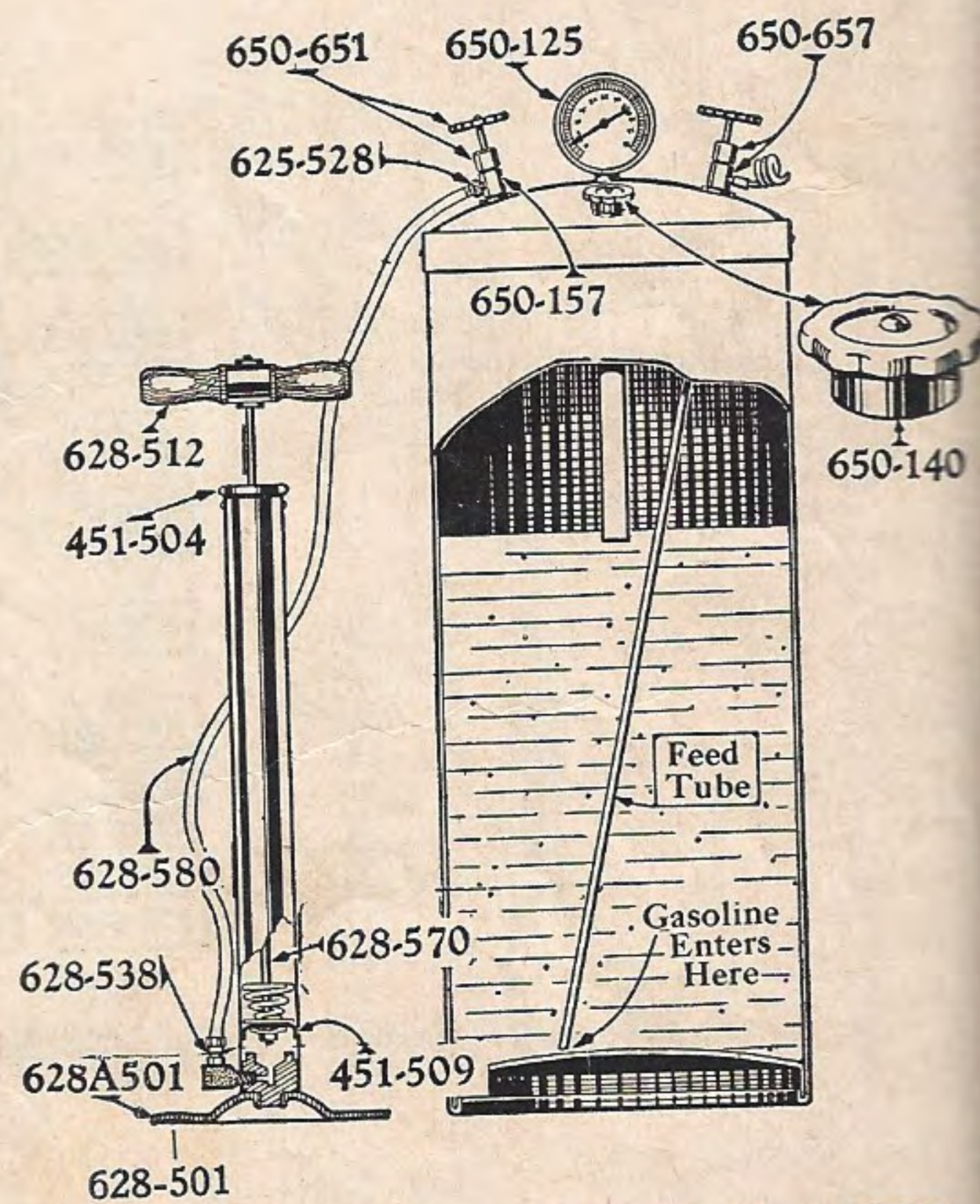
Pump No. 628 and Tank No. 652C
