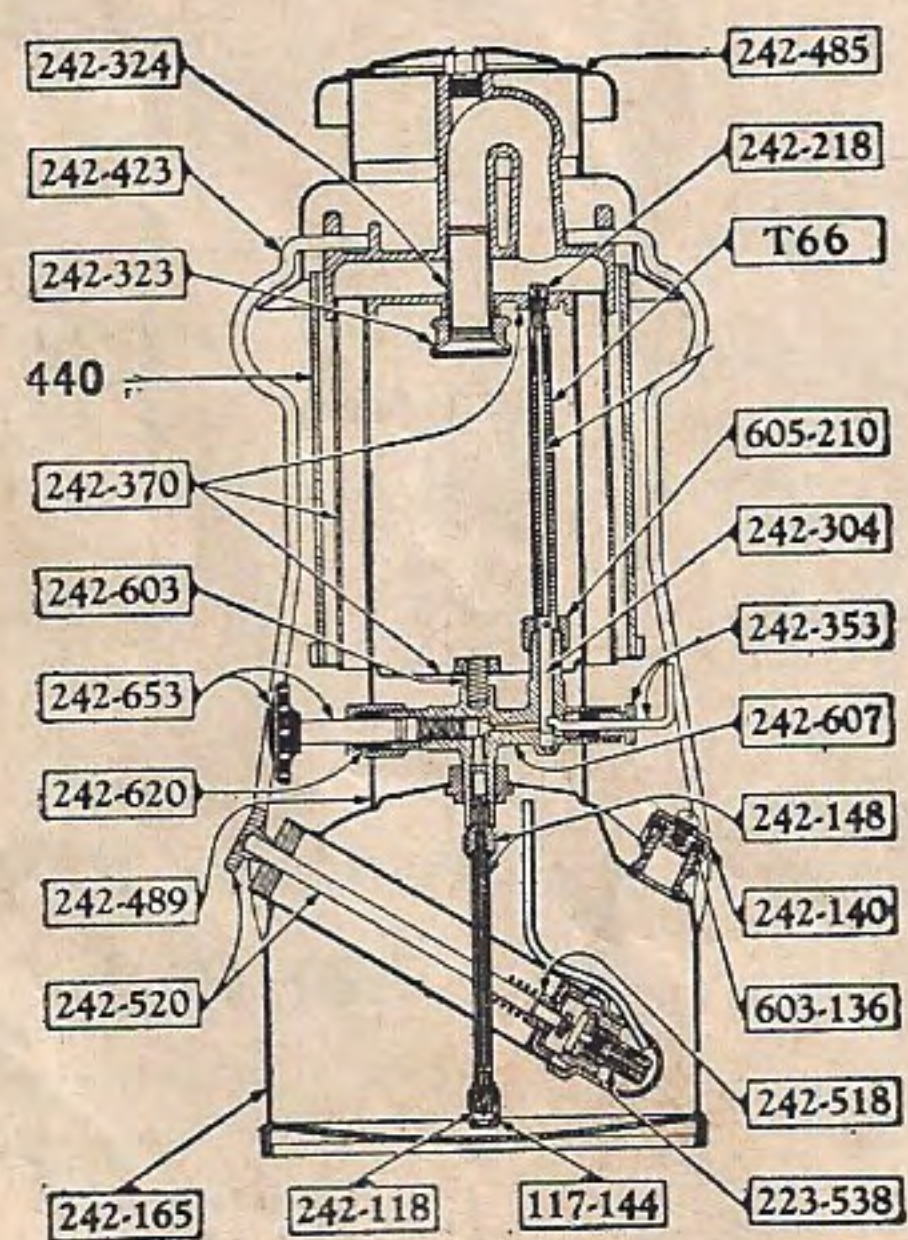
Instant-Lite Lantern No. 242
