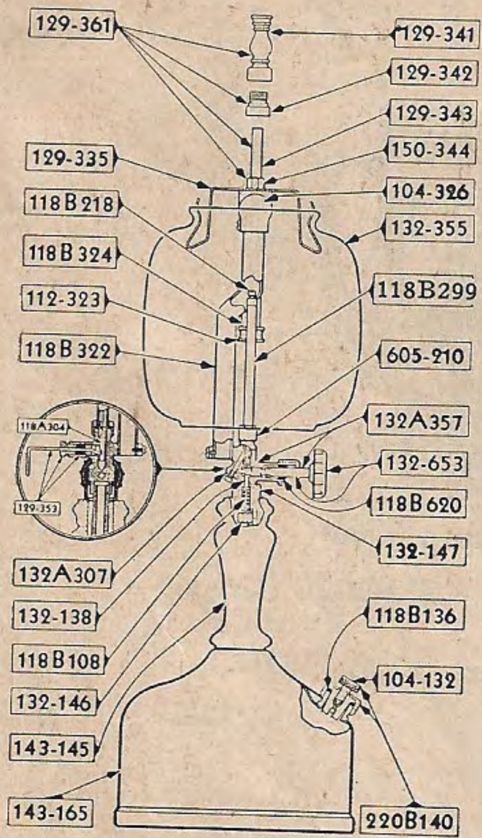
Instant-Lighting Lamp No. 143
