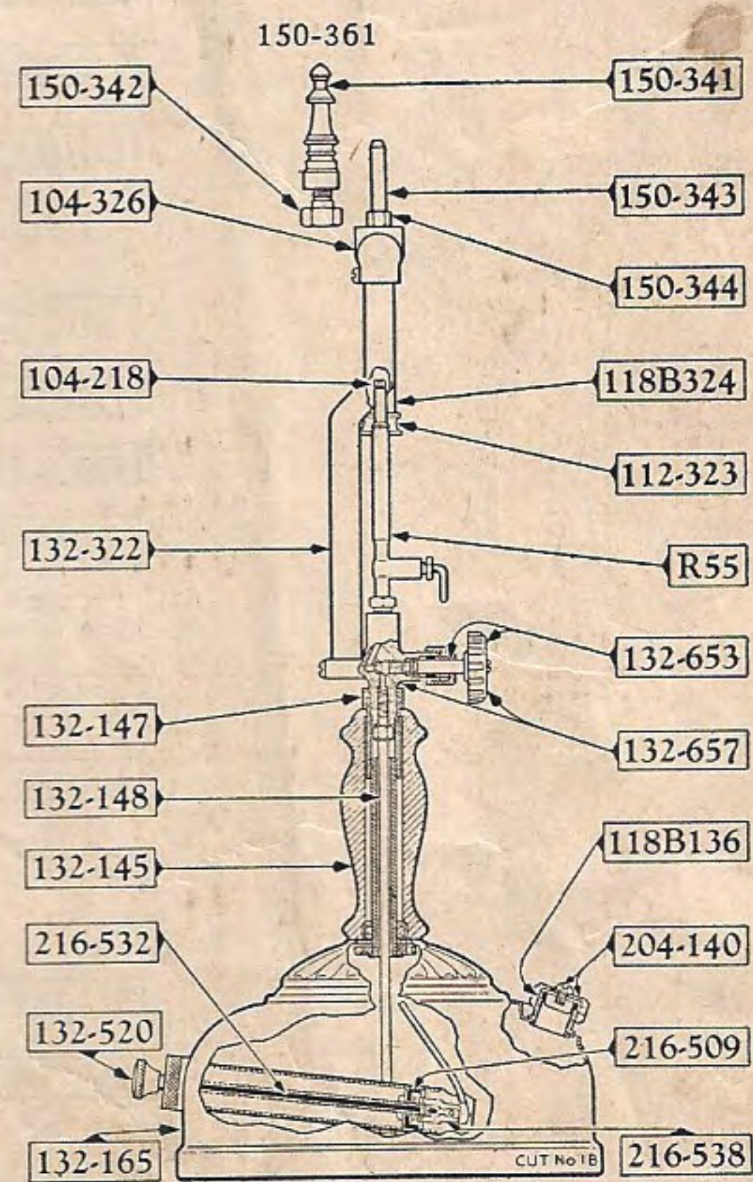
Instant-Lighting Lamp No. 132P
