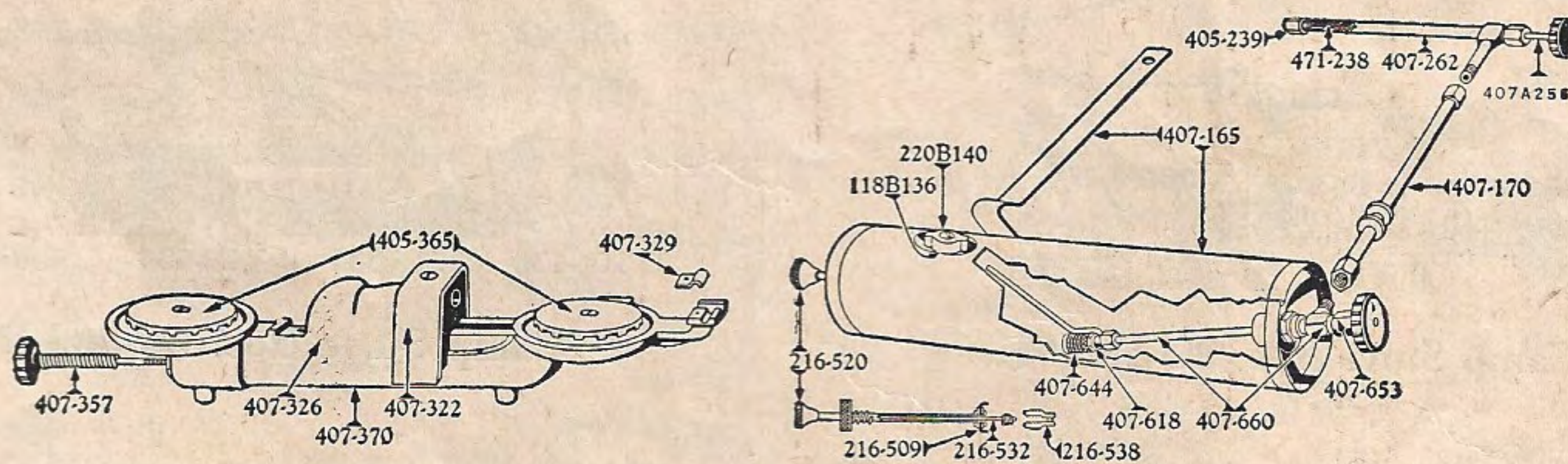
Camp Stove Nos. 2E, 9E, 2F and 9F
