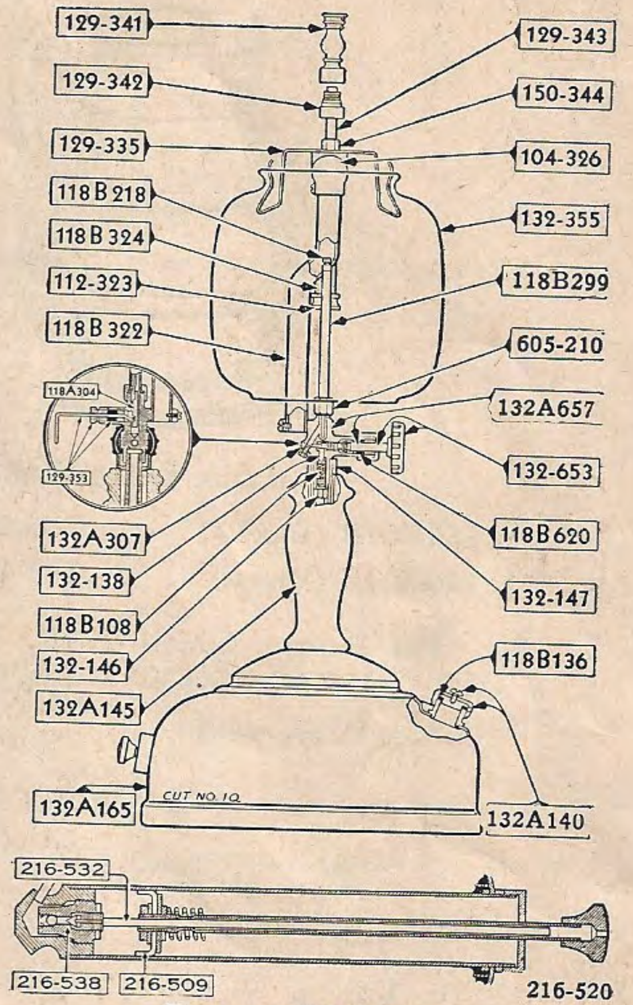
Instant Lighting Lamp No. 132A
