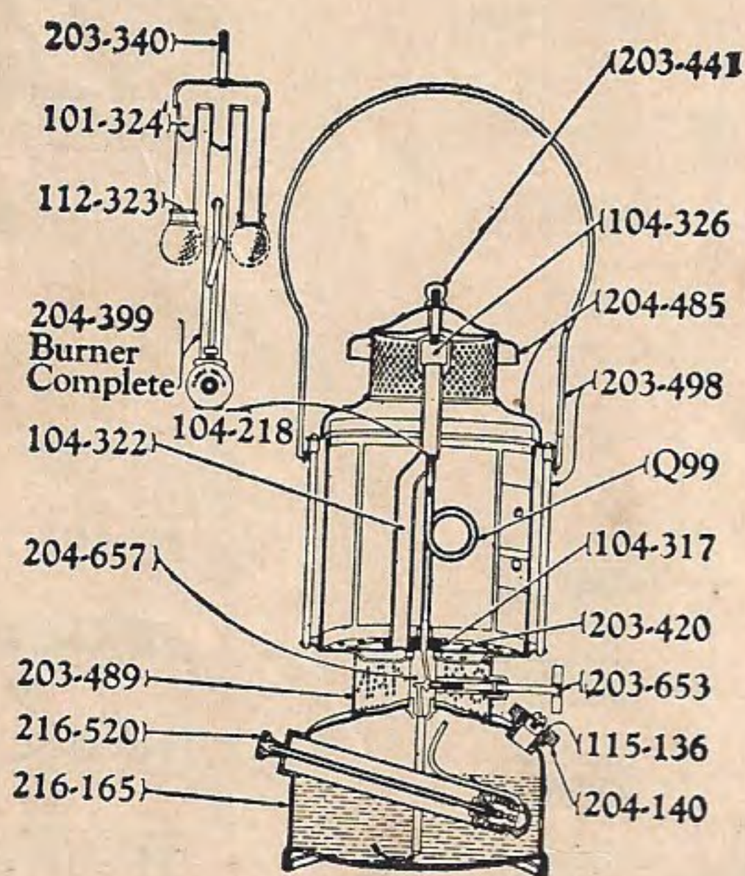
Match-Generating Lantern No. L427
