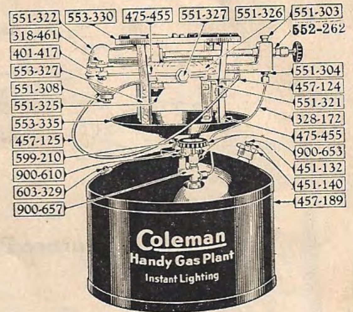
Handy Gas Plant Nos. 457, 457G and 575
