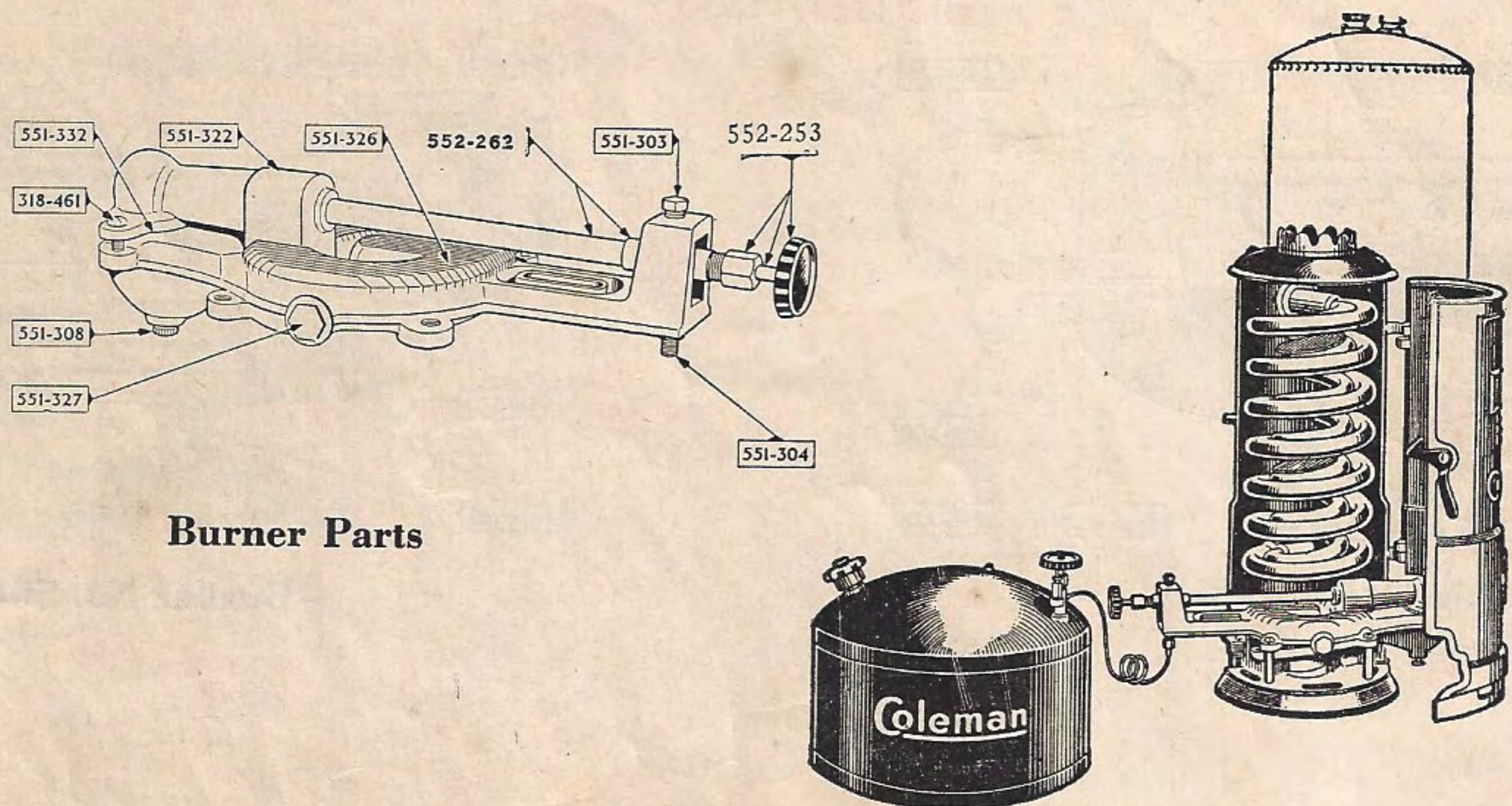
Water Heater No. 463G (Instant-Lighting)
