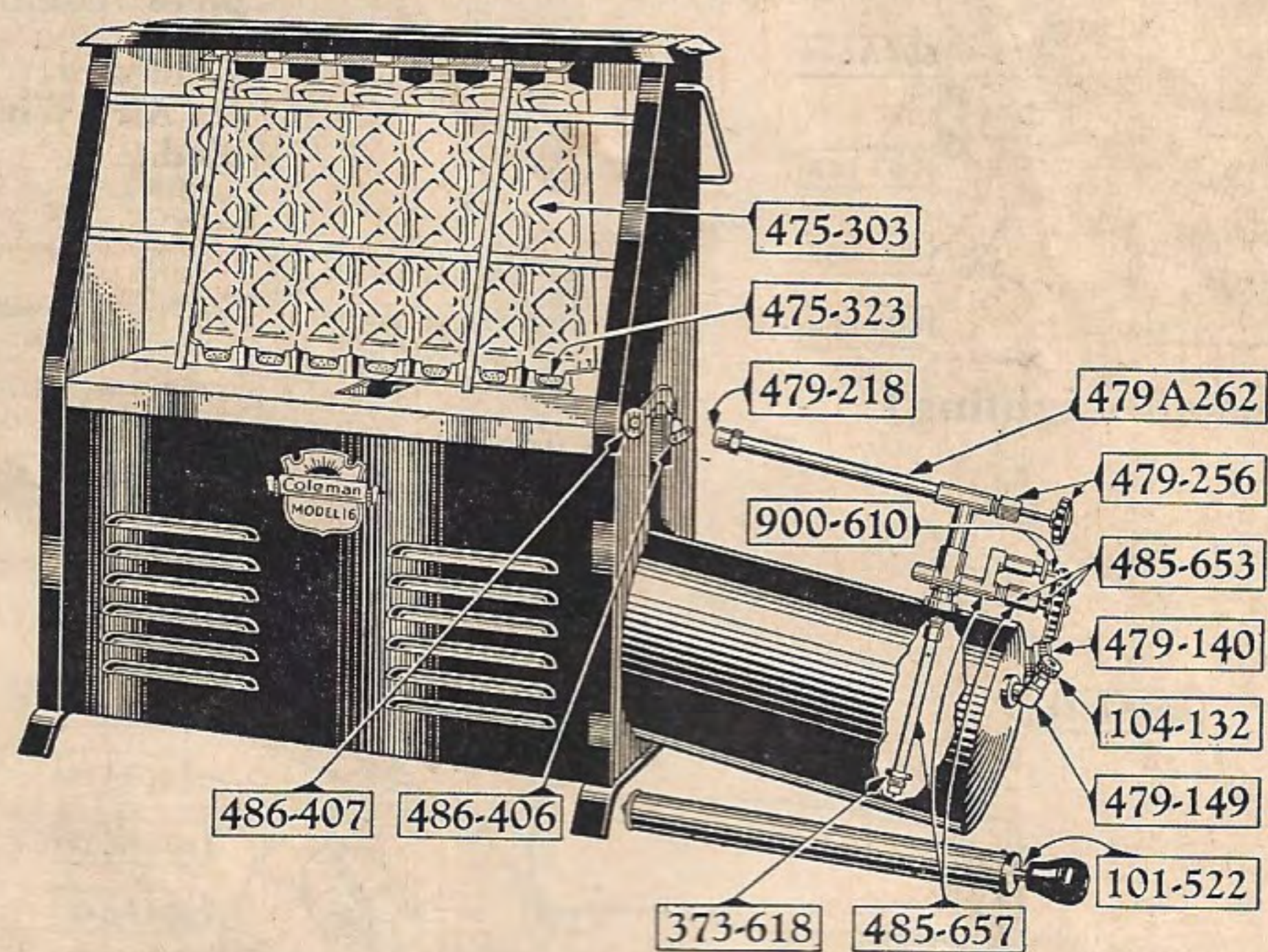
Radiant Heater No. 16 (Instant-Lighting)
