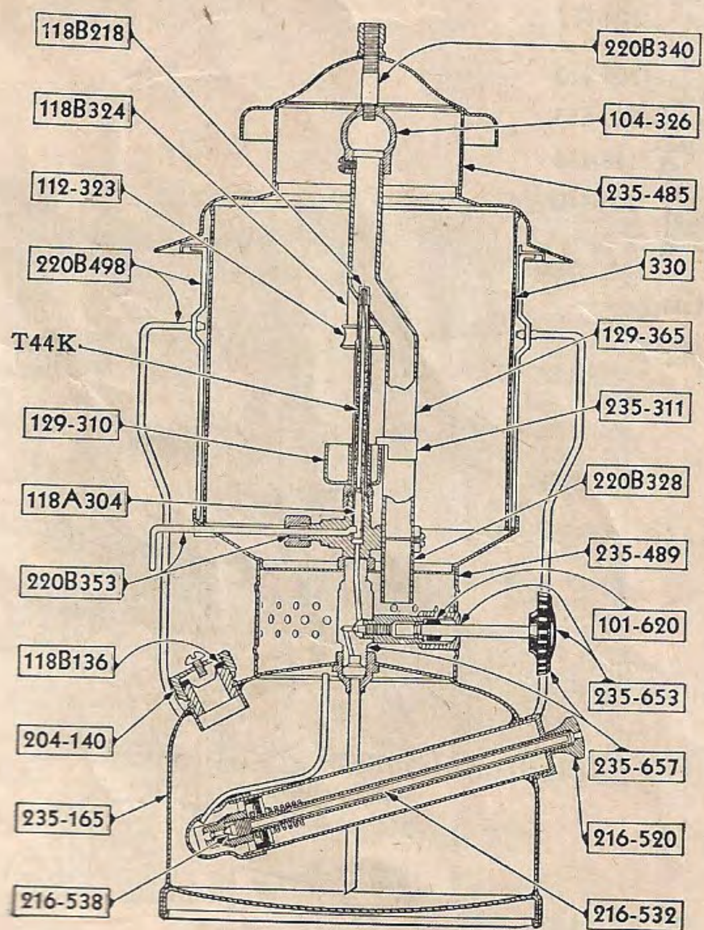
Kerosene Double Mantle Lantern No. 235 Alcohol Generating
