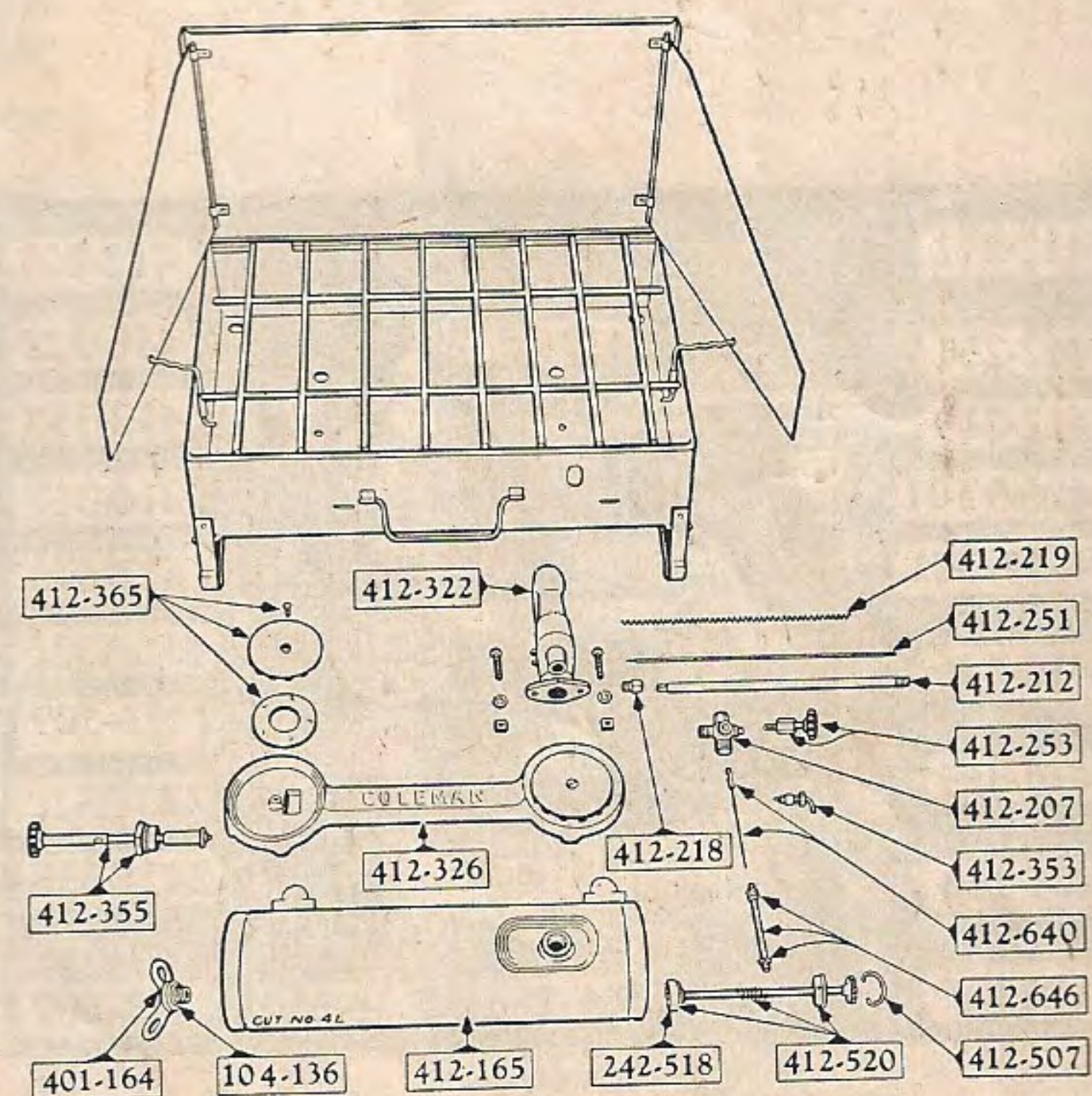
Camp Stove No. 6F
