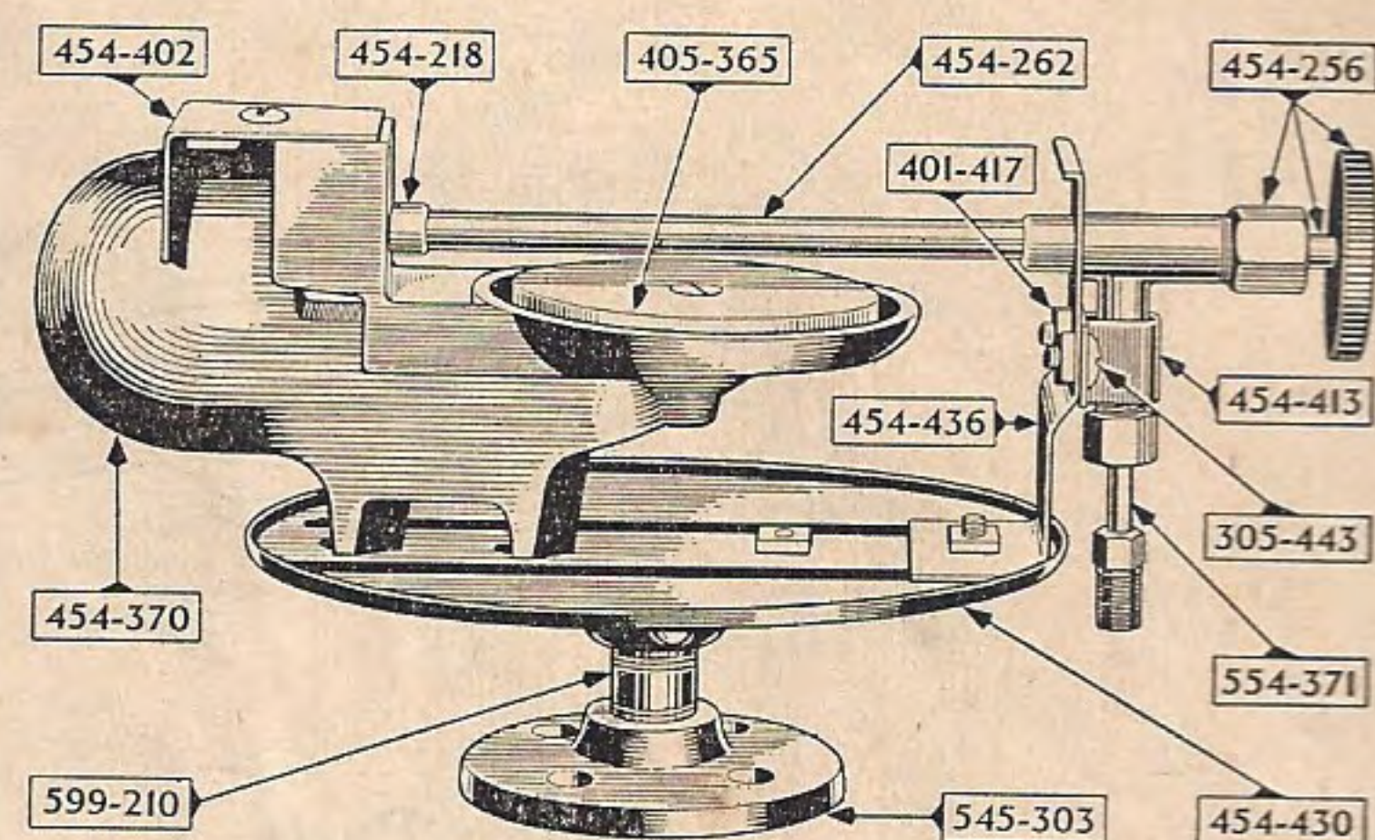
Burner No. 554
