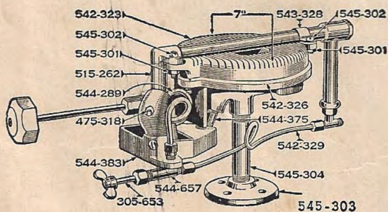
Burner No. 707 (Uses 7-inch Burner Cap)
