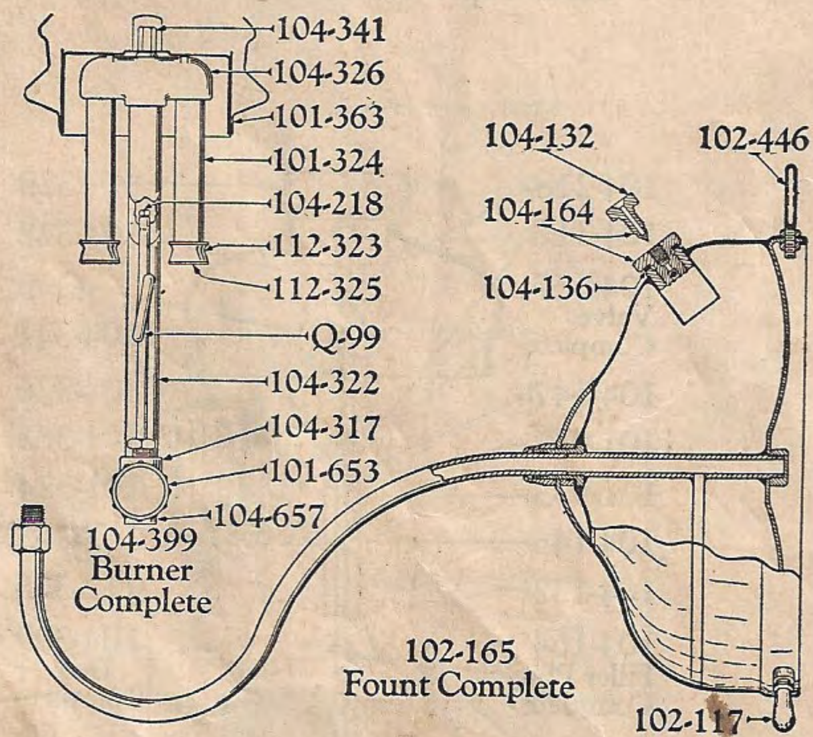
Model "B" Quick-Lite Bracket Lamp (With Separate Pump)
