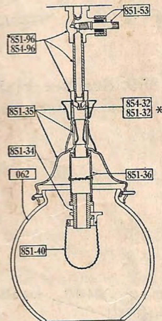
Burner Parts for Liquid Gas Lighting Fixtures
