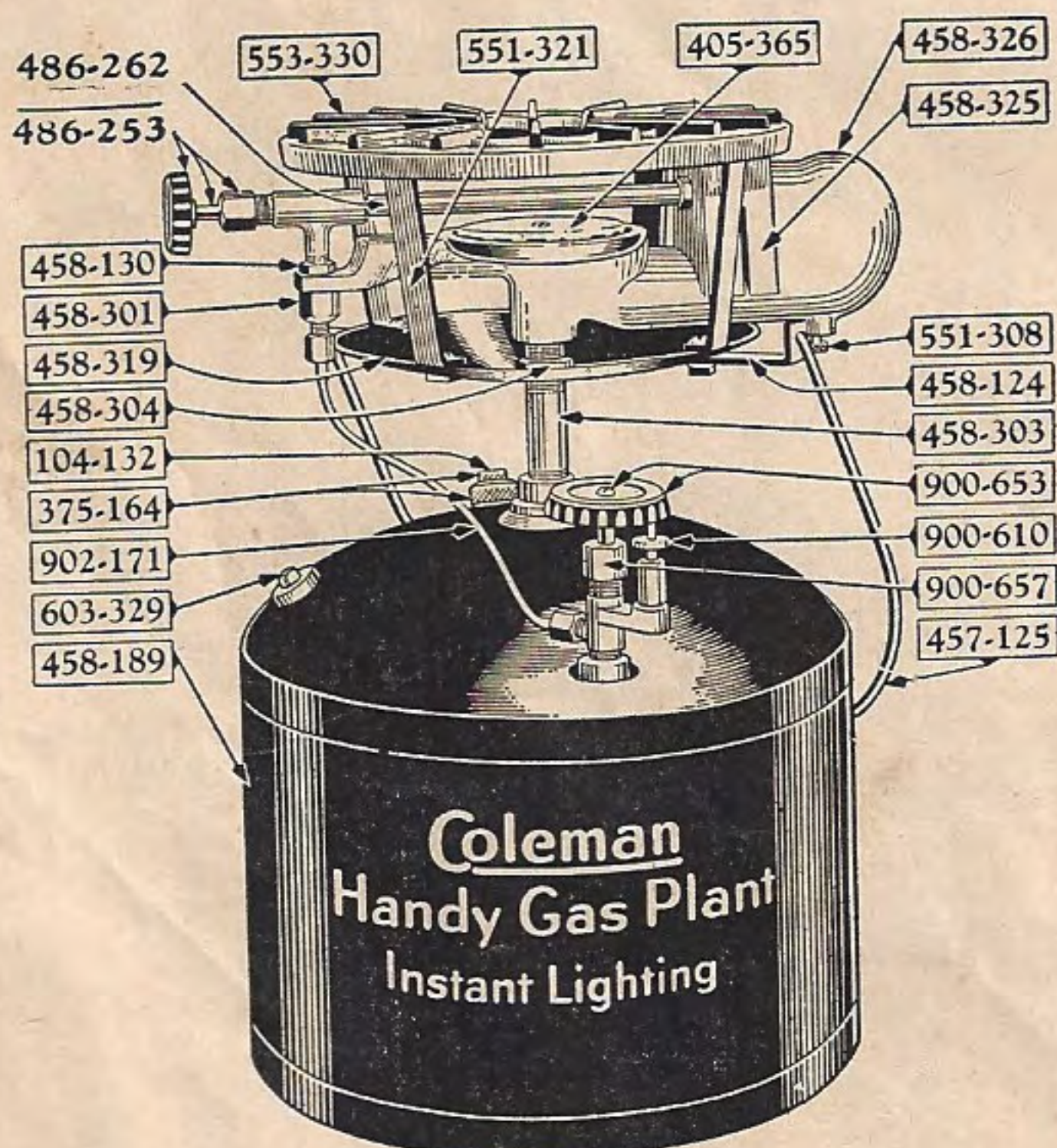
Handy Gas Plant Nos. 458 and 458G
