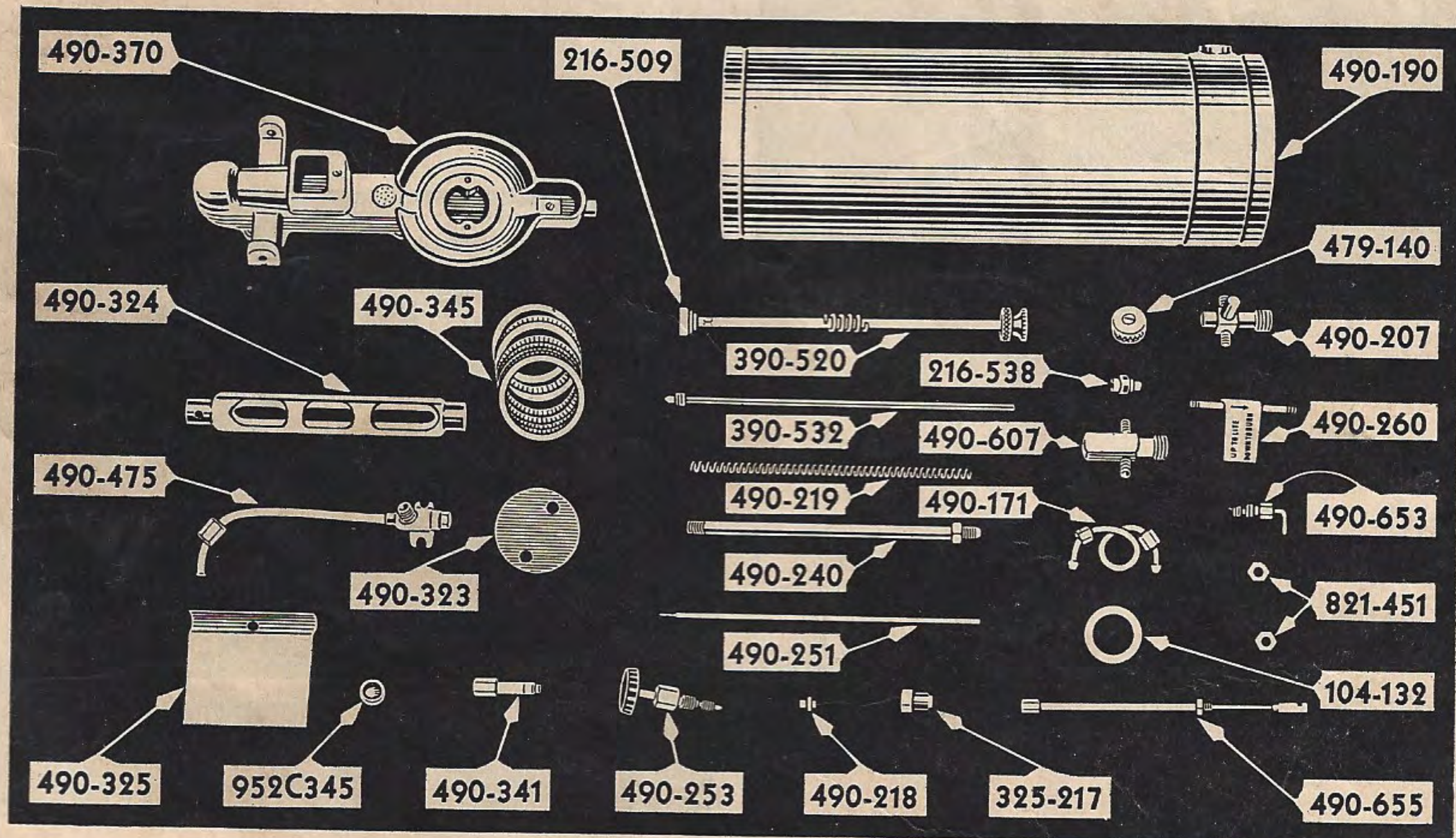
Trailer Heater No. 490
