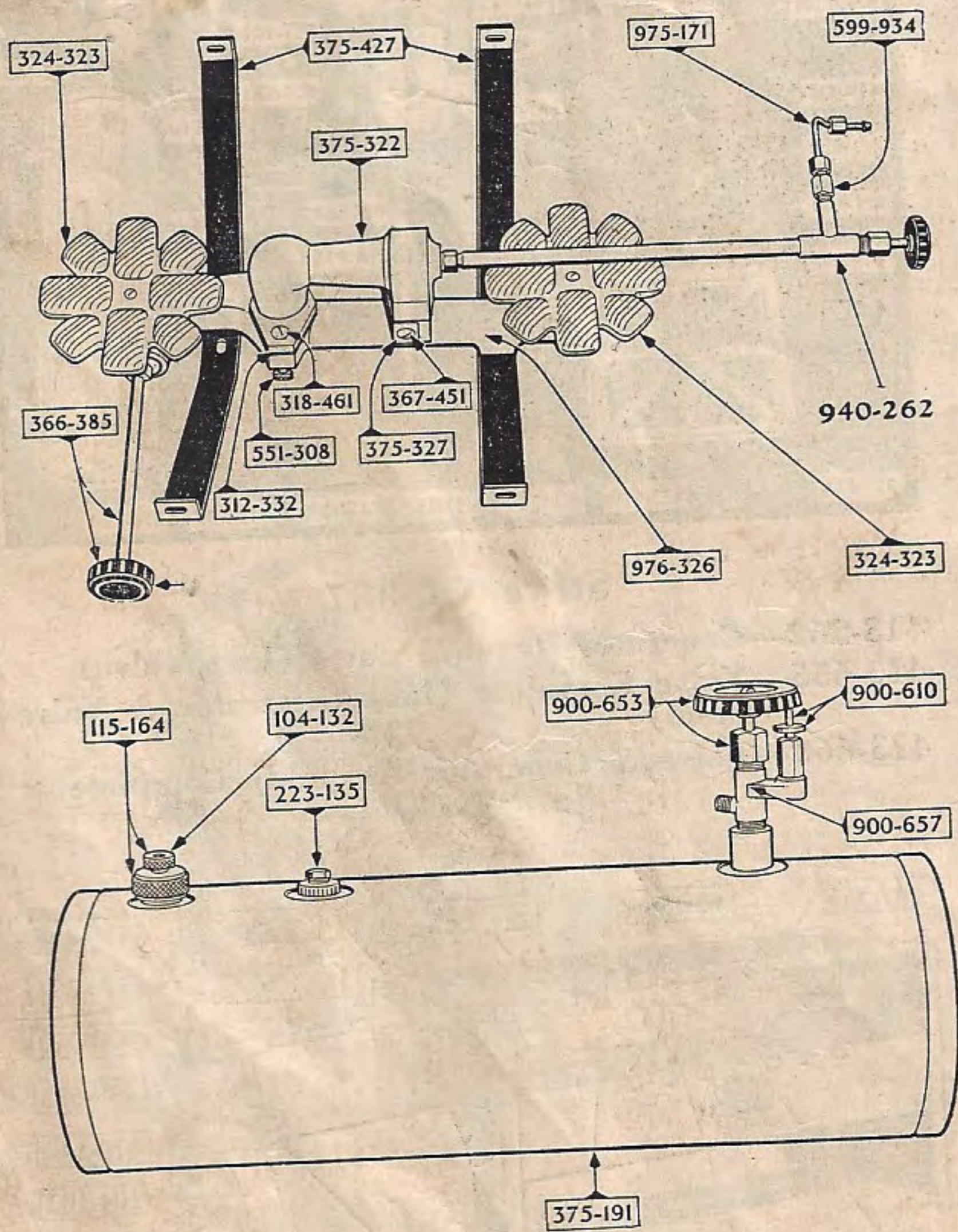
Cabin Stove No. 376
