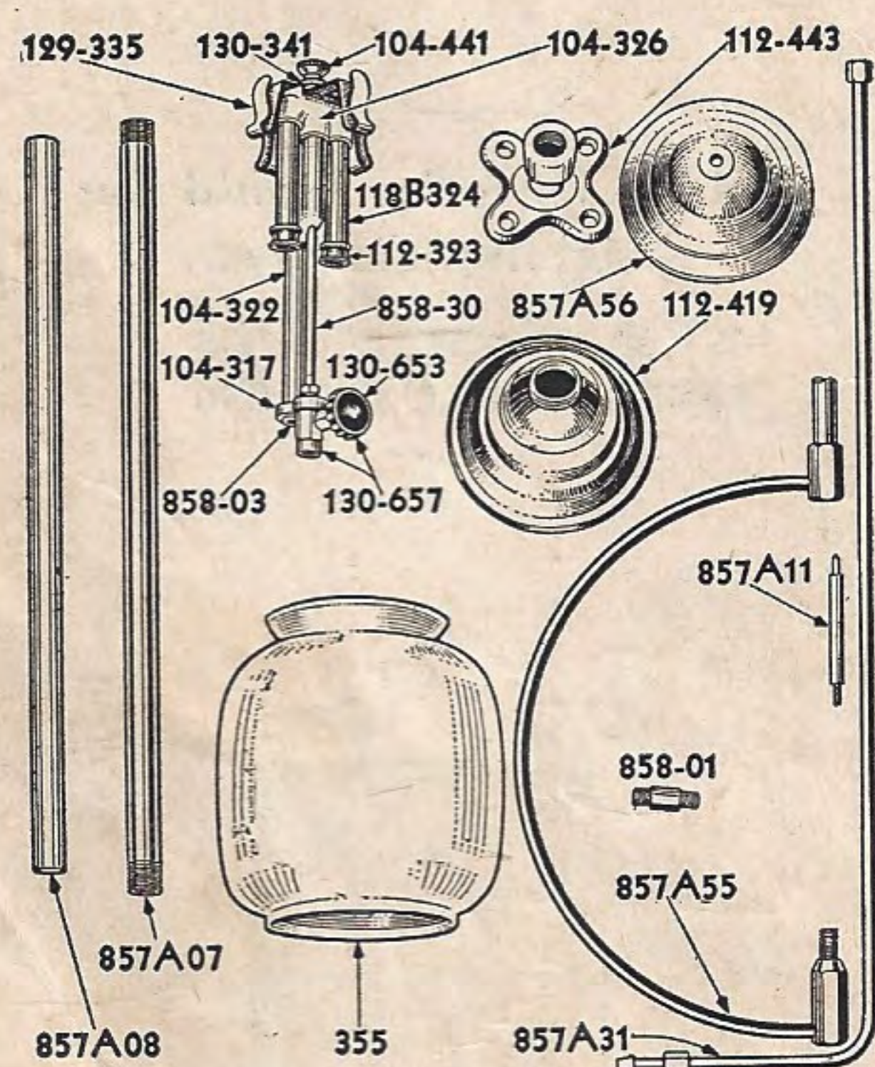
No. 857A Single-Drop Fixture
