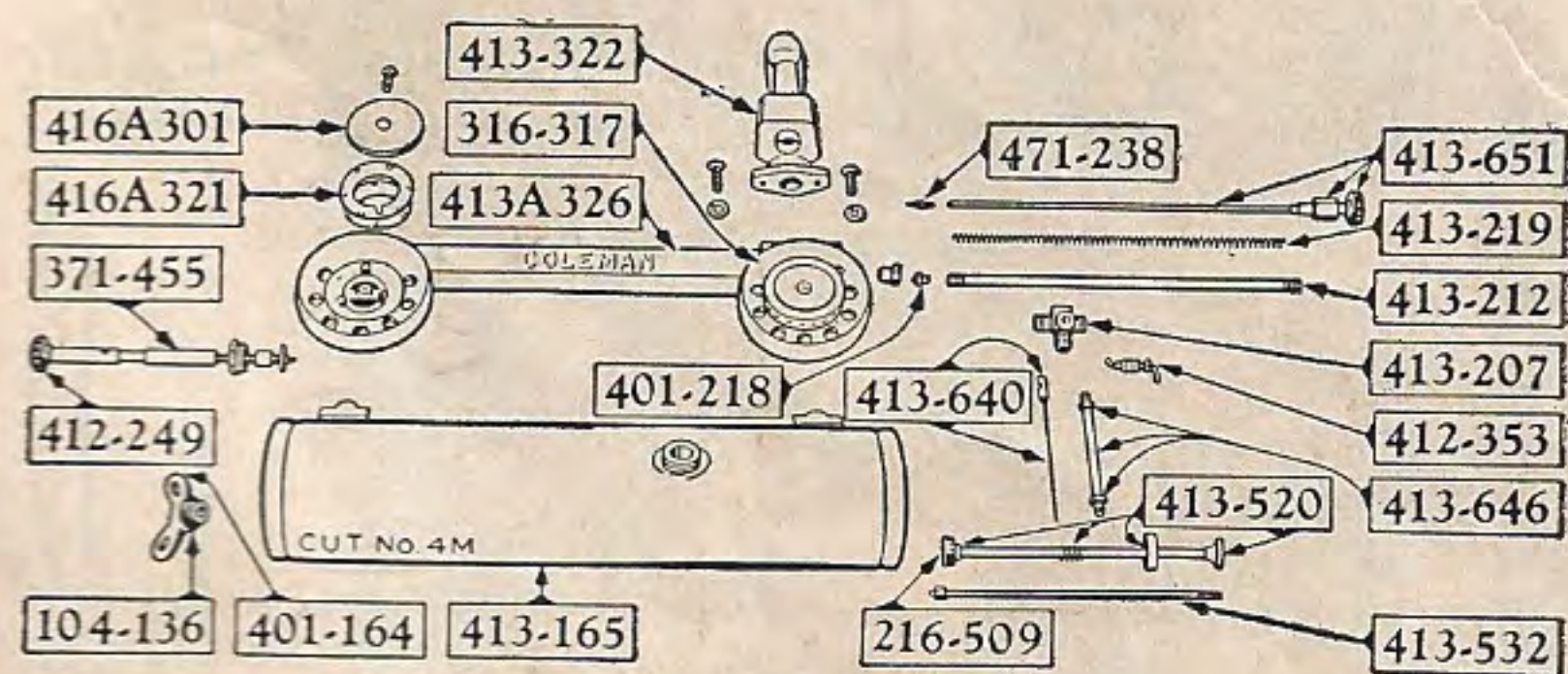
Stove No. 371
