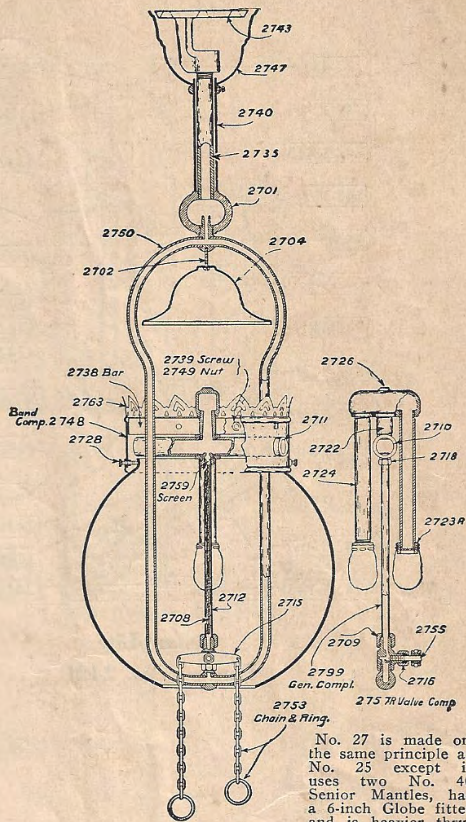
Ceiling Fixture System Lamp No. 27
