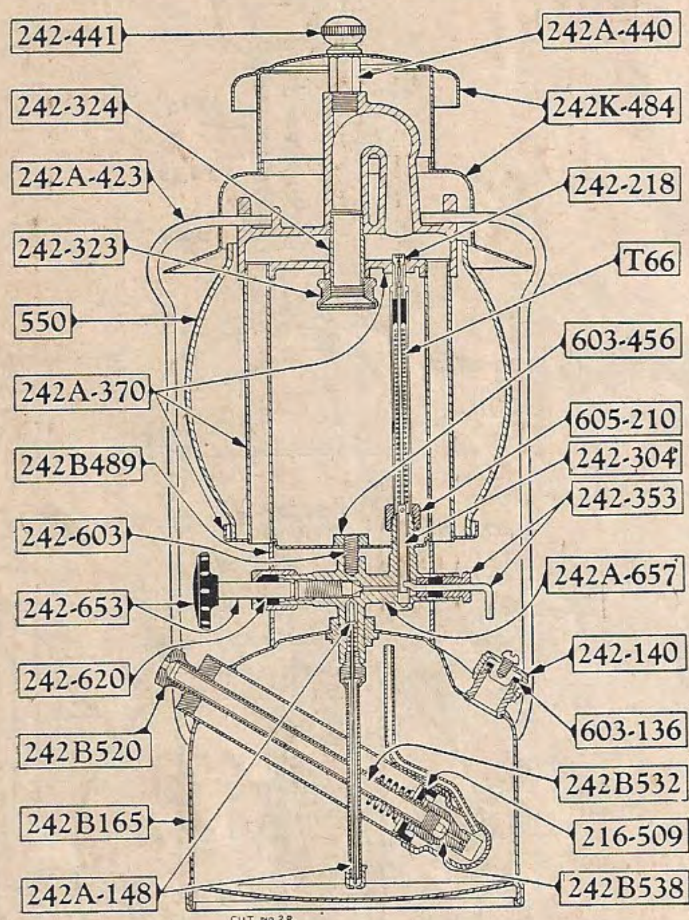
Instant-Lite Lantern No. 242B
