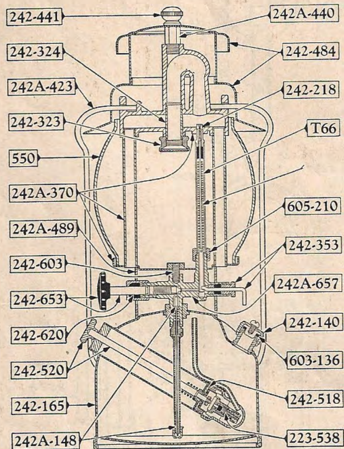
Instant-Lite Lantern No. 242A
