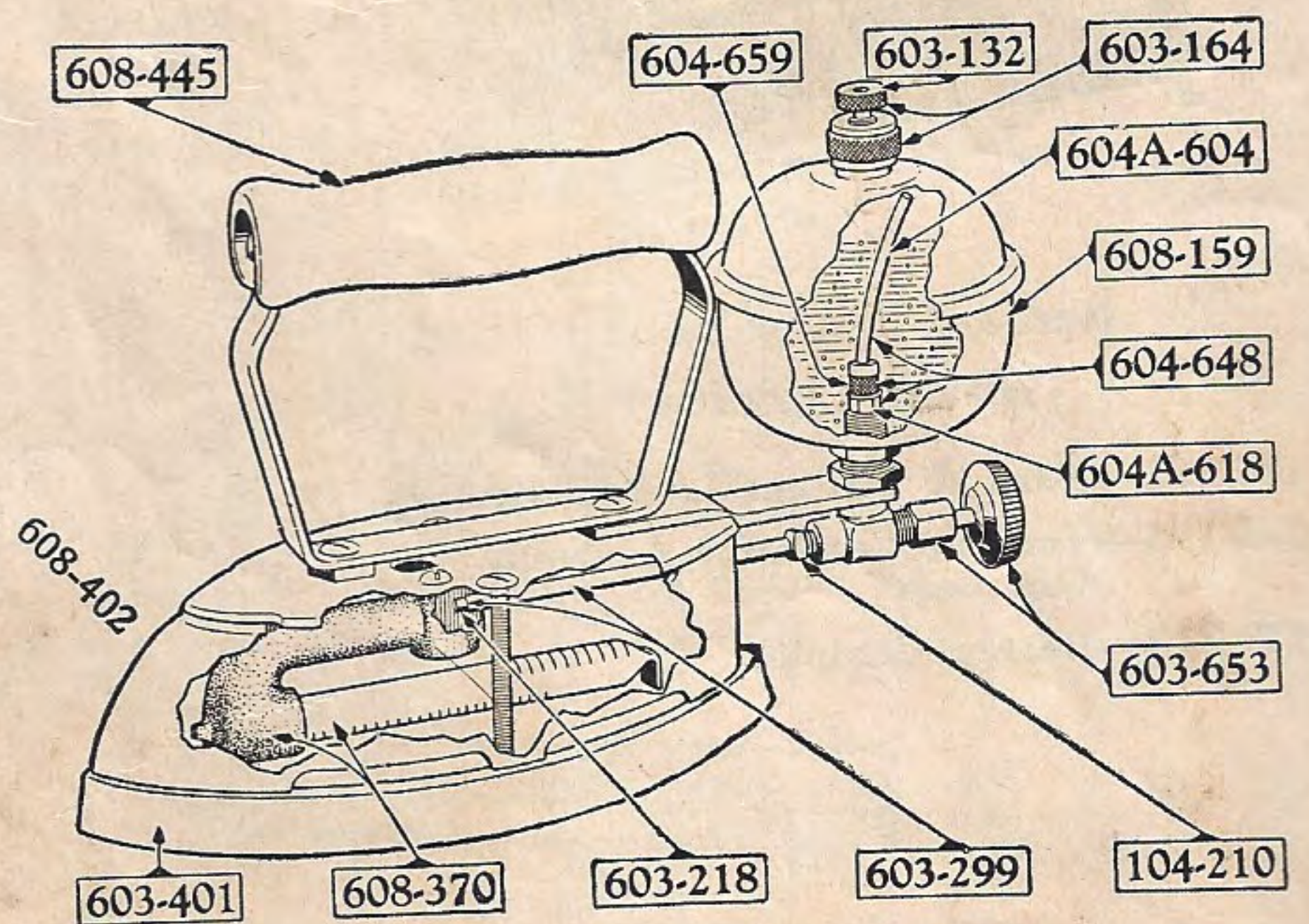
Iron No. 8 (Instant-Lighting)
