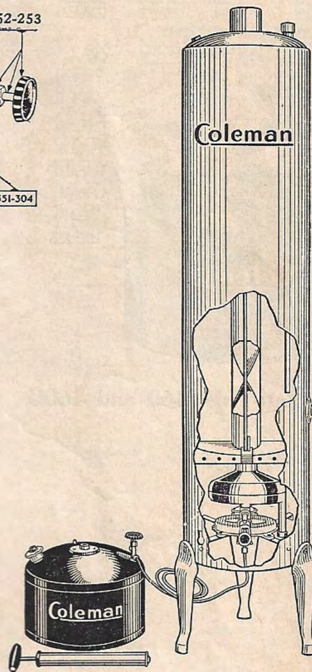
Water Heater No. 464 (Instant-Lighting)
