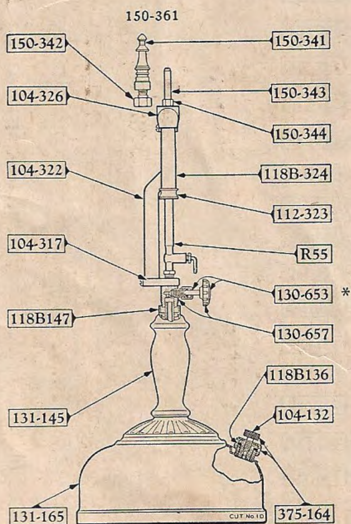
Match-Generating Lamp No. 131P
