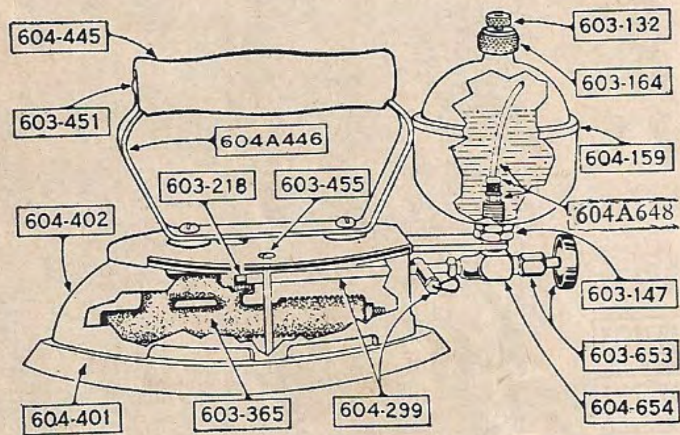
Iron No. 4A (Instant-Lighting)
