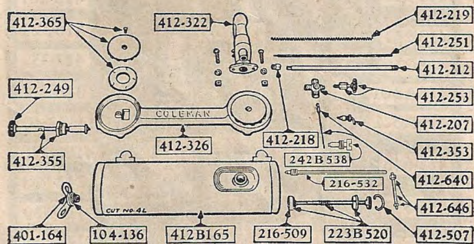
Camp Stove No. 6B
