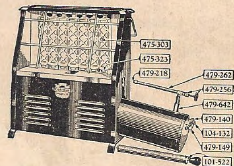
Radiant Heater No. 9 (Torch-Generating)
