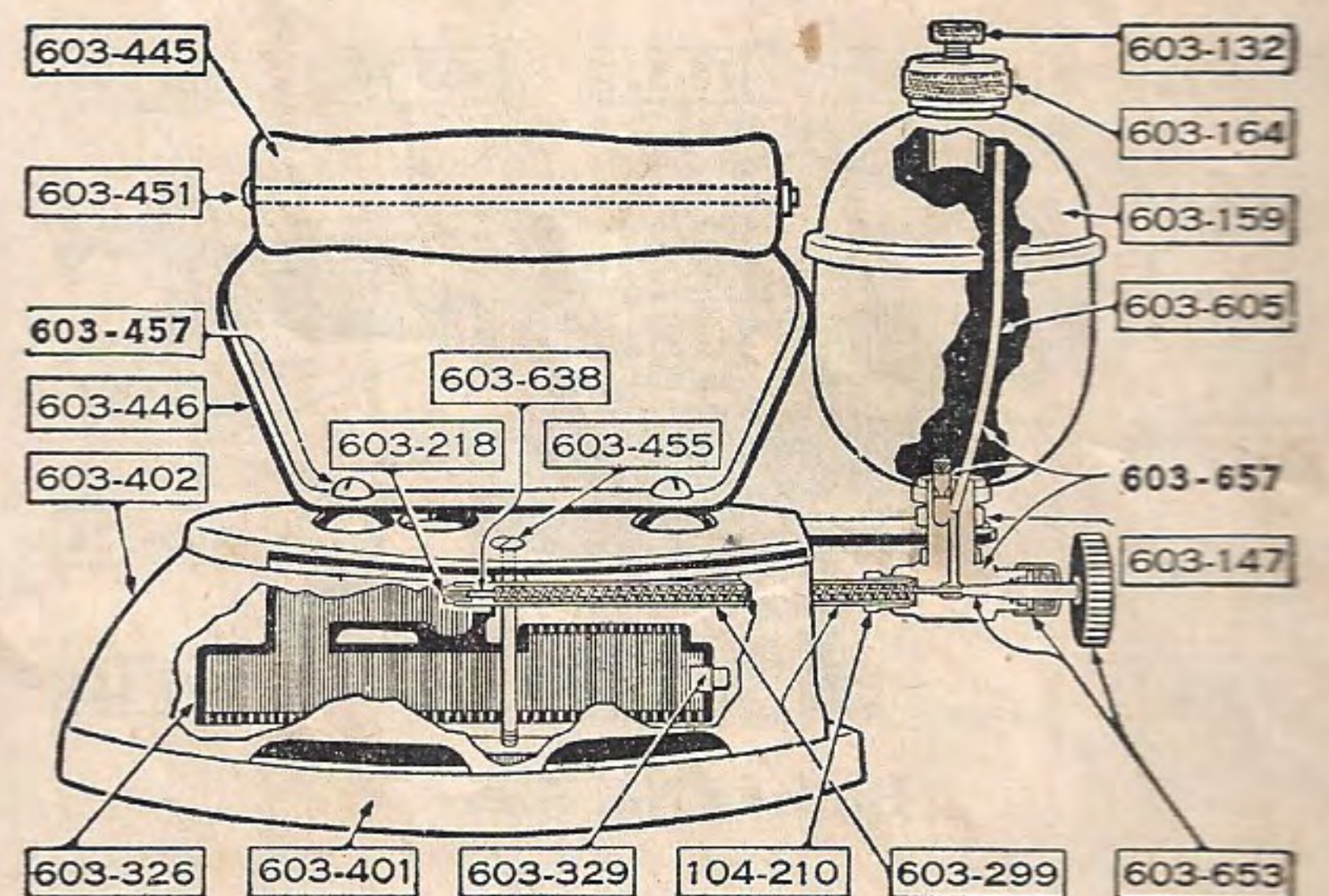
Iron No. 3 (Instant-Lighting)
