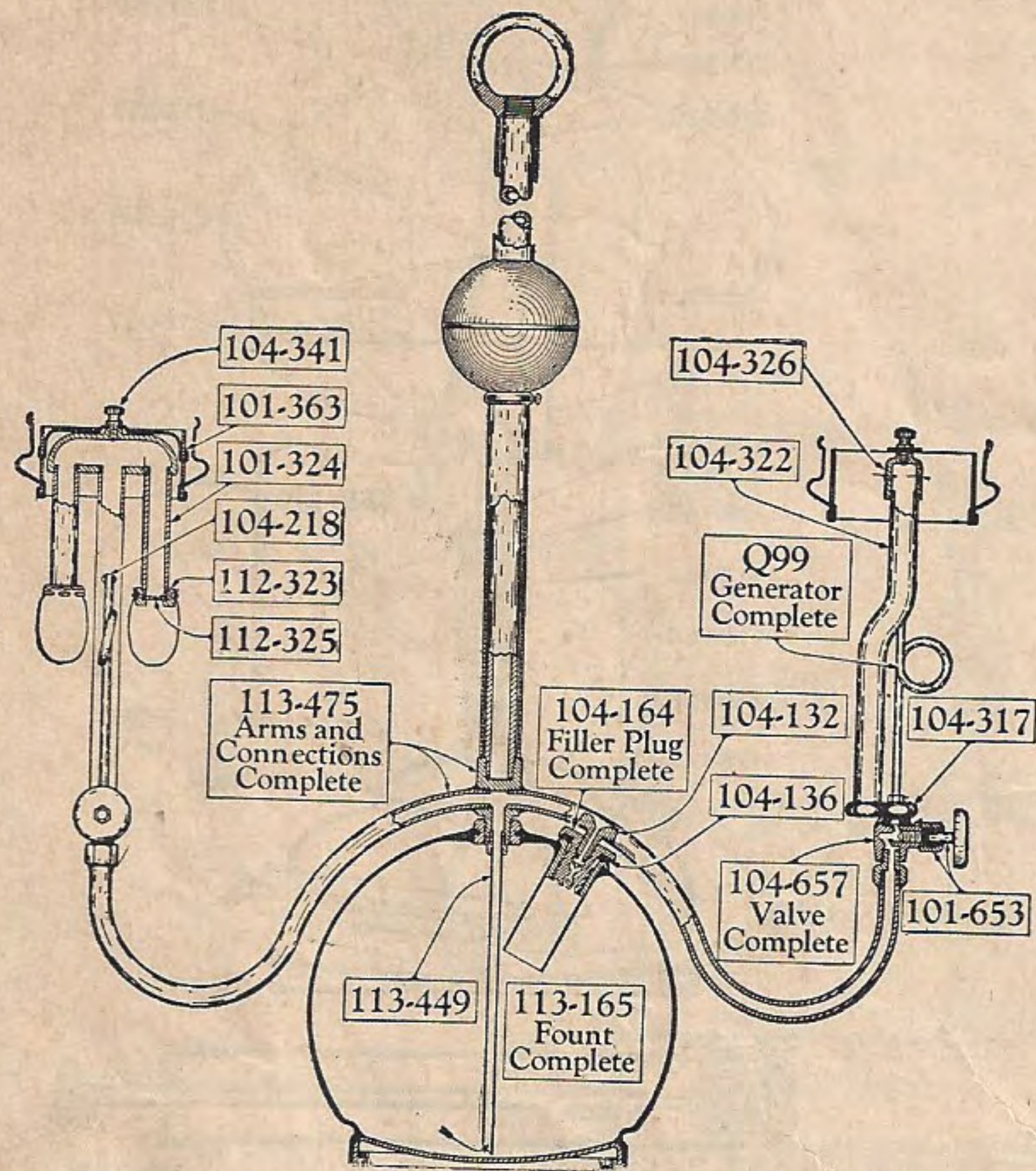
Quick-Lite Chandelier Lamp Model "P" (With Separate Pump)
