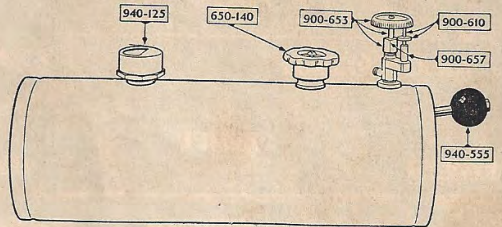
Tank Complete 974-191
