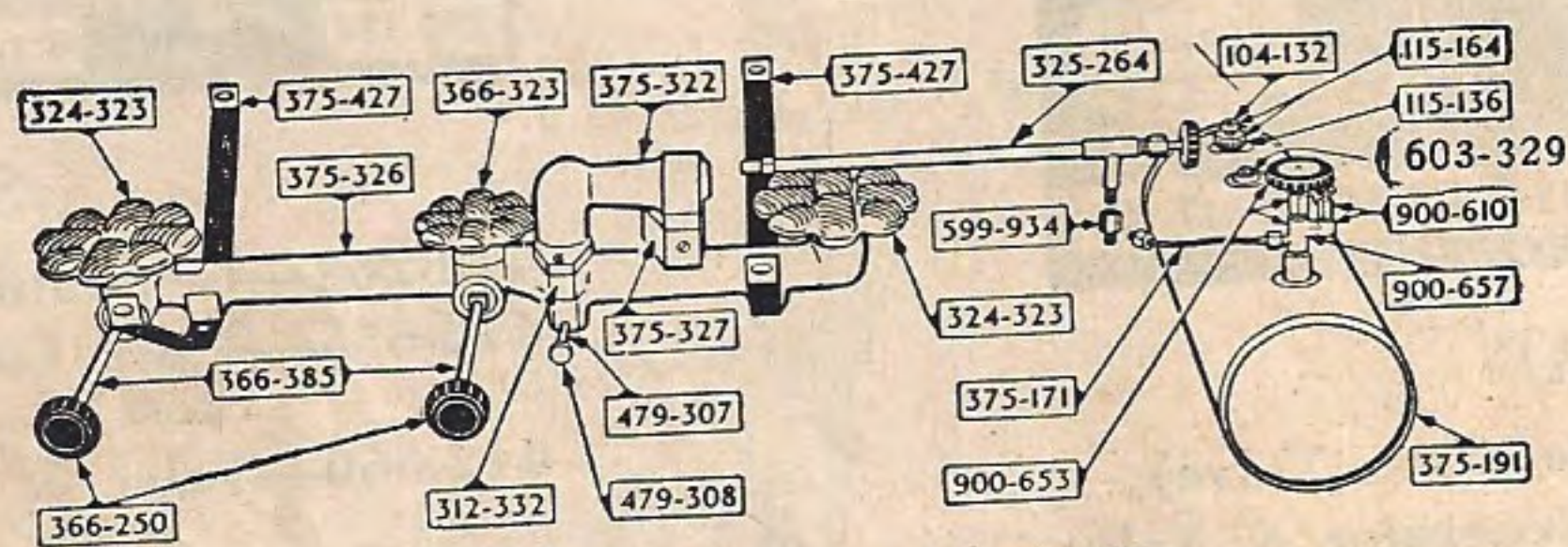
Cabin Stove No. 375
