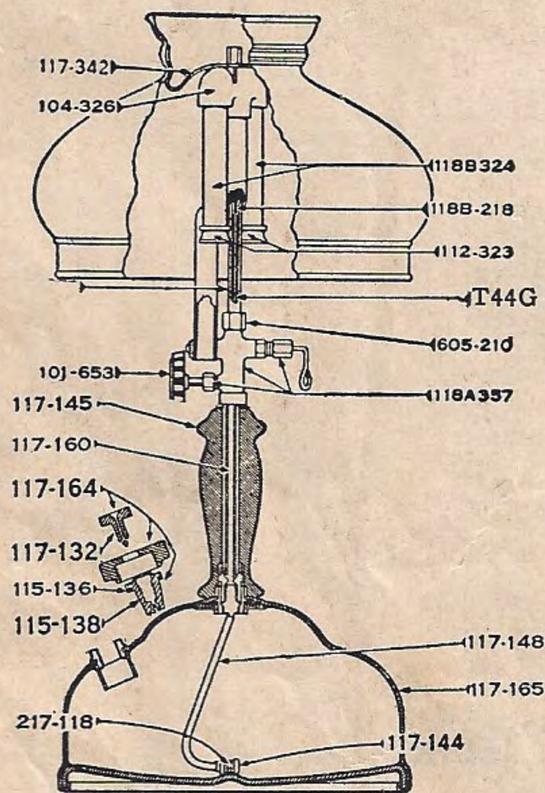
Instant-Lite Lamp No. 117A
