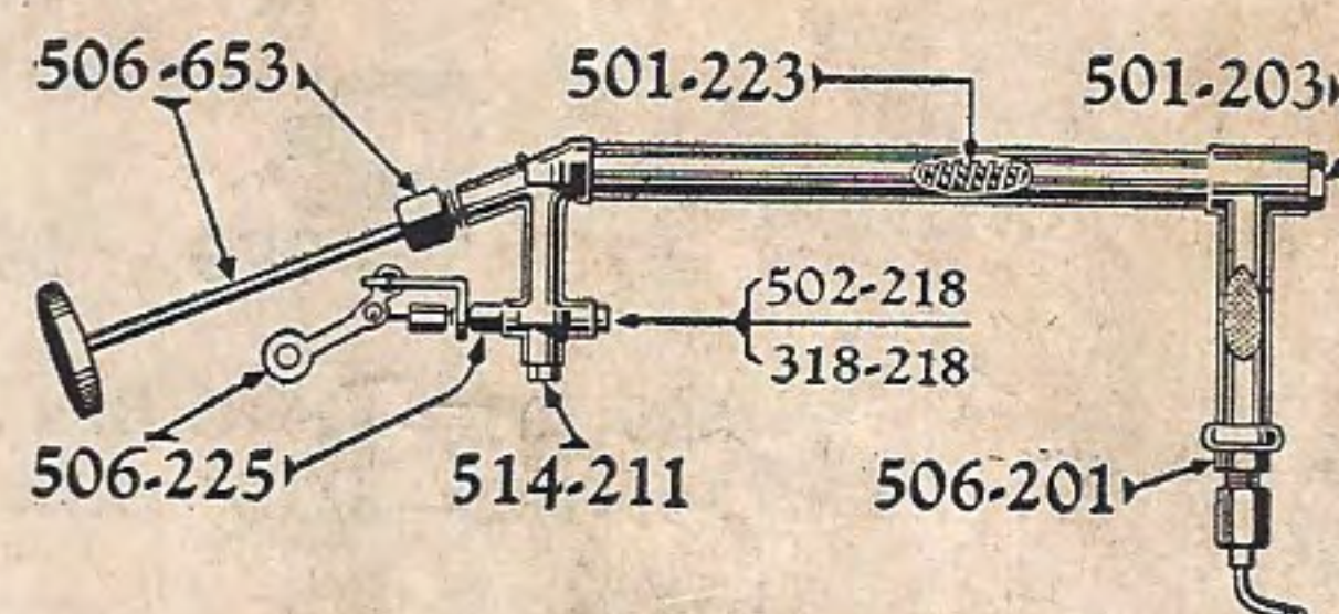
Generator No. 506-262
