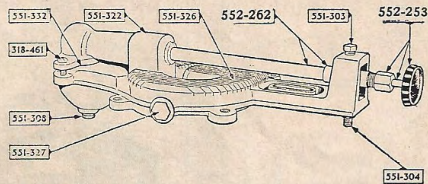
Burner Parts
