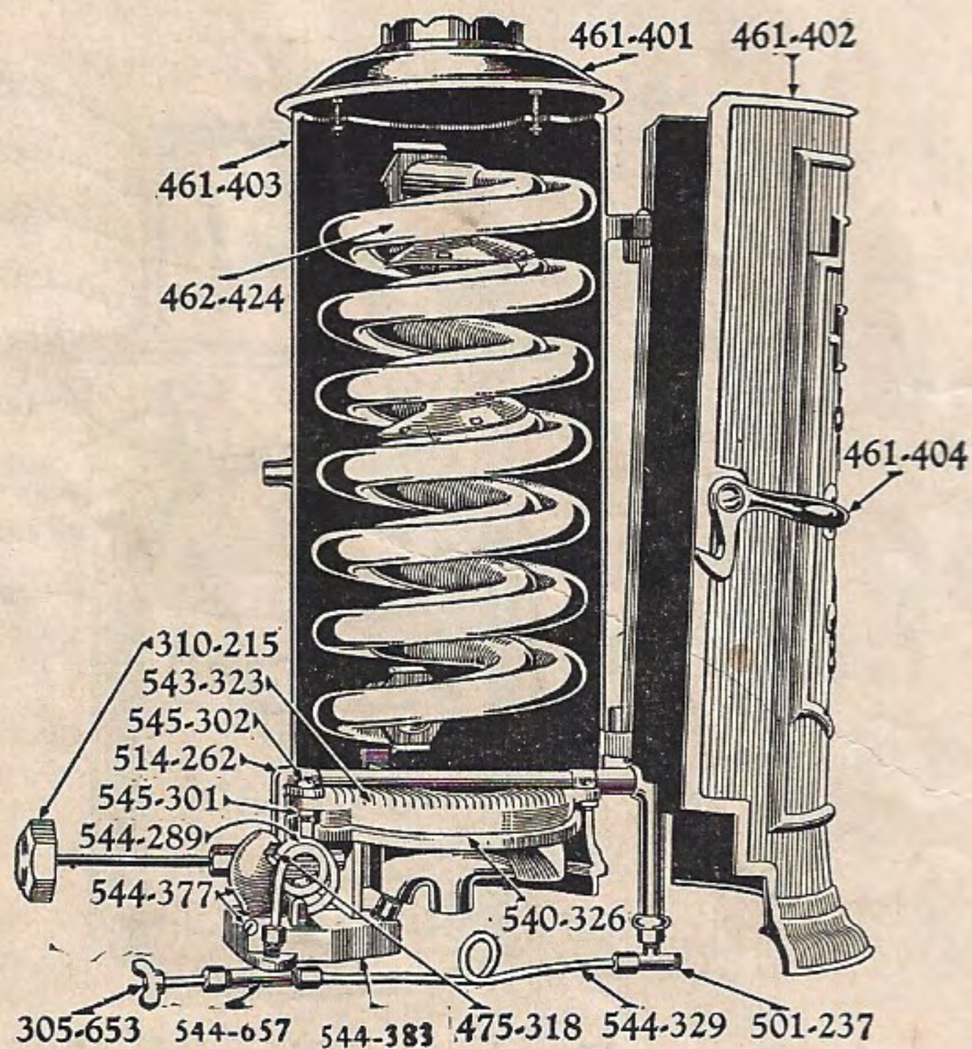
Water Heater No. 1 (With 2 Coils) (Match-Generating)
