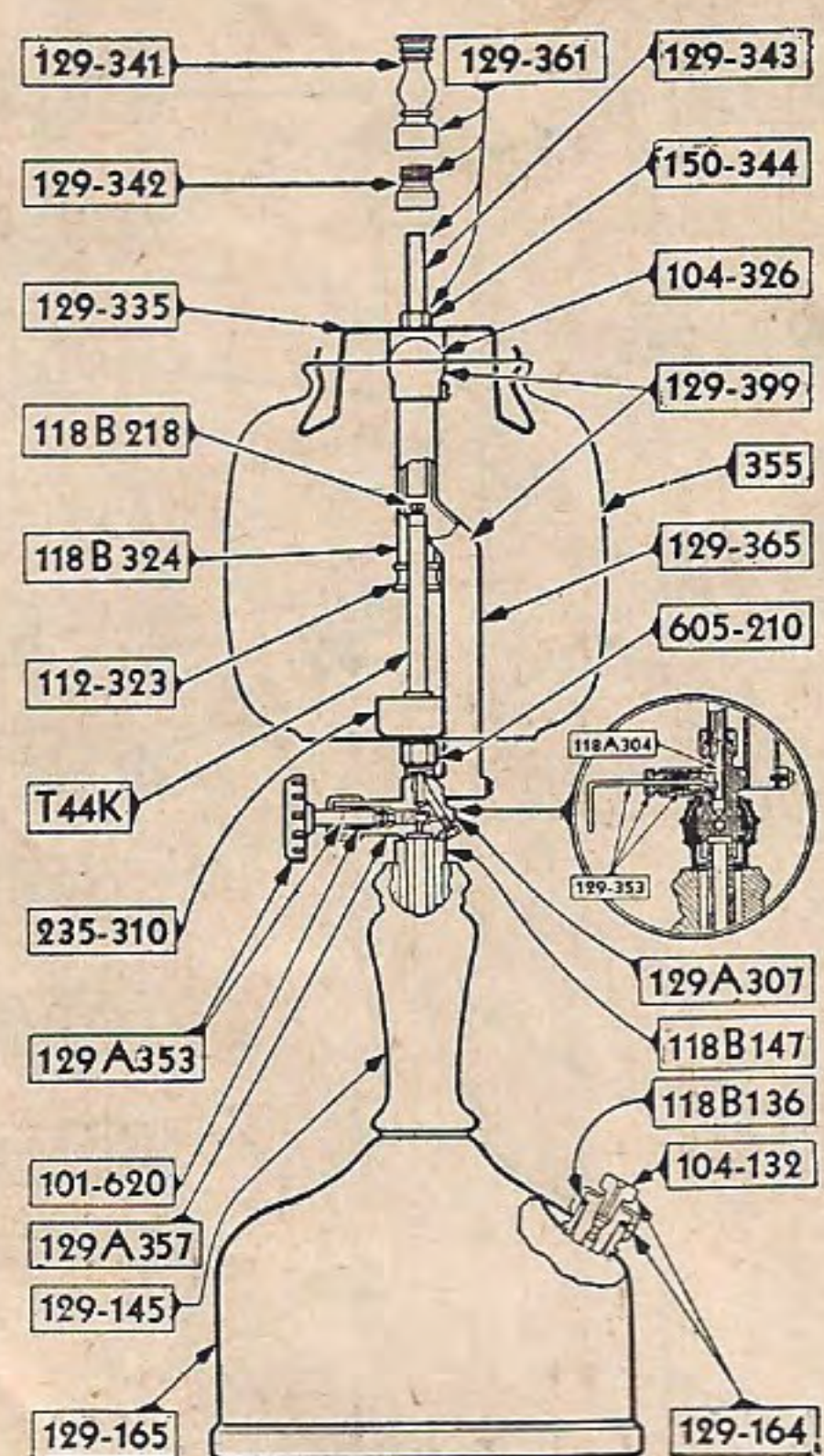
Kerosene Mantle Lamp Alcohol Generating Lamp No. 129
