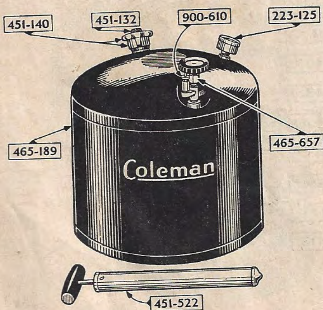
Tank, Pump and Wire No. 465-199
