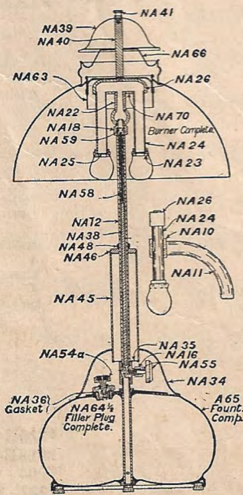
Torch-Lighting Air-O-Lite Model "A"
