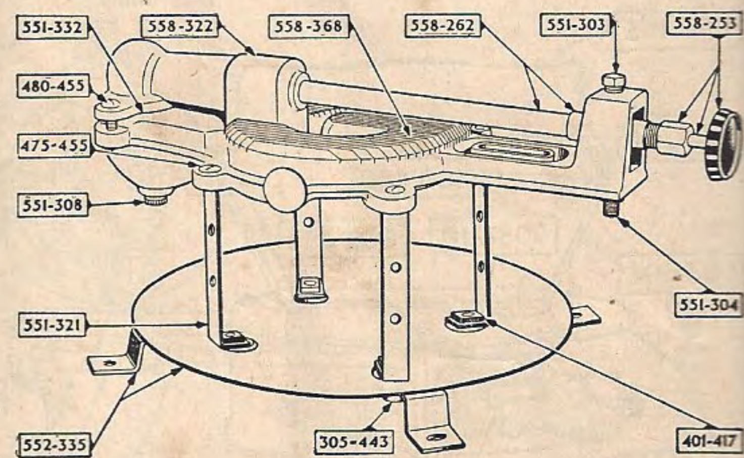
Burner No. 558
