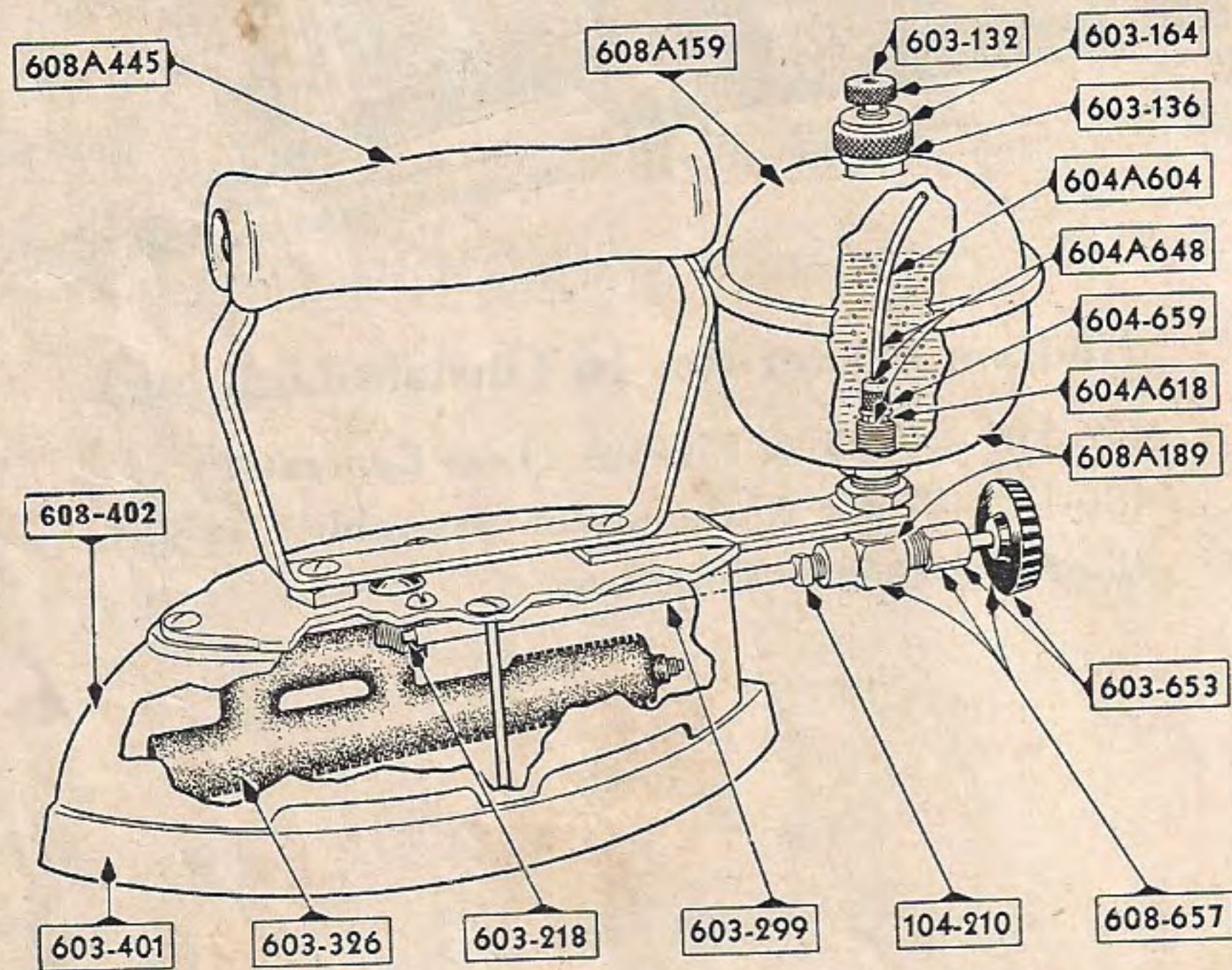
Iron No. 8A (Instant-Lighting)
