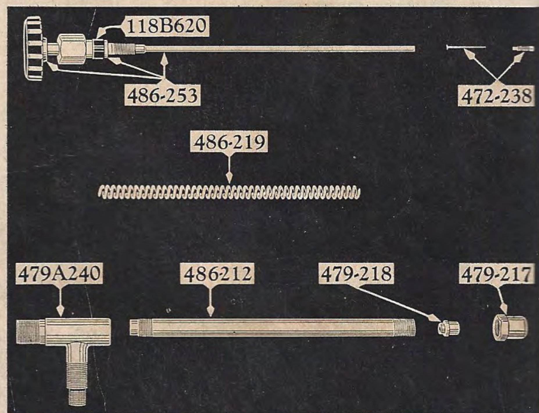
Generator 486-262
