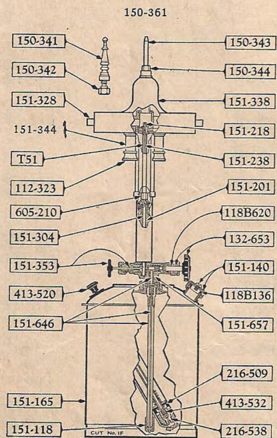
3-Mantle DeLuxe Instant-Lighting Lamp Nos. 151B and 151G
