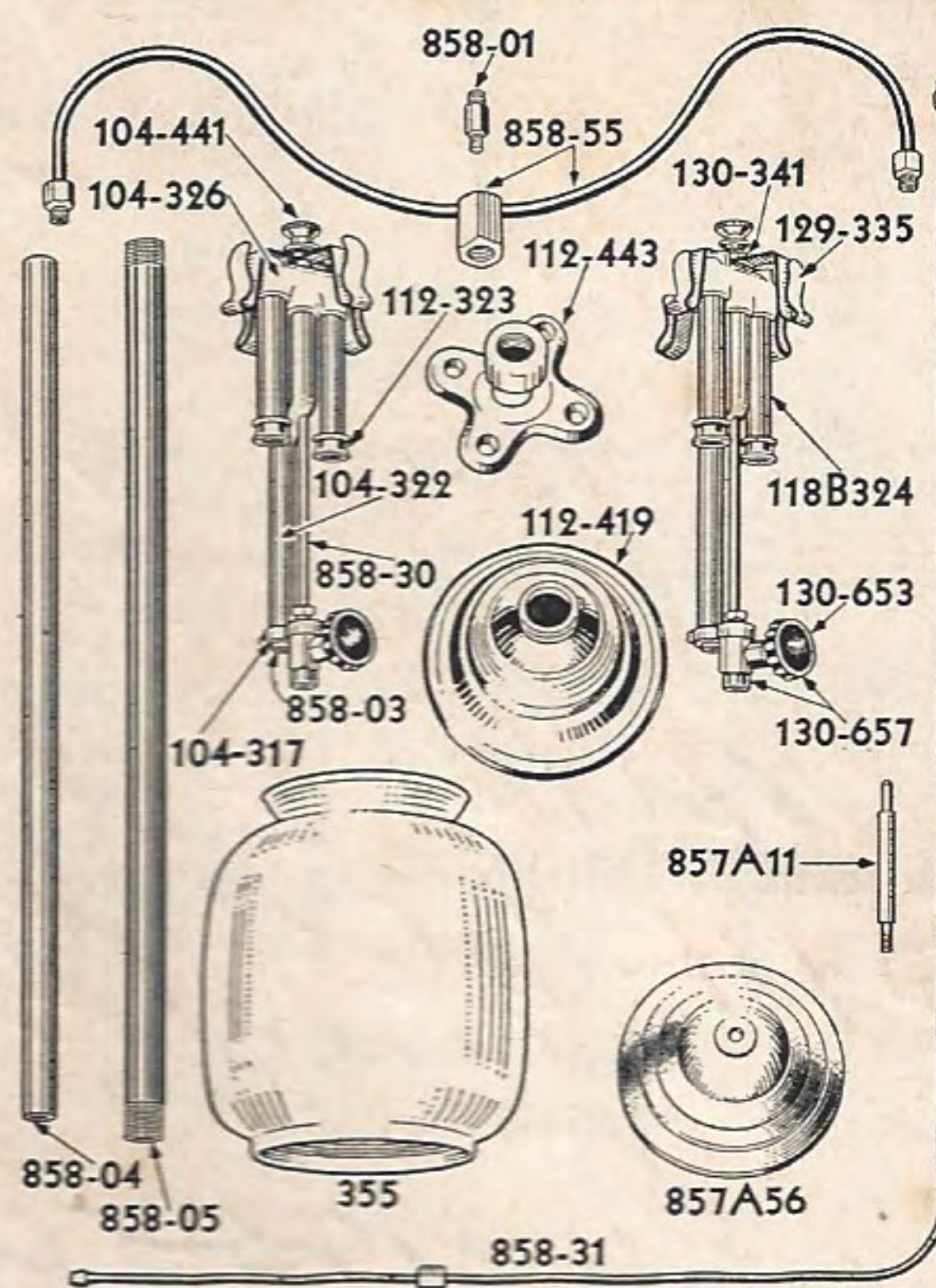
No. 858 Double Drop Fixture
