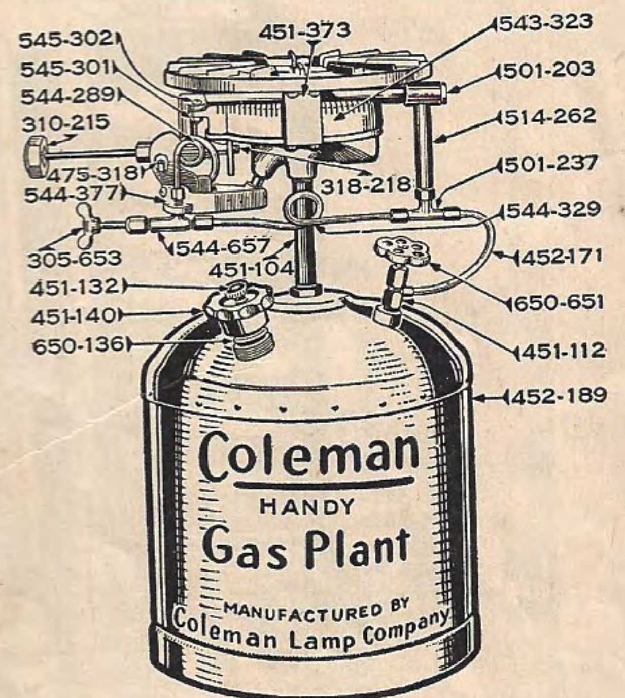
Handy Gas Plant No. 5052
