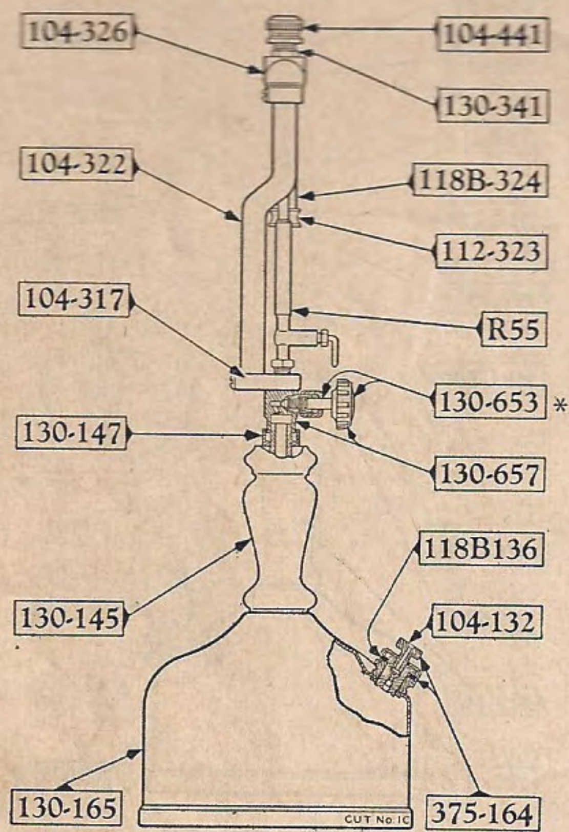
Match-Generating Lamp Nos. 130P and G
