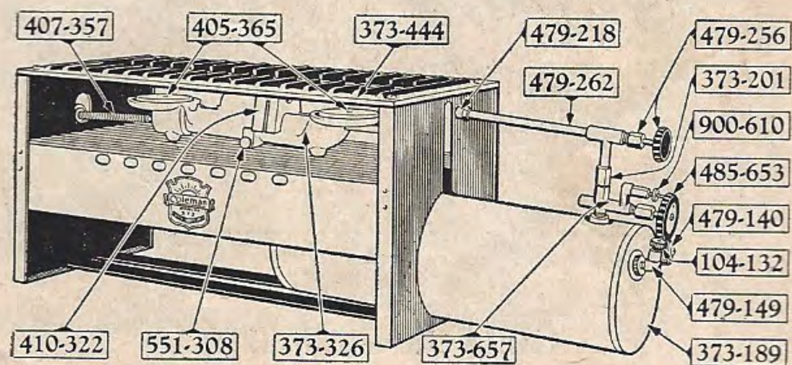
Cook Stove No. 373
