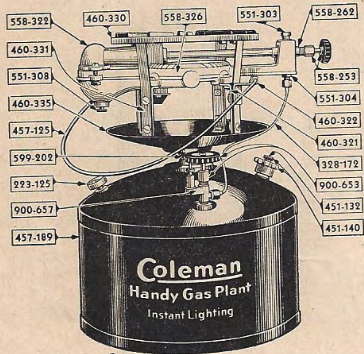
Handy Gas Plants Nos. 460 and 460G
