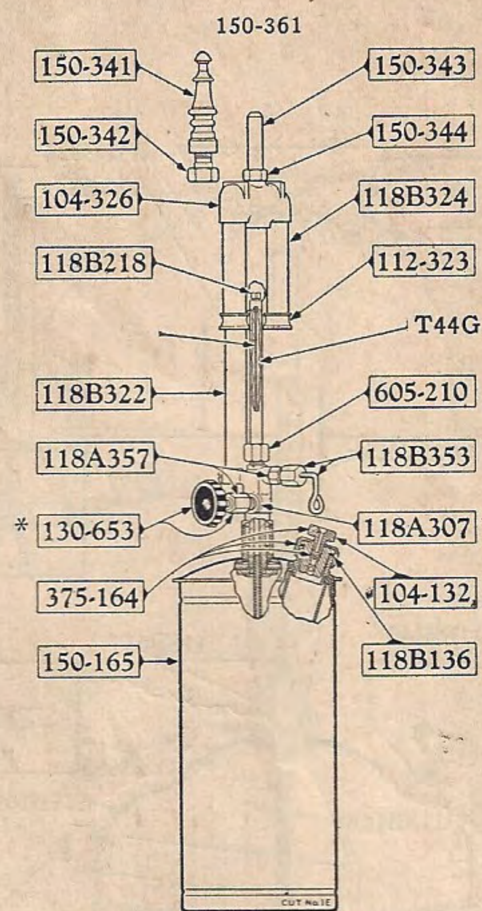
DeLuxe Match-Generating Lamp Nos. 150B, 150G, 150I, 150R
