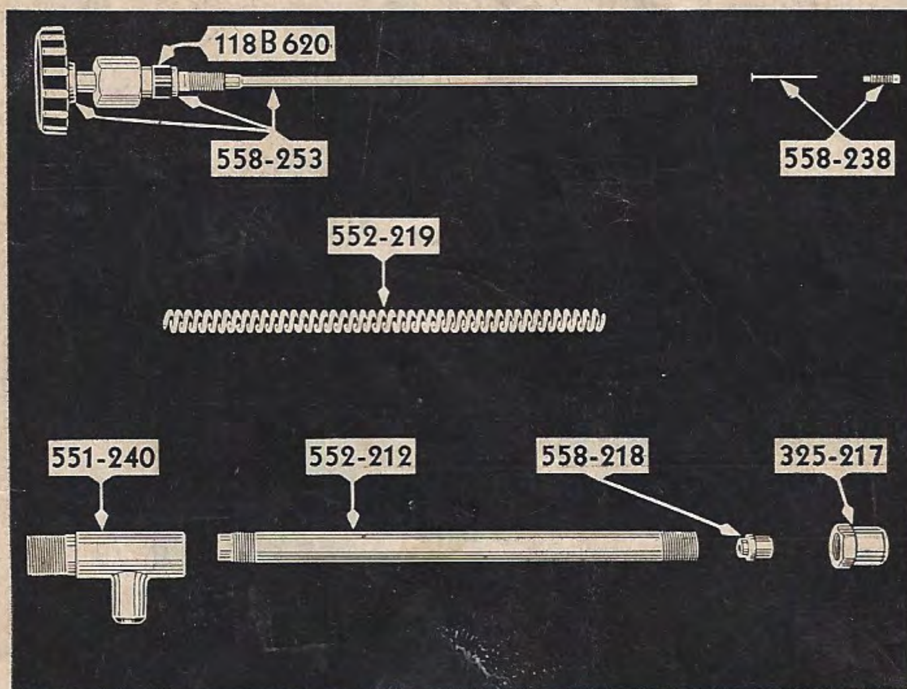
Generator No. 558-262
