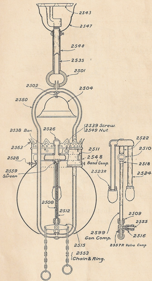
Ceiling Fixture System Lamp No. 25
