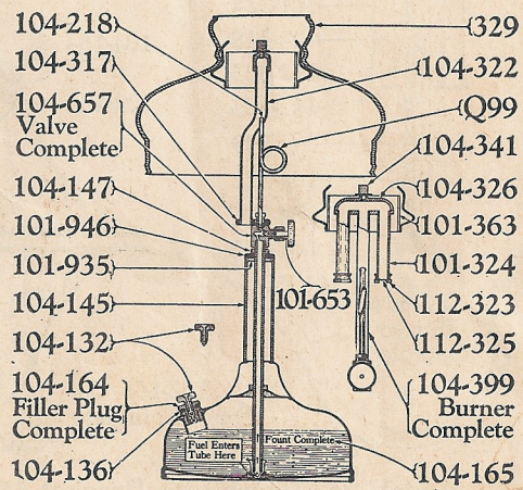
"C" Model Quick-Lite Lamp
