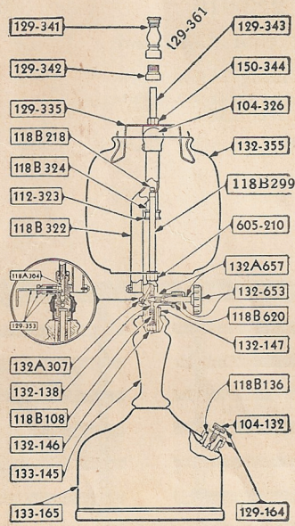
Instant Lighting Lamp No. 133
