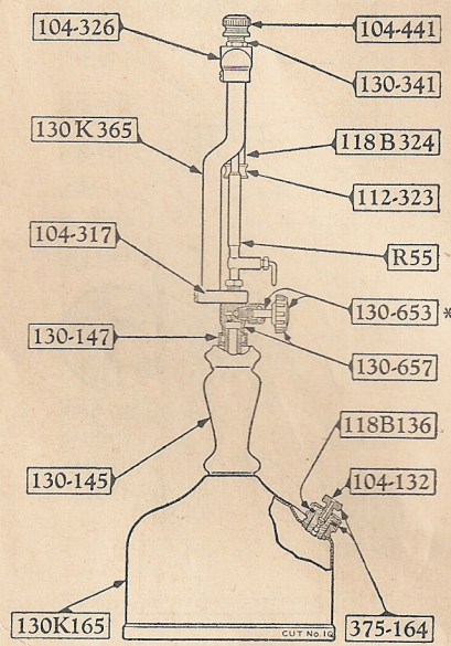
Kerosene Mantle Lamp Torch-Generating Lamp No. 130K
